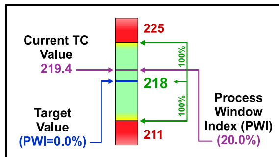
Figure 226: The Process Window Index (Single Statistic—Peak Temperature of one Thermocouple)
