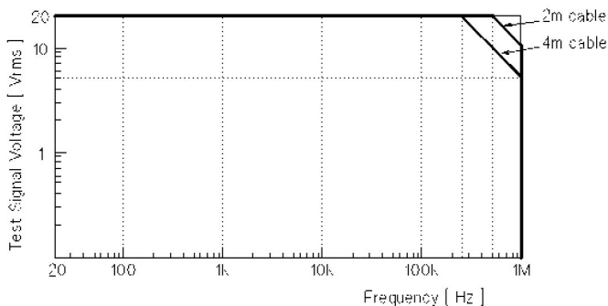
Figure 1-1. Test Signal Voltage and Test Frequency Upper Limits to Apply Measurement Accuracy to 2 m and 4 m Cable Length Operation
