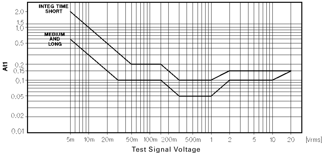
Figure 1-4. Basic Accuracy A (2 of 2)
