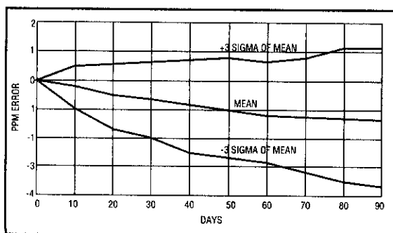
Figure 1. This plot shows stability with time of the reference voltage standard used in the HP 3458A Multimeter.
