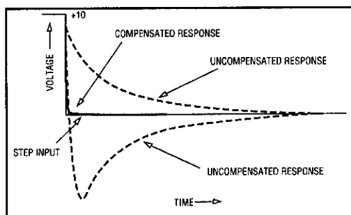
Figure 5. The frequency response of the AC attenuator is adjusted based on two readings taken at specific delays after application of a step input. Shown in this drawing are two different uncompensated responses representing undershoot and overshoot.
