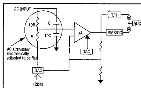
Figure 4. The AC input paths are first adjusted for flatness. Later, in the normal calibration process, gain adjustments are made.
