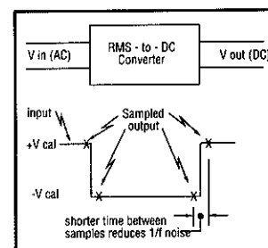
Figure 6. Positive and negative signals are internally provided to eliminate turnover errors. This input is also sampled at a higher rate to reject 1/f noise.
