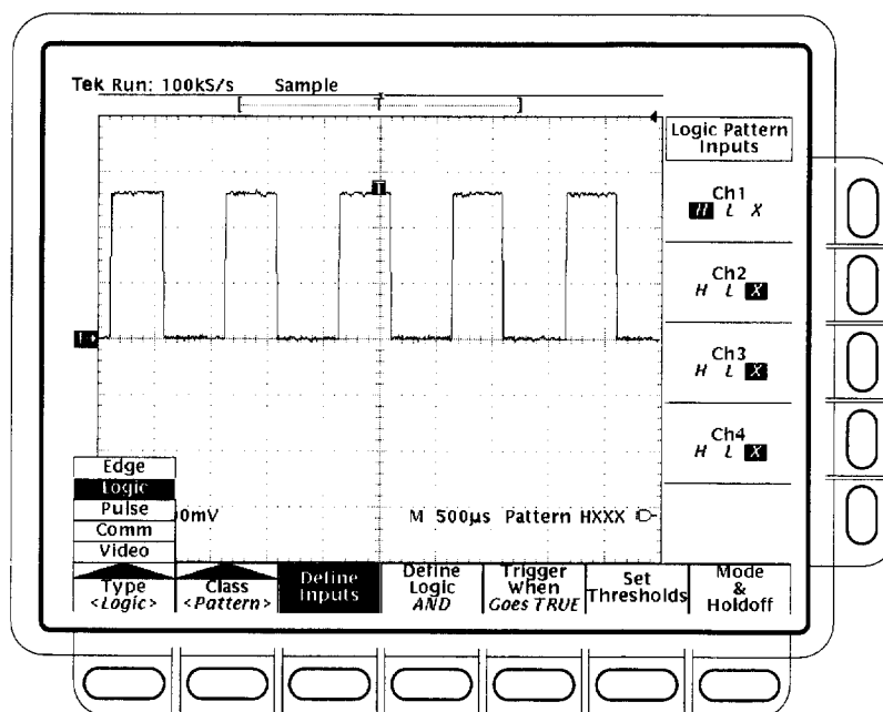
Figure 3-46: Logic Trigger Menu
