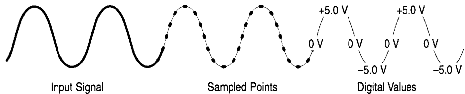
Figure 3–11: Acquisition: Input Analog Signal, Sample, and Digitize
