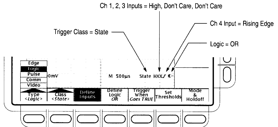
Figure 3-45: Logic Trigger Readouts — State Class Selected
