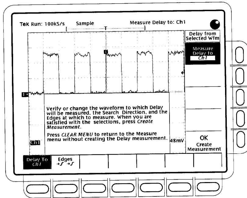
Figure 3-63: Measure Delay Menu — Delay To
