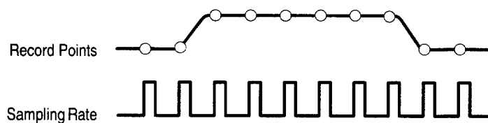
Figure 3–13: Real-Time Sampling
