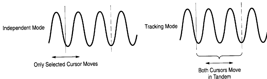
Figure 3-66: Cursor Modes
