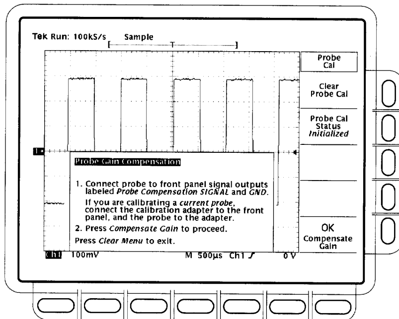
Figure 3–73: Probe Cal Menu and Gain Compensation Display
