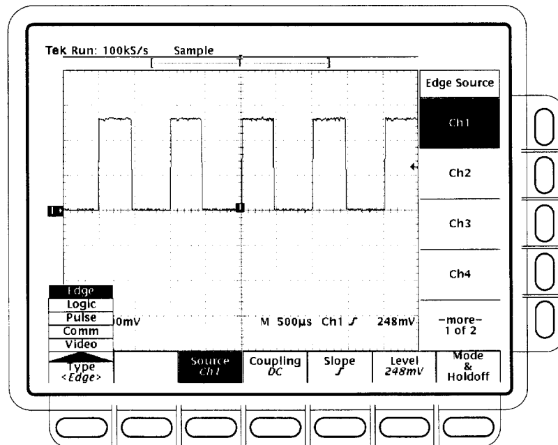
Figure 3-43: Main Trigger Menu — Edge Type
