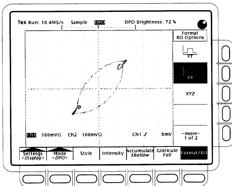
Figure 3–31: DPO XY Display
