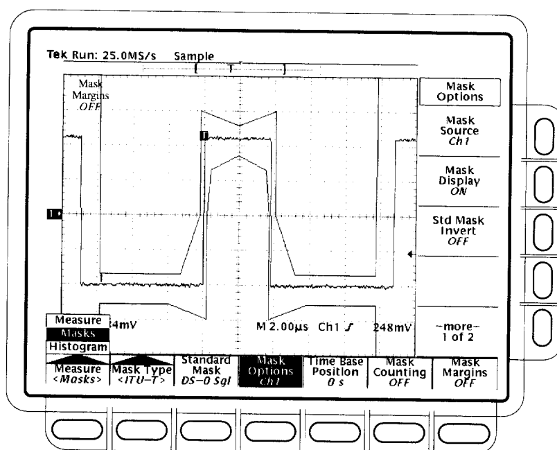
Figure 3-70: Mask menu
