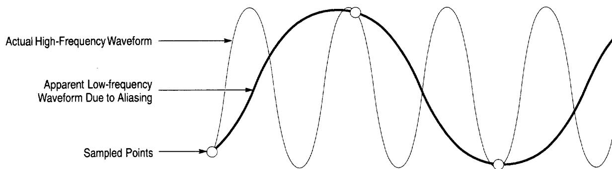
Figure 3–18: Aliasing
