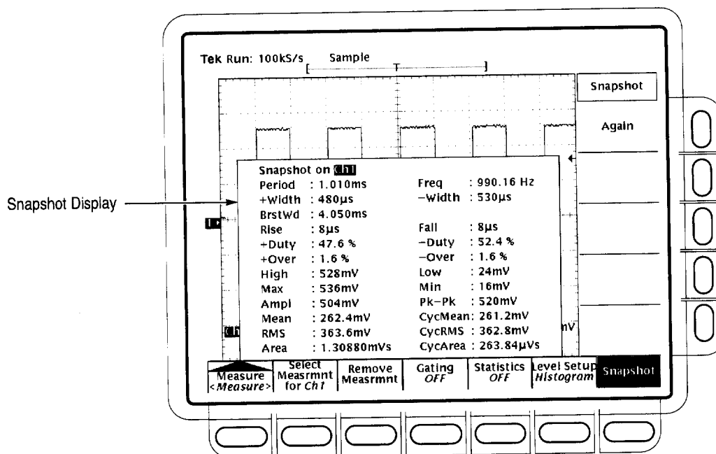
Figure 3-64: Snapshot Menu and Readout
