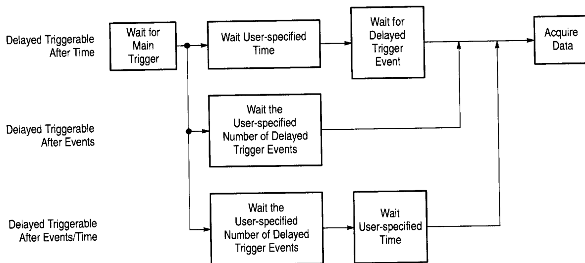
Figure 3–55: Delayed Triggerable
