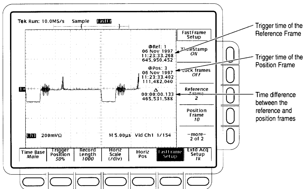
Figure 3-35: FastFrame TimeStamp
