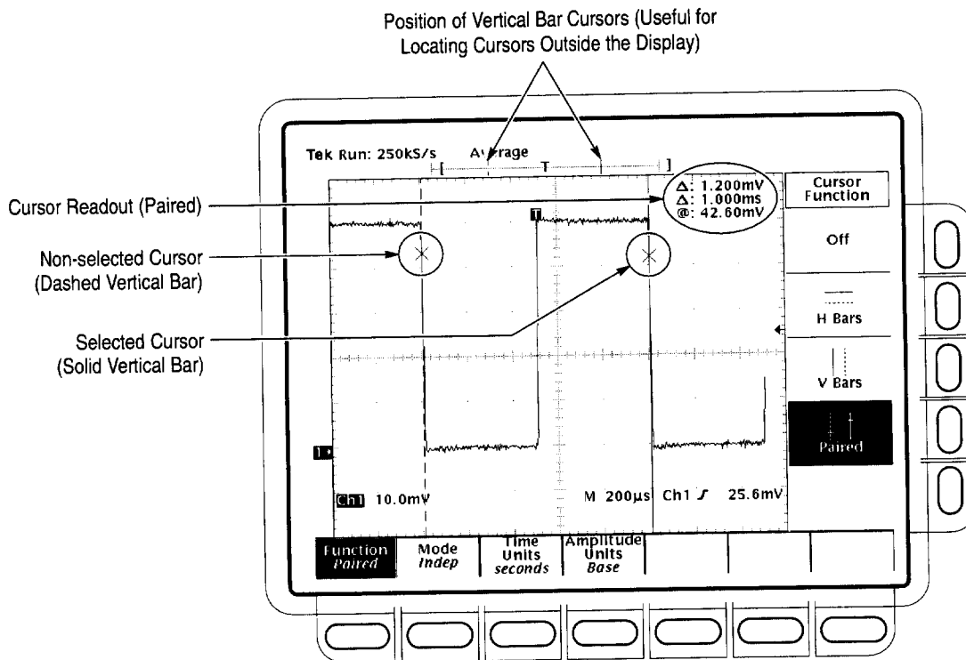
Figure 3-68: Paired Cursor Menu and Readouts
