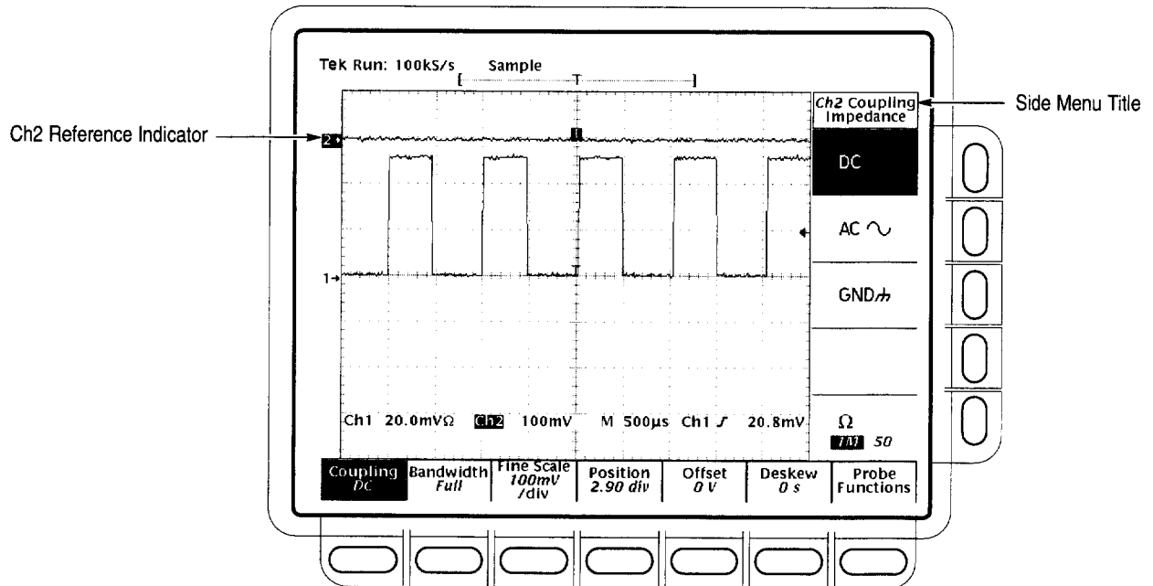
Figure 2-12: The Vertical Main Menu and Coupling Side Menu
