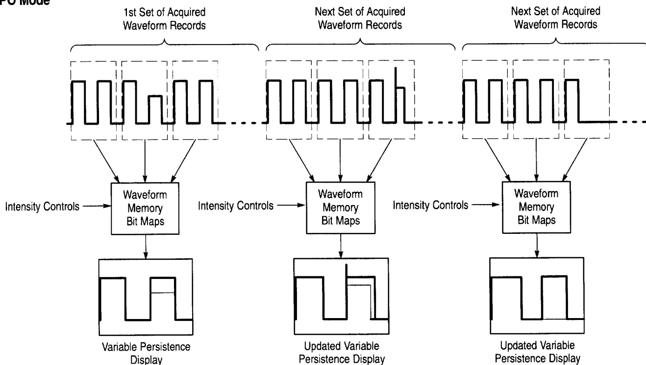
Figure 3–28: Normal DSO Acquisition and Display Mode Versus DPO Mode
