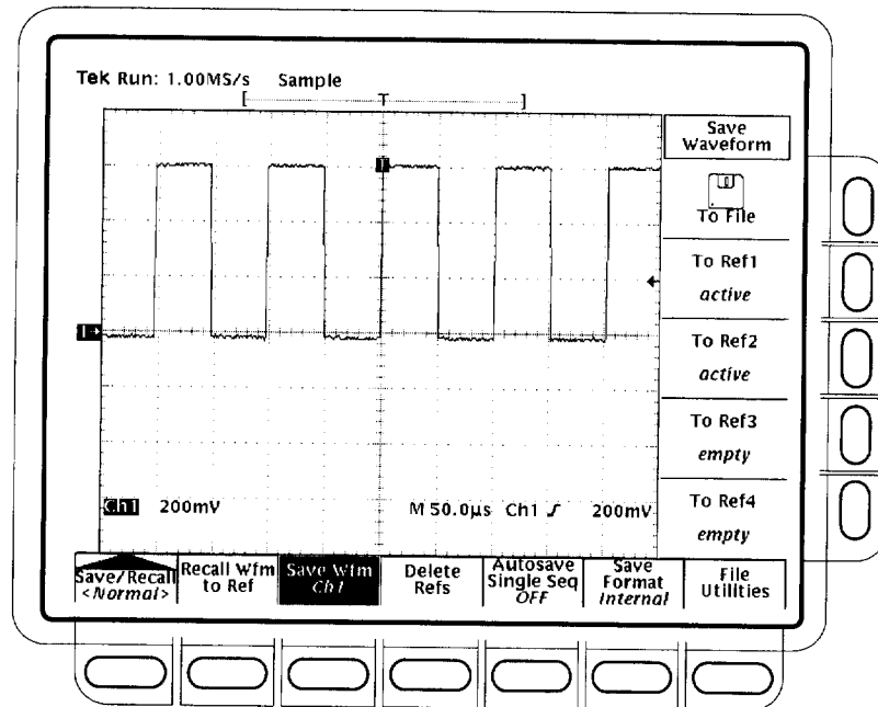
Figure 3-76: Save Waveform Menu
