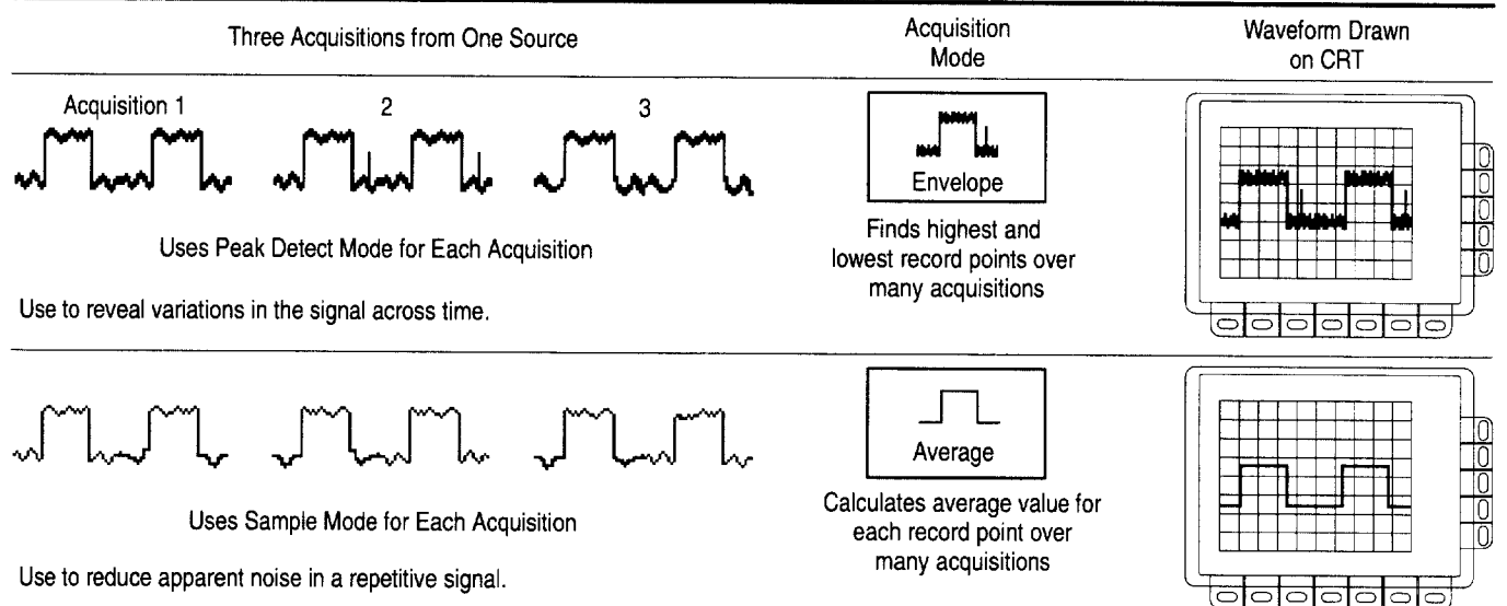
Figure 3–15: How the Acquisition Modes Work
