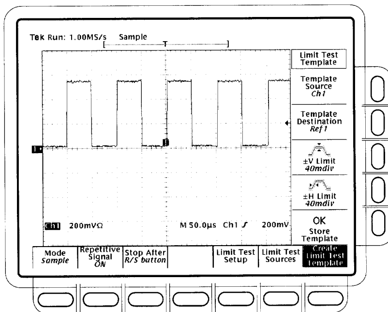
Figure 3-93: Acquire Menu — Create Limit Test Template
