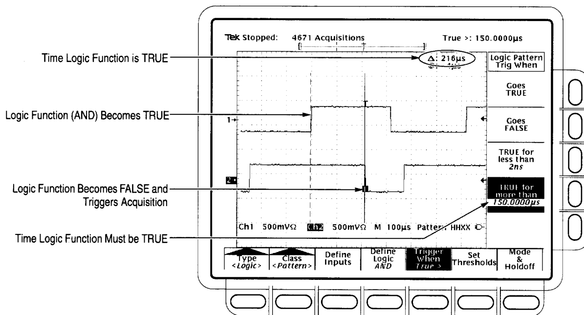
Figure 3–47: Logic Trigger Menu — Time Qualified TRUE
