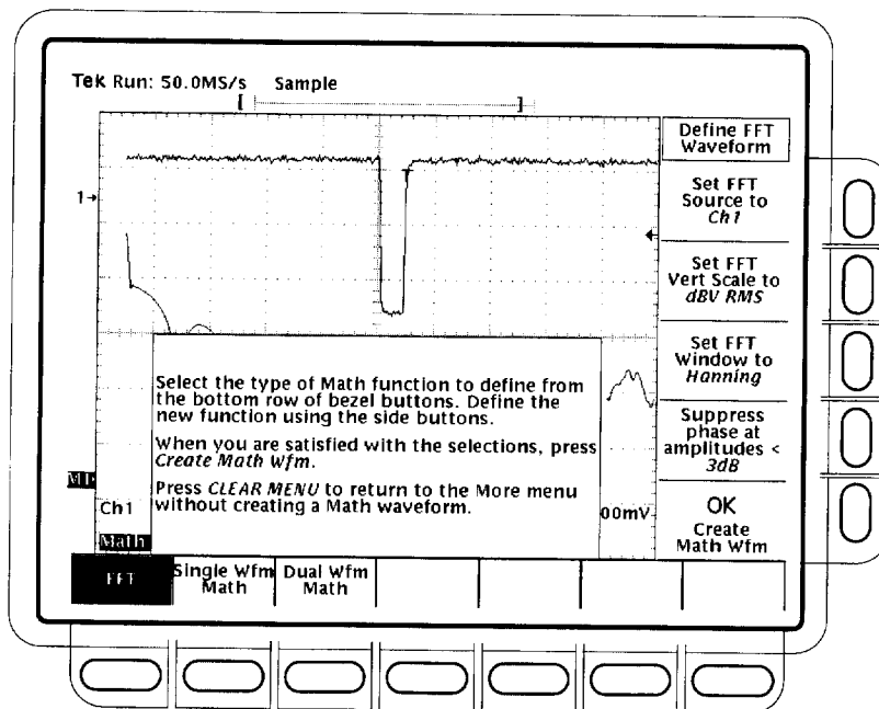
Figure 3-97: Define FFT Waveform Menu
