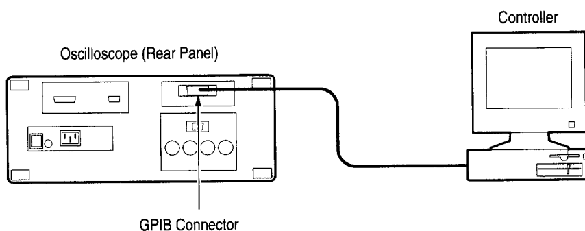
Figure 3-87: Connecting the Oscilloscope to a Controller
