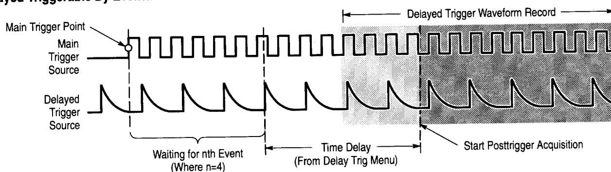
Figure 3-56: How the Delayed Triggers Work
