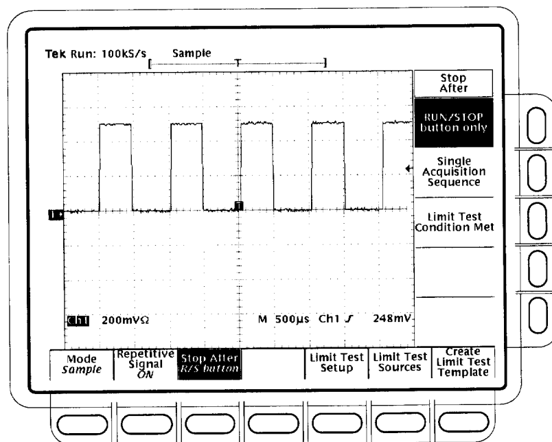
Figure 3-17: Acquire Menu — Stop After
