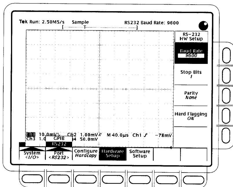
Figure 3–80: Utility Menu — System I/O
