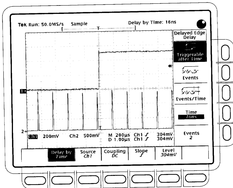
Figure 3-57: Delayed Trigger Menu
