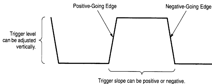
Figure 3–38: Slope and Level Controls Help Define the Trigger
