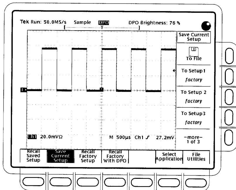
Figure 3–75: Save/Recall Setup Menu
