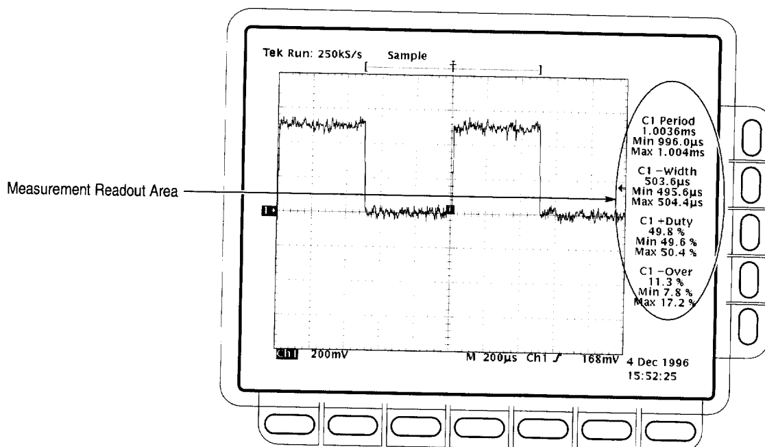
Figure 3-59: Measurement Readouts with Statistics
