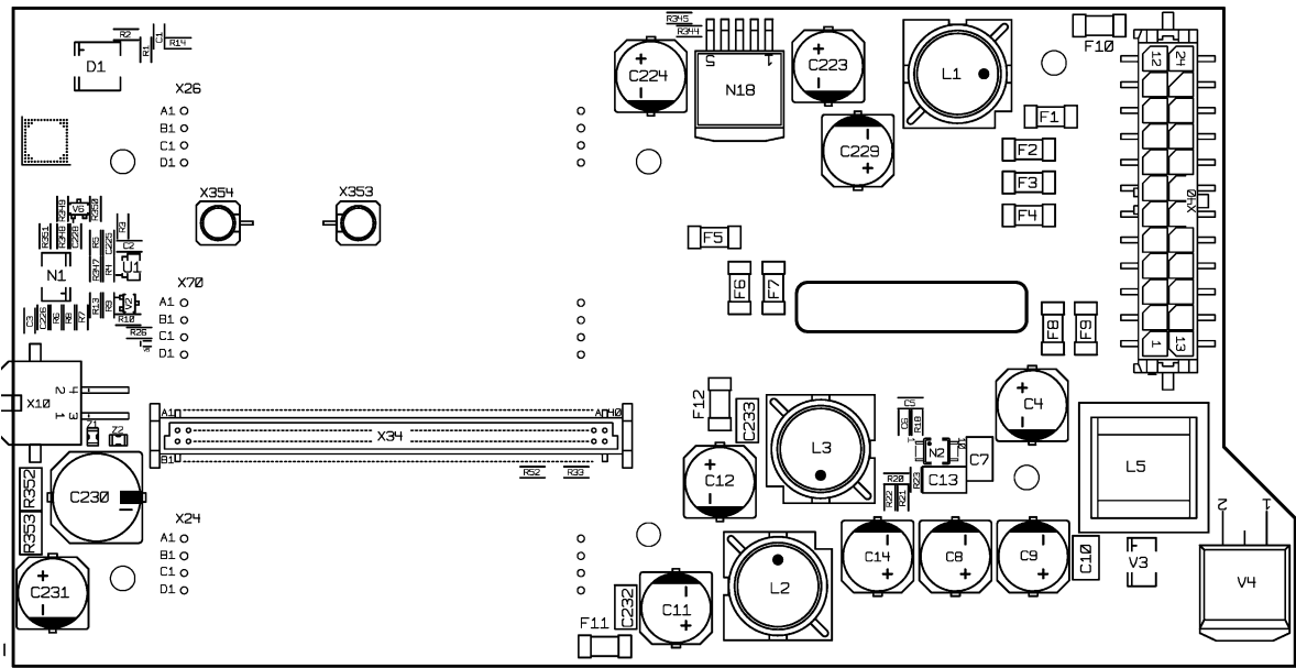
Fig. 3-2 Motherboard
