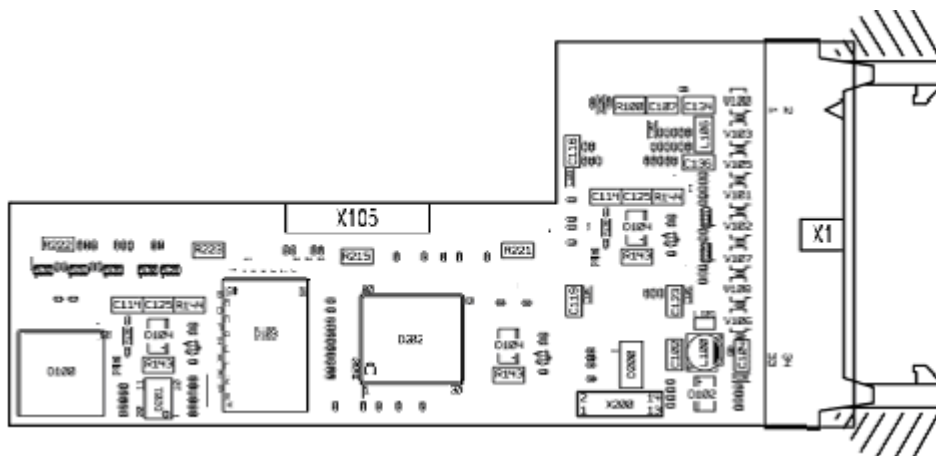
Fig. 3-5 Display Adapter Board
