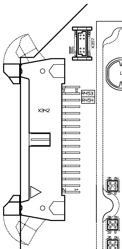
Fig. 3-7 Connection X357 to Keyboard Controller Board, X342 is not fitted for Var. 03
