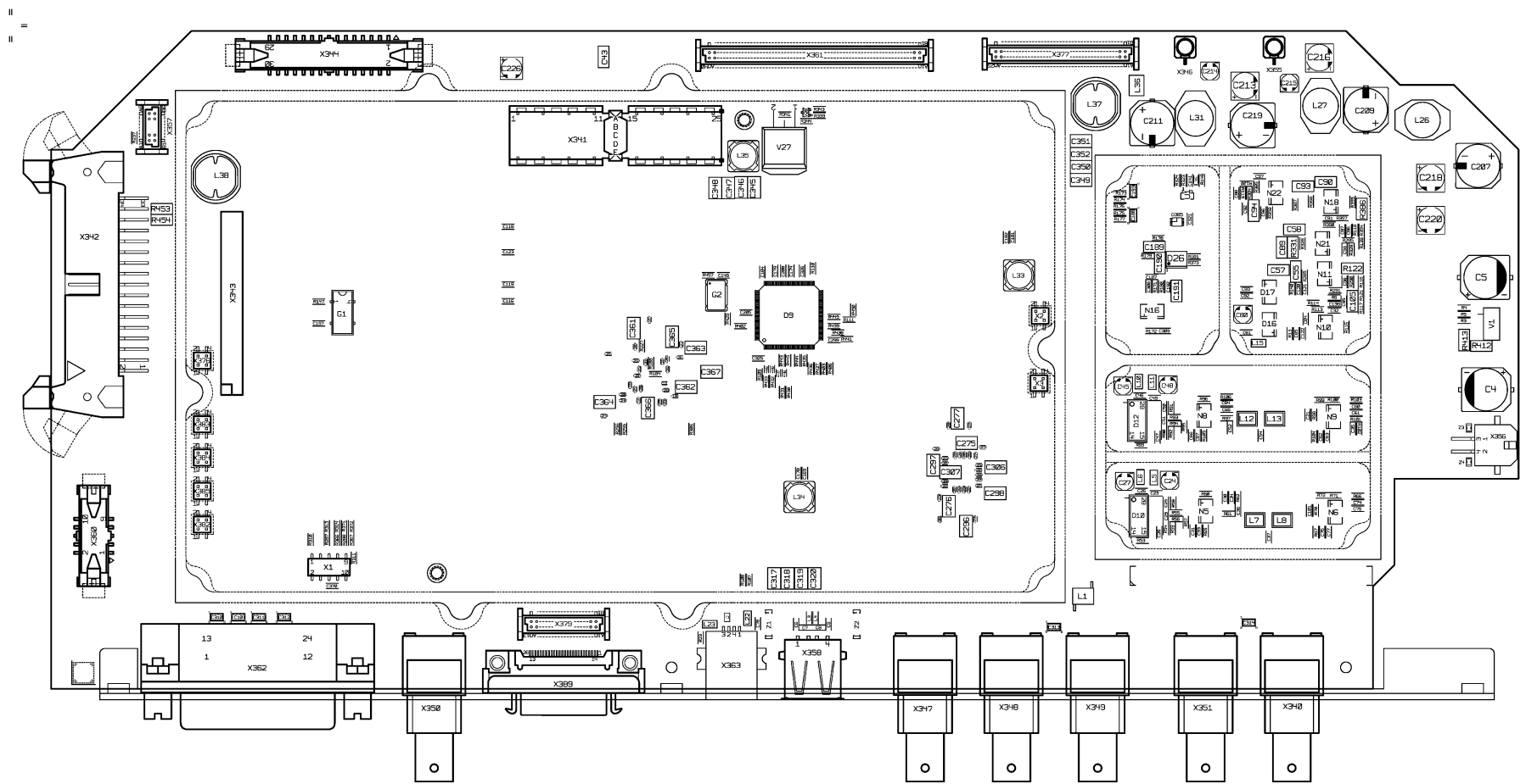
Fig. 3-3 Interface Board
