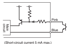
Zero shift input circuit (AP-C30K/C31K/C33K)
