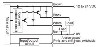
Input/output circuit (AP-C30KP/C31KP/C33KP)
