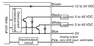
Analog output circuit
