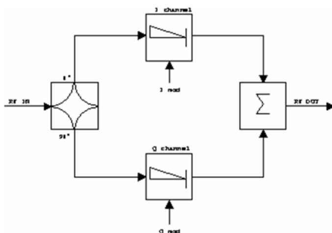
Fig. 3-34: I/Q modulation
