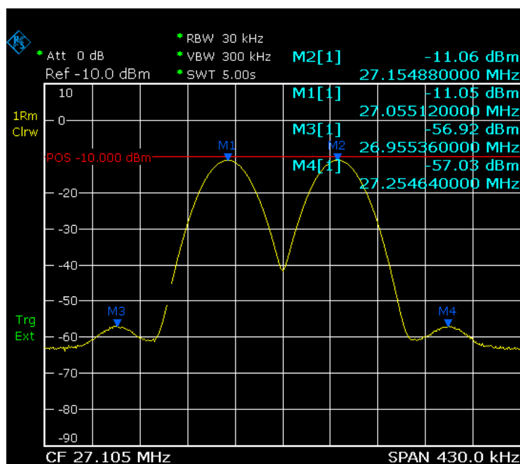
Fig. 3-10: Trace example
