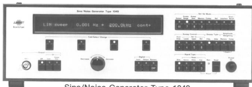
Sine/Noise Generator Type 1049
