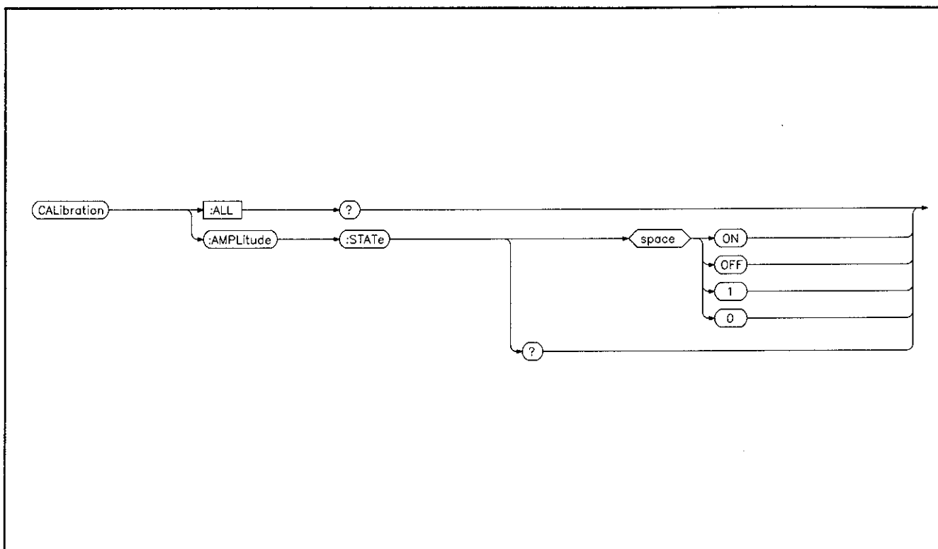
Figure 6-7. Calibration Subsystem.
