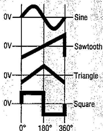
Figure 2. Relative Phase of Audio Waveforms
