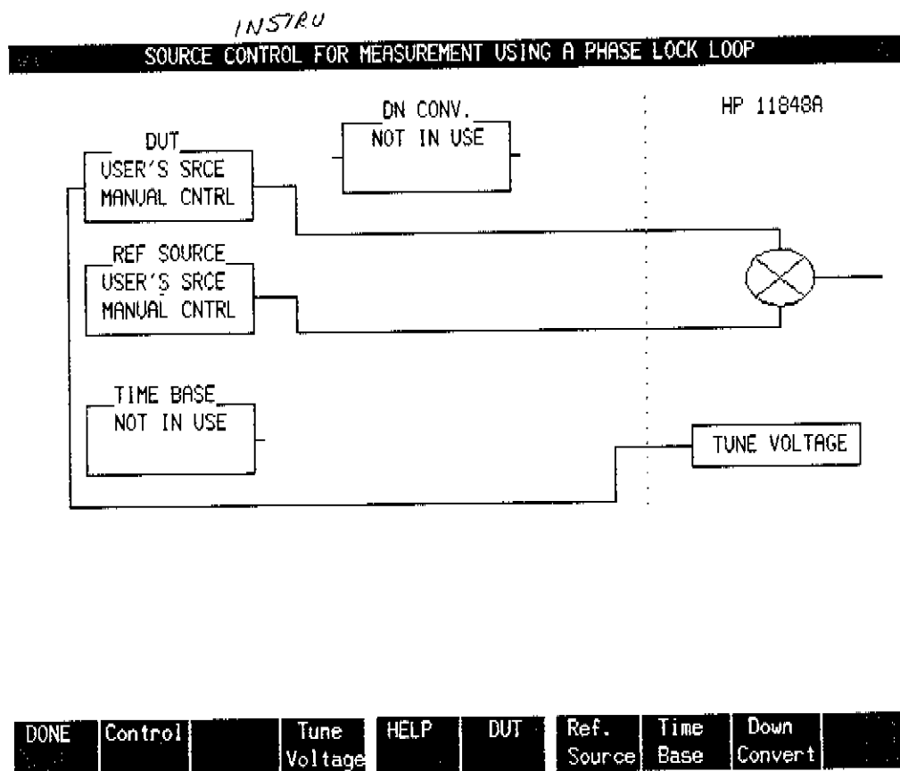
Figure 8-11. Source Control for Measurement Using a Phase Lock Loop Menu
