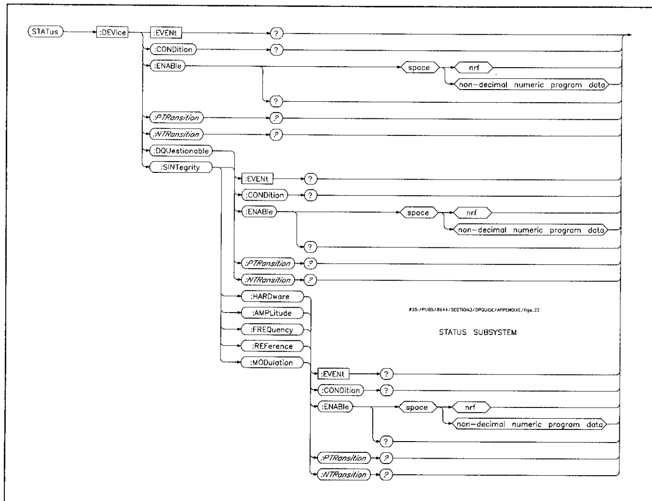
Figure 6-24. Status Subsystem.
