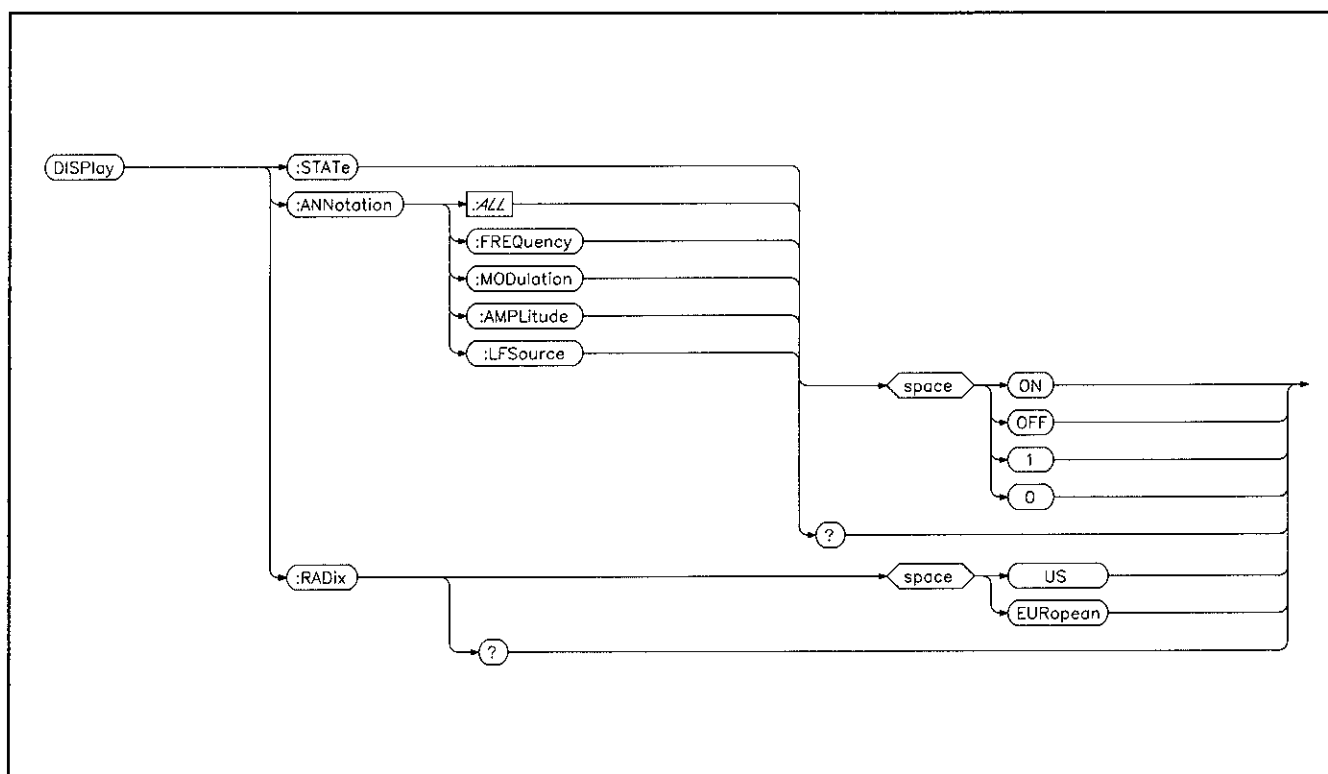
Figure 6-8. Display Subsystem.
