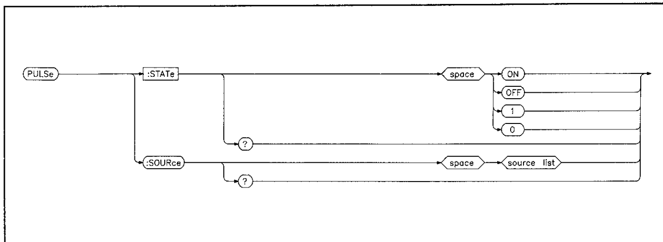
Figure 6-21. Pulse Subsystem.
