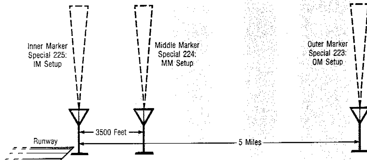
Marker Beacon Antenna Locations
