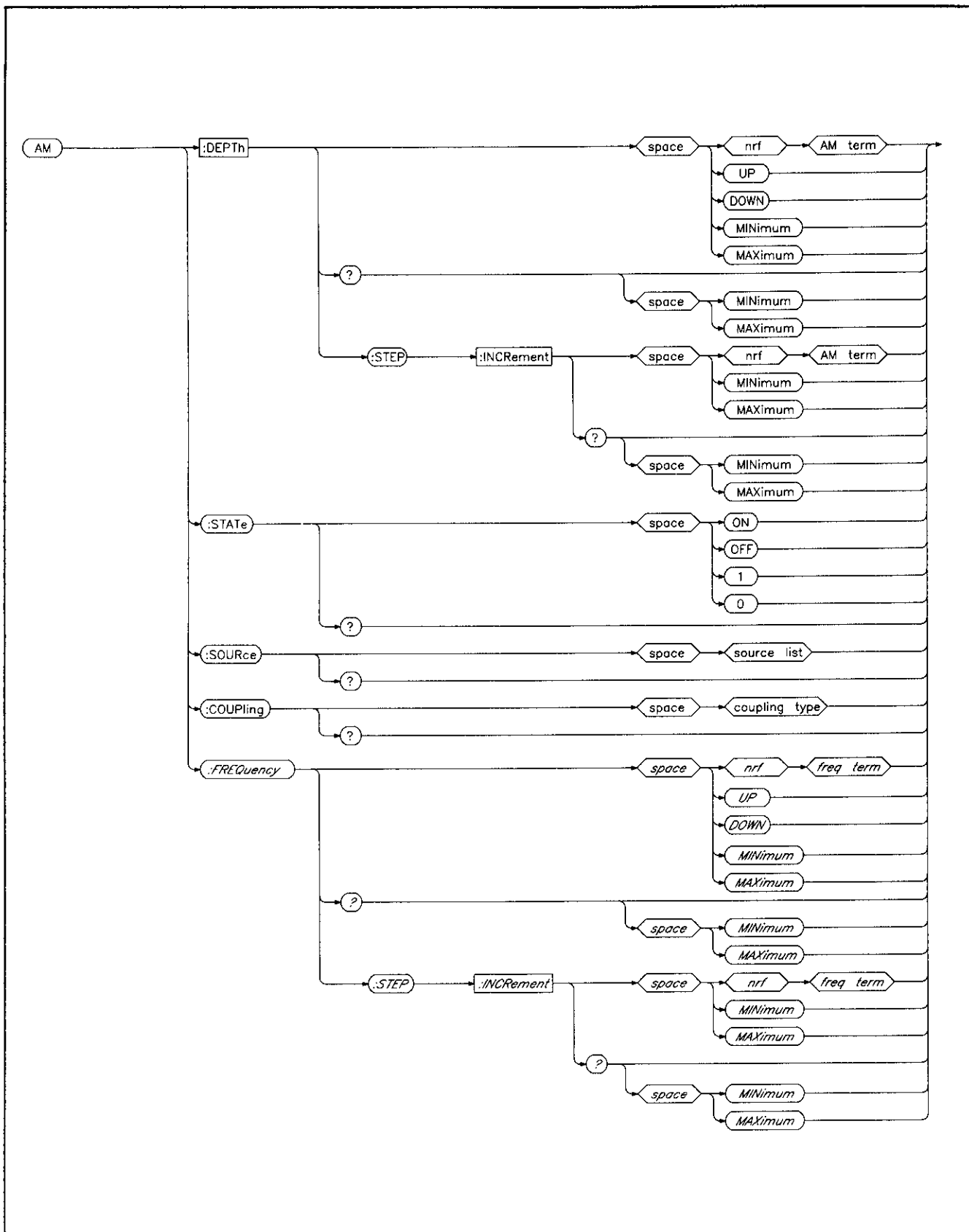
Figure 6-5. AM Subsystem.
