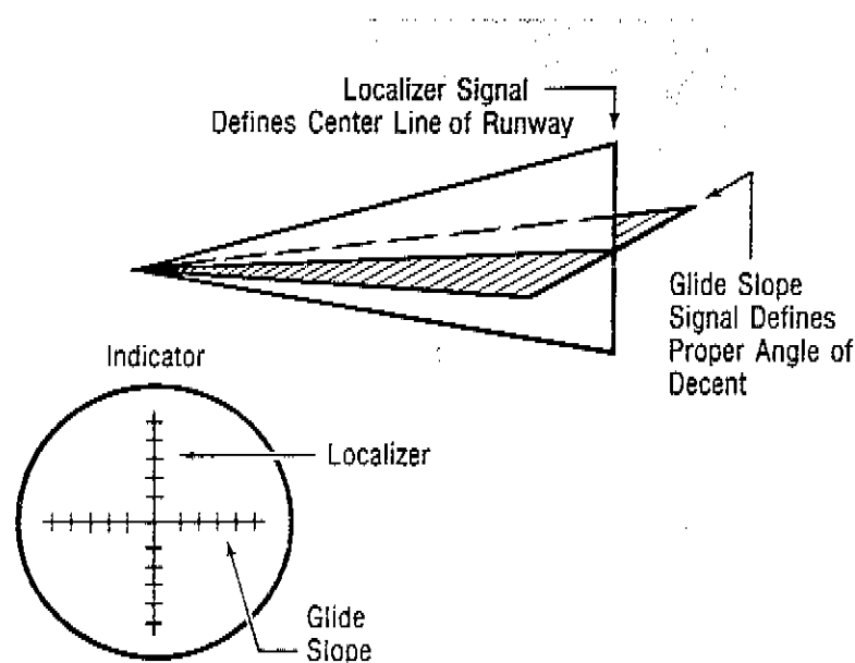
Localizer and Glide Slope Radiation Pattern and Aircraft Indicator Display
