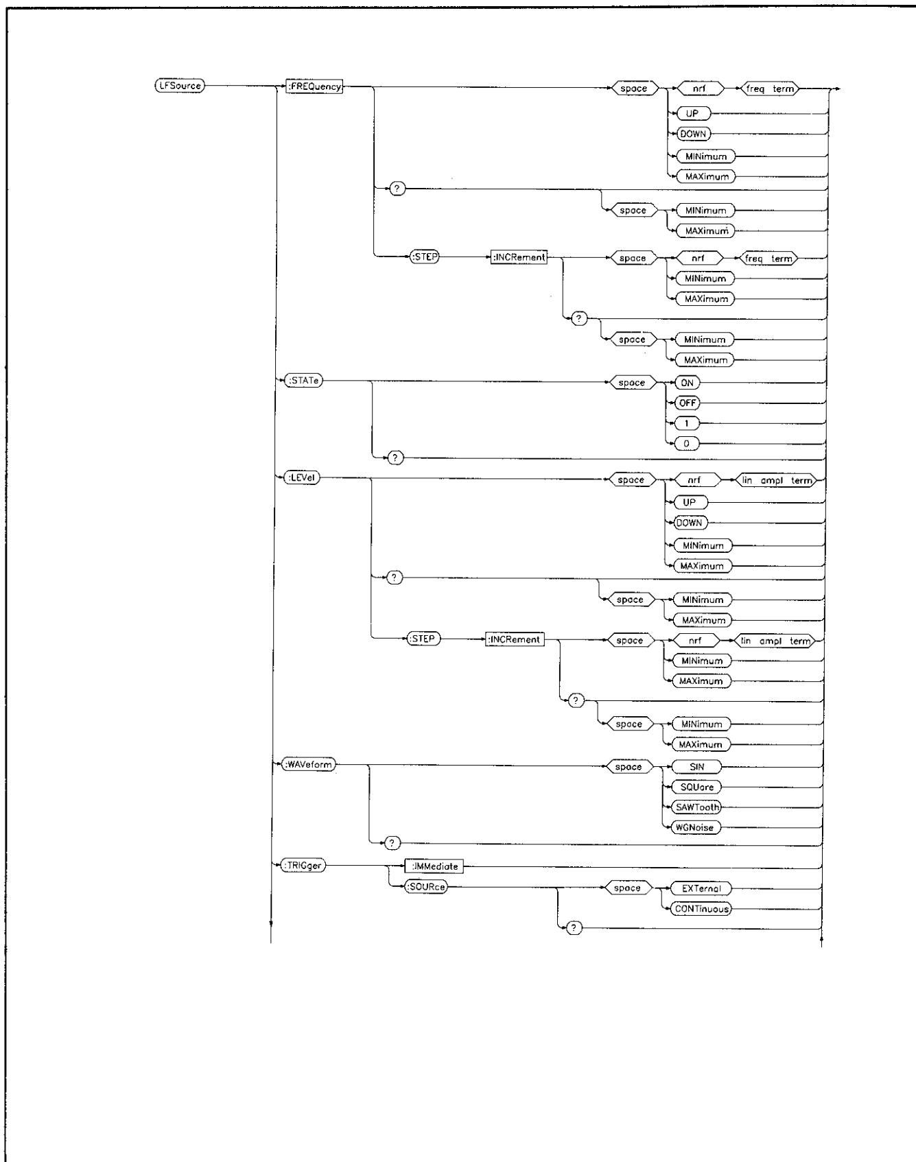
Figure 6-15. LF Source Subsystem. (1 of 6)
