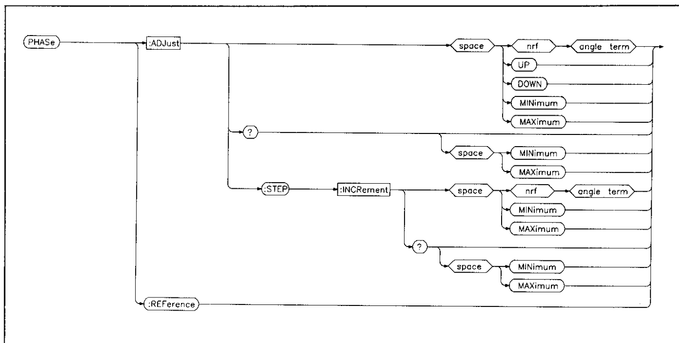
Figure 6-19. Phase Subsystem.
