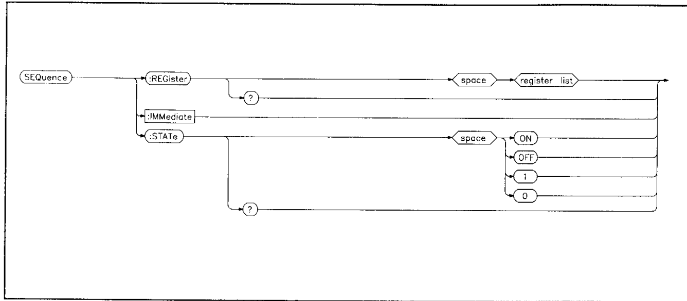
Figure 6-23. Sequence Subsystem.
