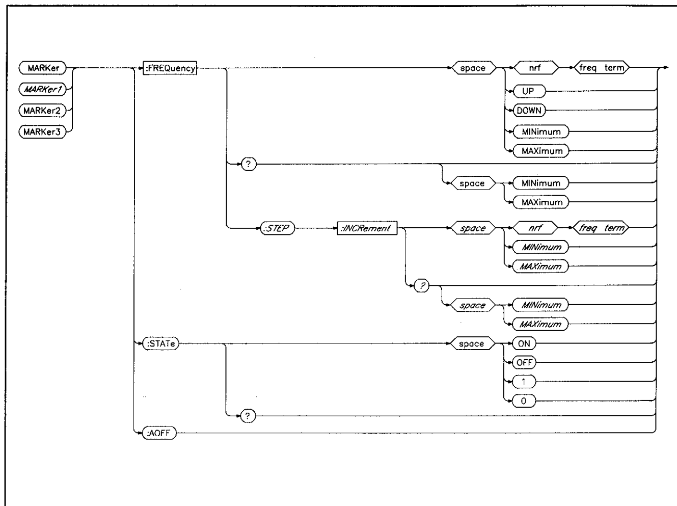
Figure 6-16. Marker Subsystem.
