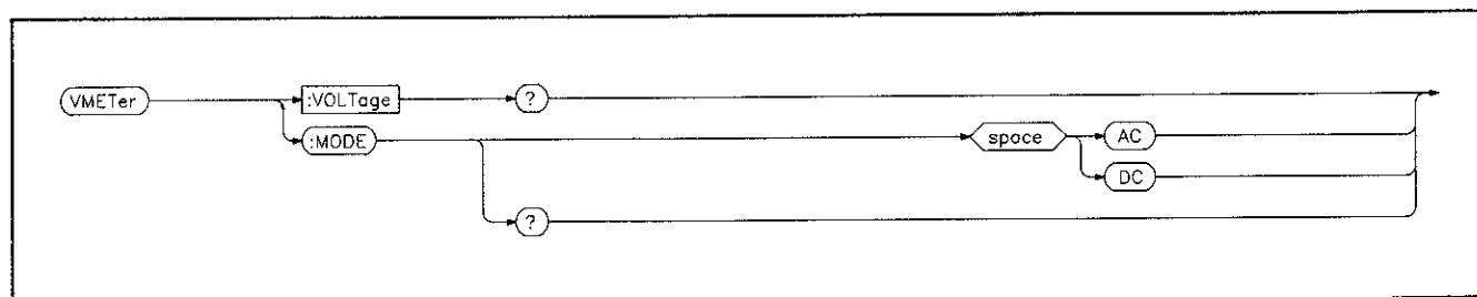
Figure 6-27. Voltmeter Subsystem.
