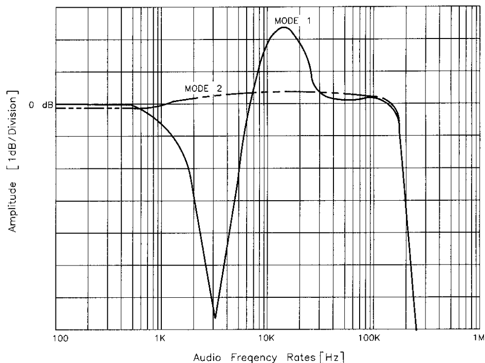
Figure 4-2. FM Indicator Accuracy with Special Function 124 Off.
