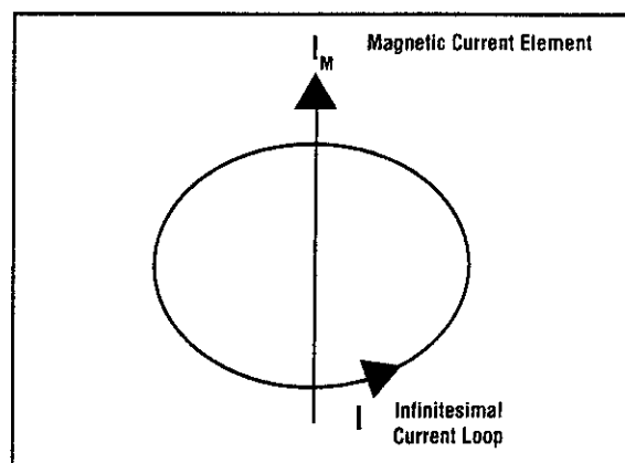
Figure 4. Magnetic current element
