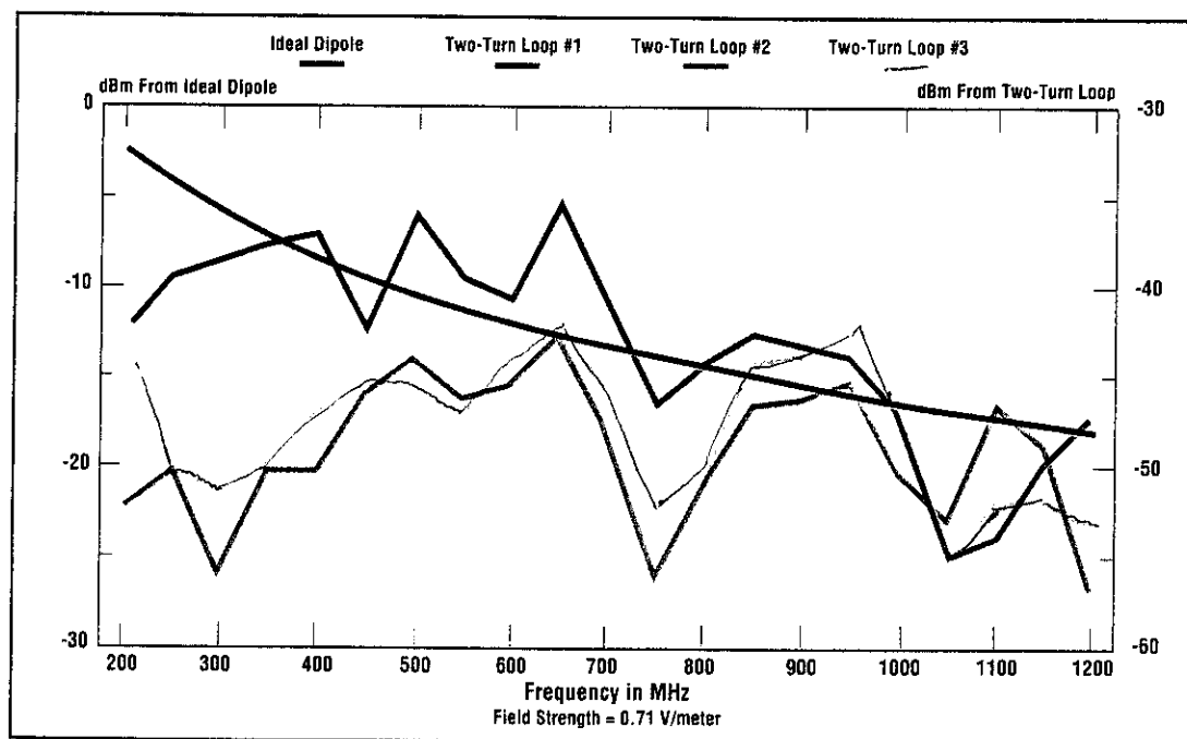
Figure 7. Two turn loop far field responses vs. ideal dipole
