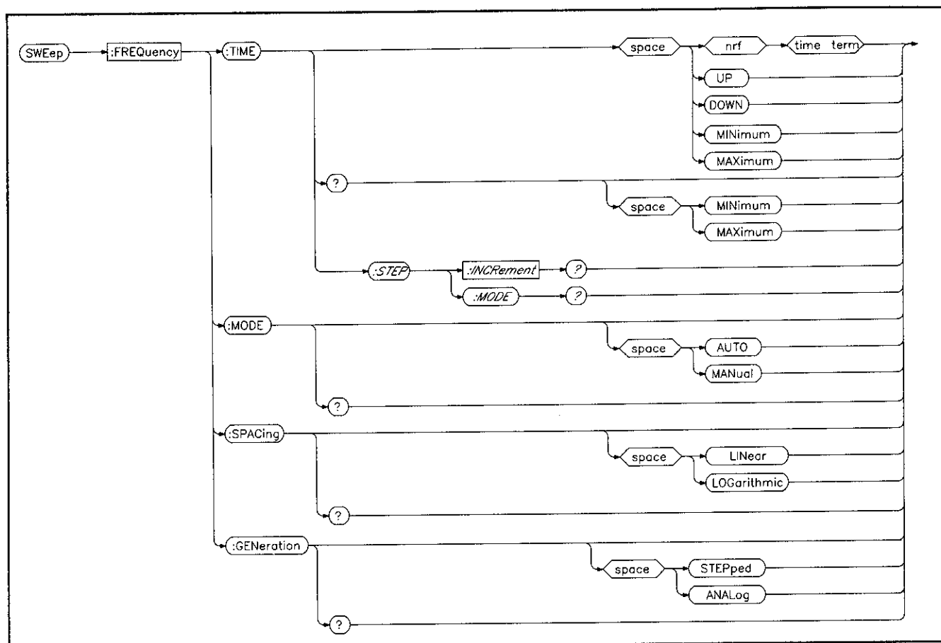
Figure 6-25. Sweep Subsystem.
