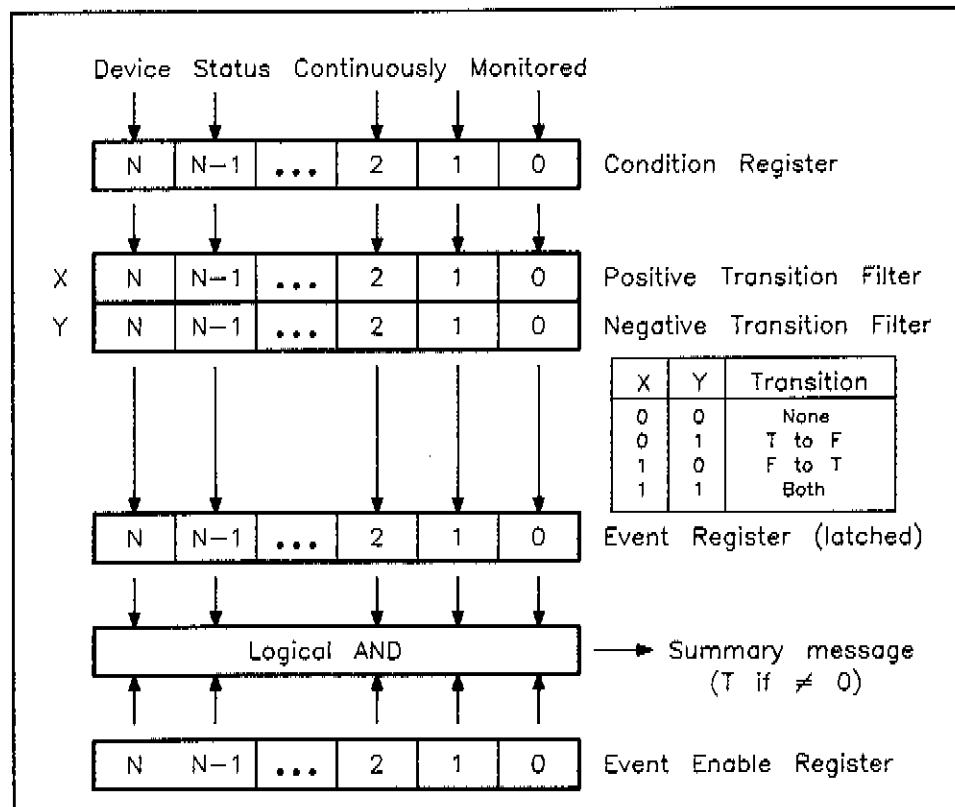
Figure 6-2. Status Register Map.
