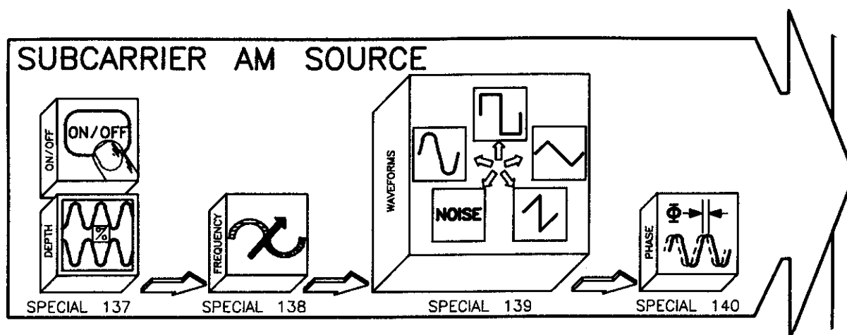
Figure 5-6. Block Diagram of the Subcarrier AM Source
