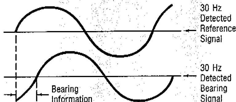
VOR Signal Seen at Aircraft Receiver
