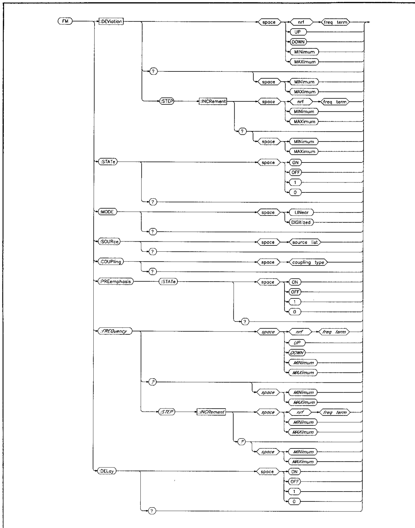
Figure 6-9. FM Subsystem.
