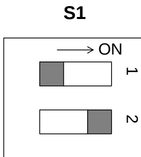
Figure 3-9: Switch Settings for Manual Impedance Control
