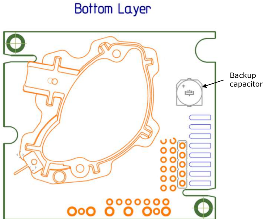
Figure 5, Backup capacitor
