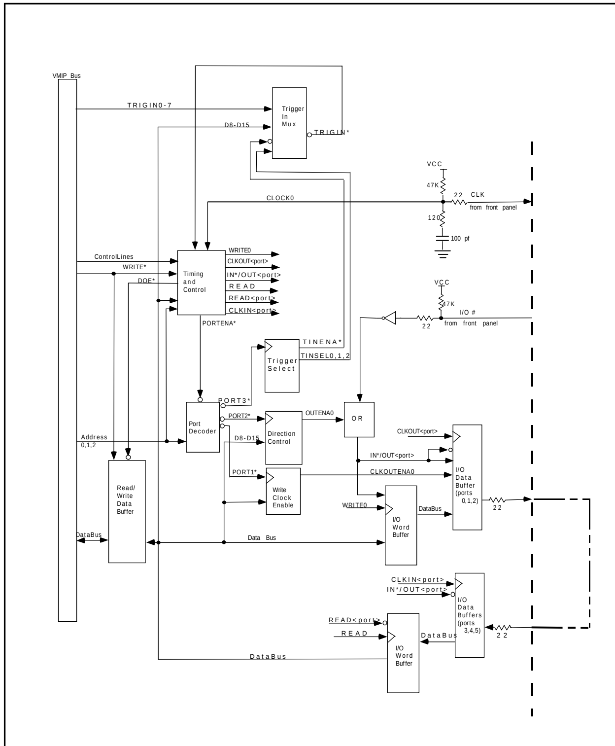
FIGURE 3-3: WRITE/READ
