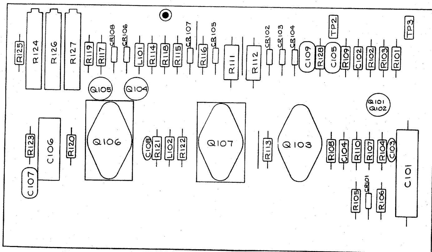
Figure 5-2. Circuit Board Layout
