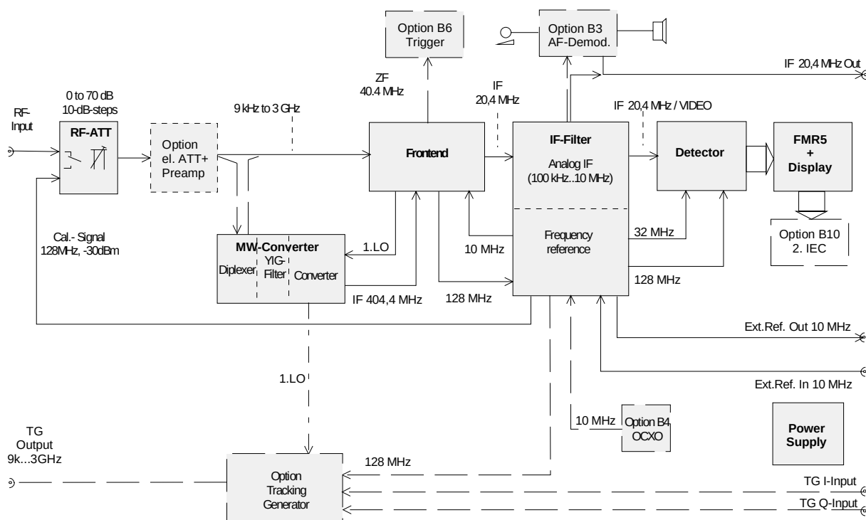
Fig. 3-1 Block diagram
