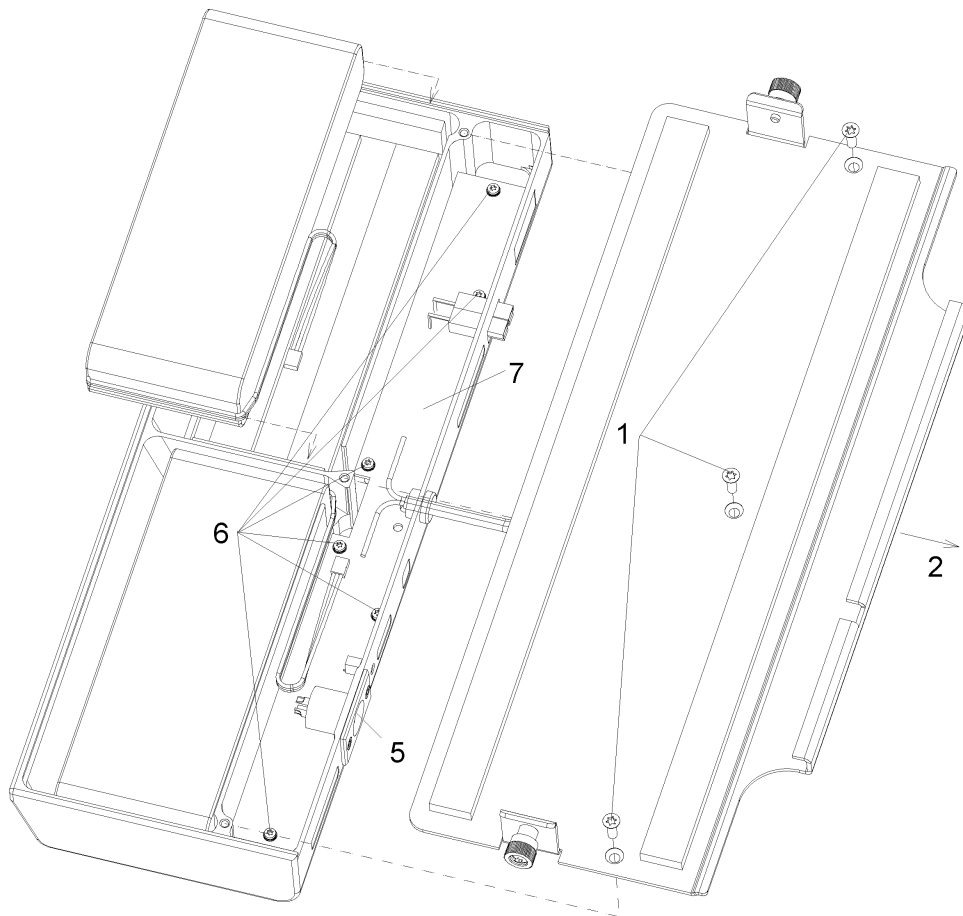
Fig. 3-1 Removing and installing the battery charger
