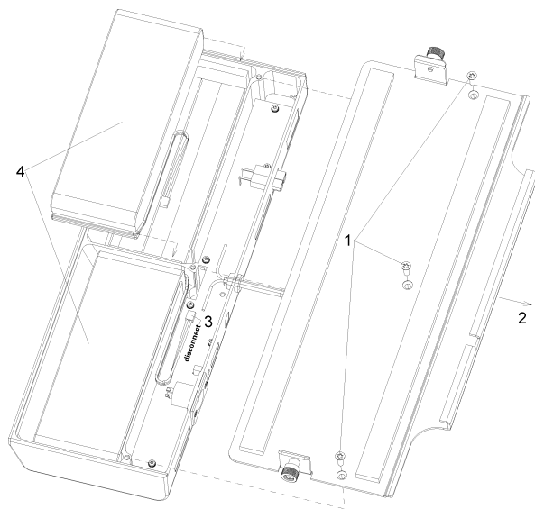
Fig. 3-2 Removing and installing the batteries
