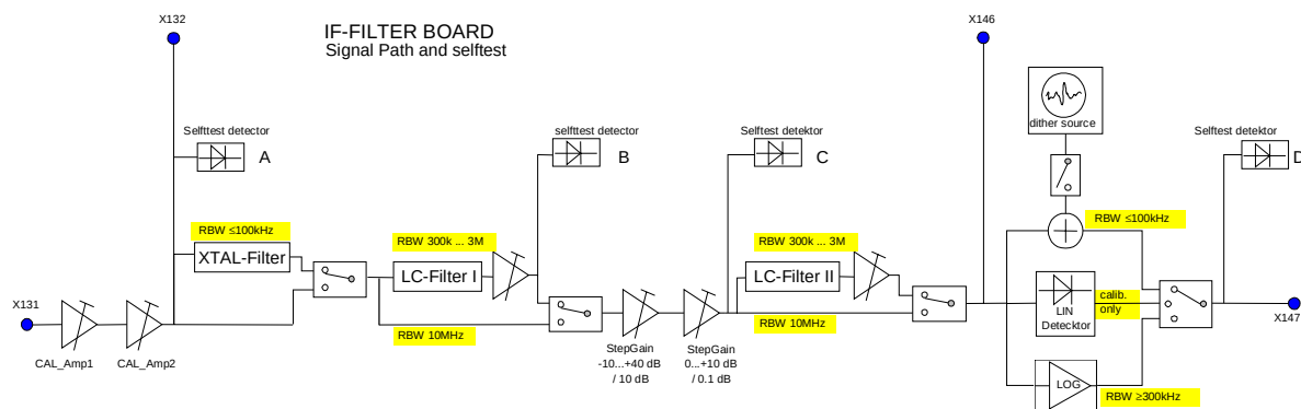
Fig. 3-4 IF filter
