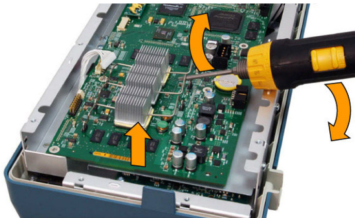
Figure 4-4: Disconnecting the main board
