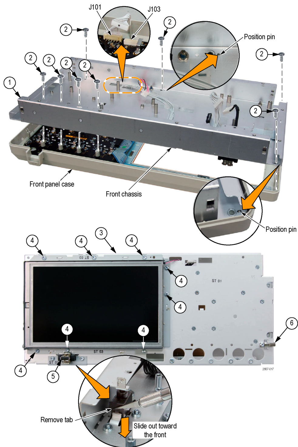
Figure 5-6: Exploded view: Front chassis and LCD assembly
