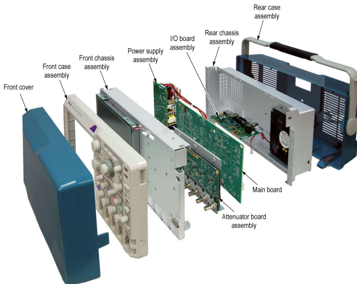
Figure 4-1: Locator for internal modules
