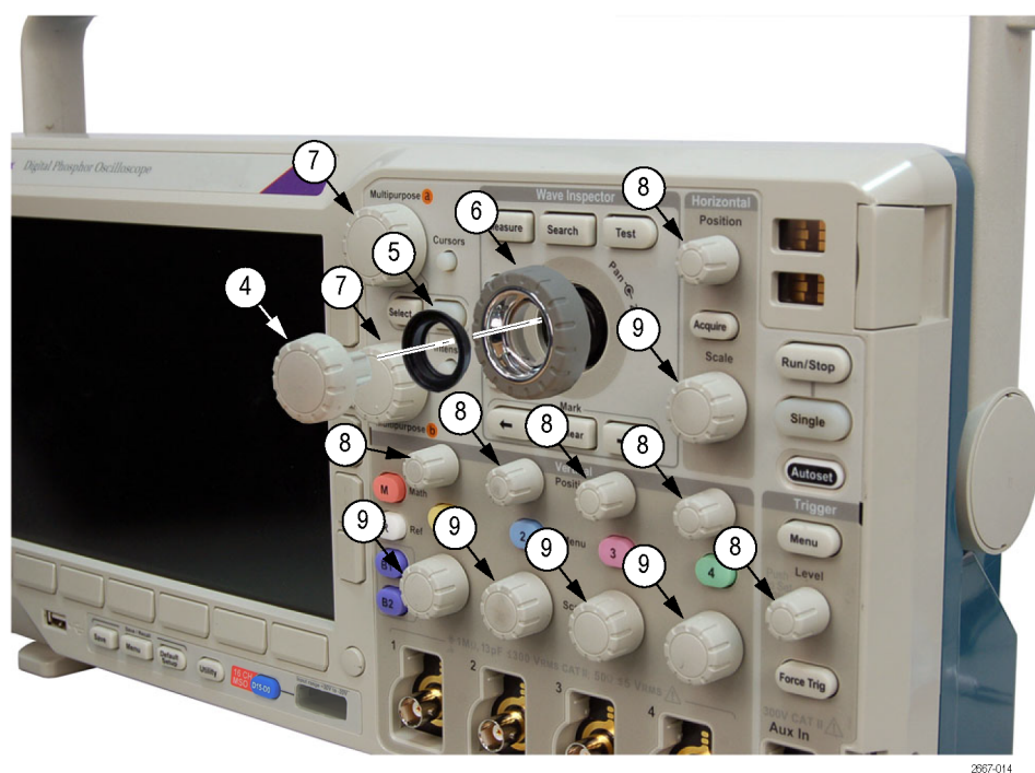
Figure 5-3: Exploded view: Front panel and power supply
