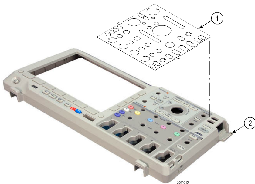
Figure 5-4: Exploded view: Front panel labels
