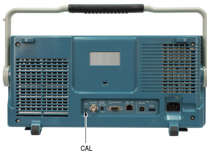
Figure 3-1: Rear panel
