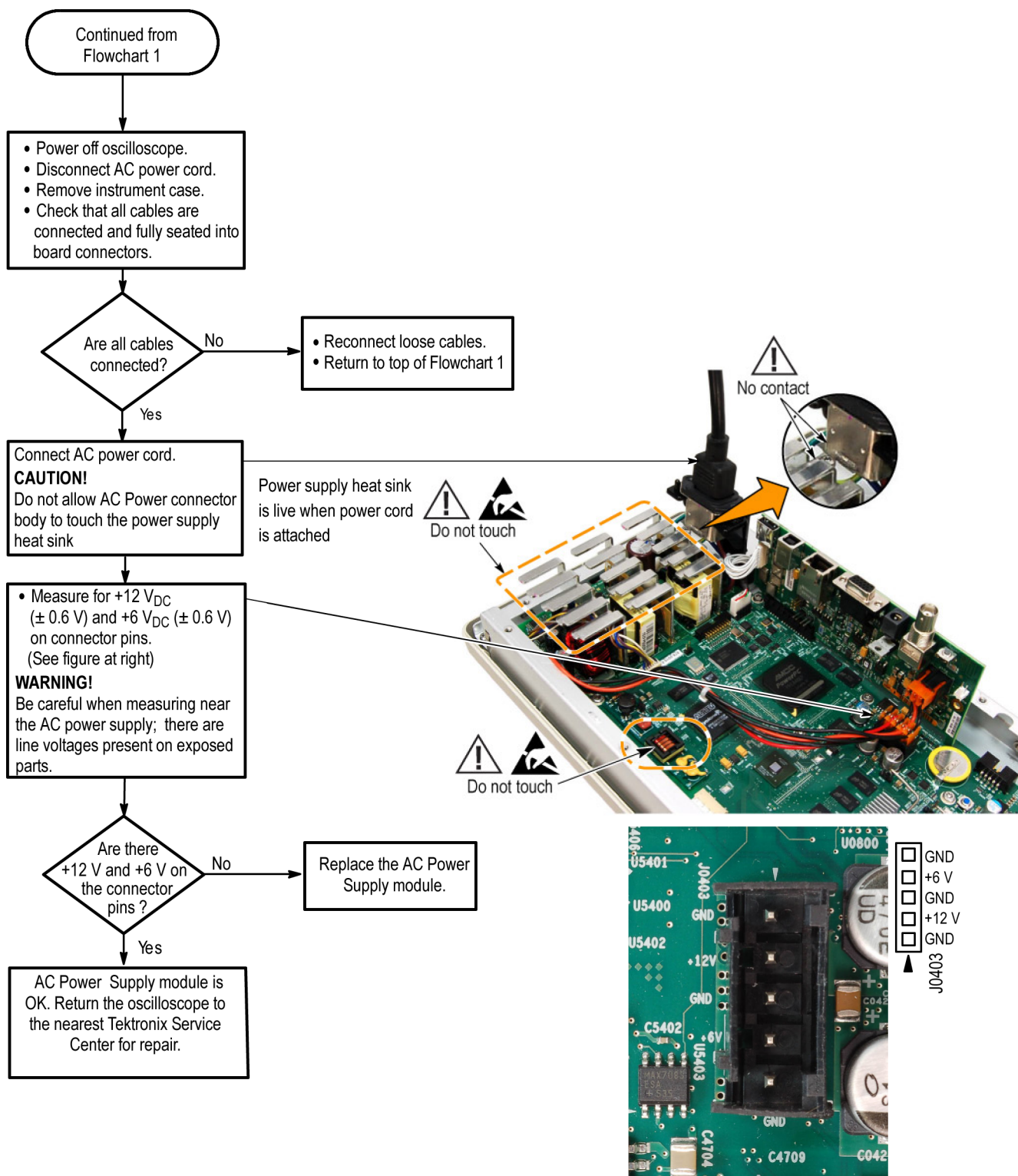
Flowchart 2 — AC power supply troubleshooting procedure
