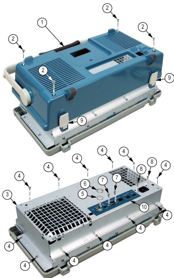
Figure 5-1: Exploded view: rear case and rear chassis
