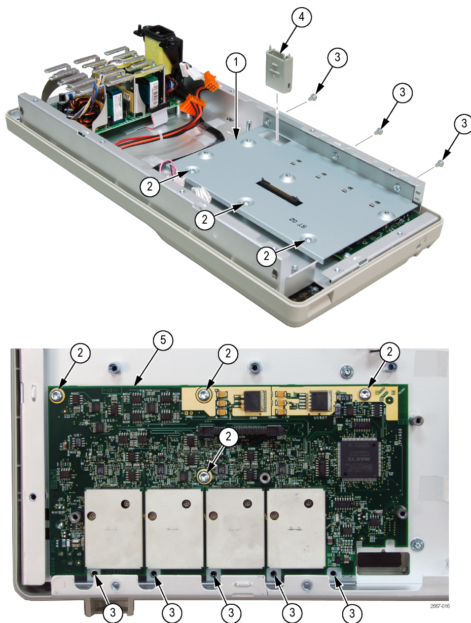
Figure 5-5: Exploded view: Main board shield and attenuator board
