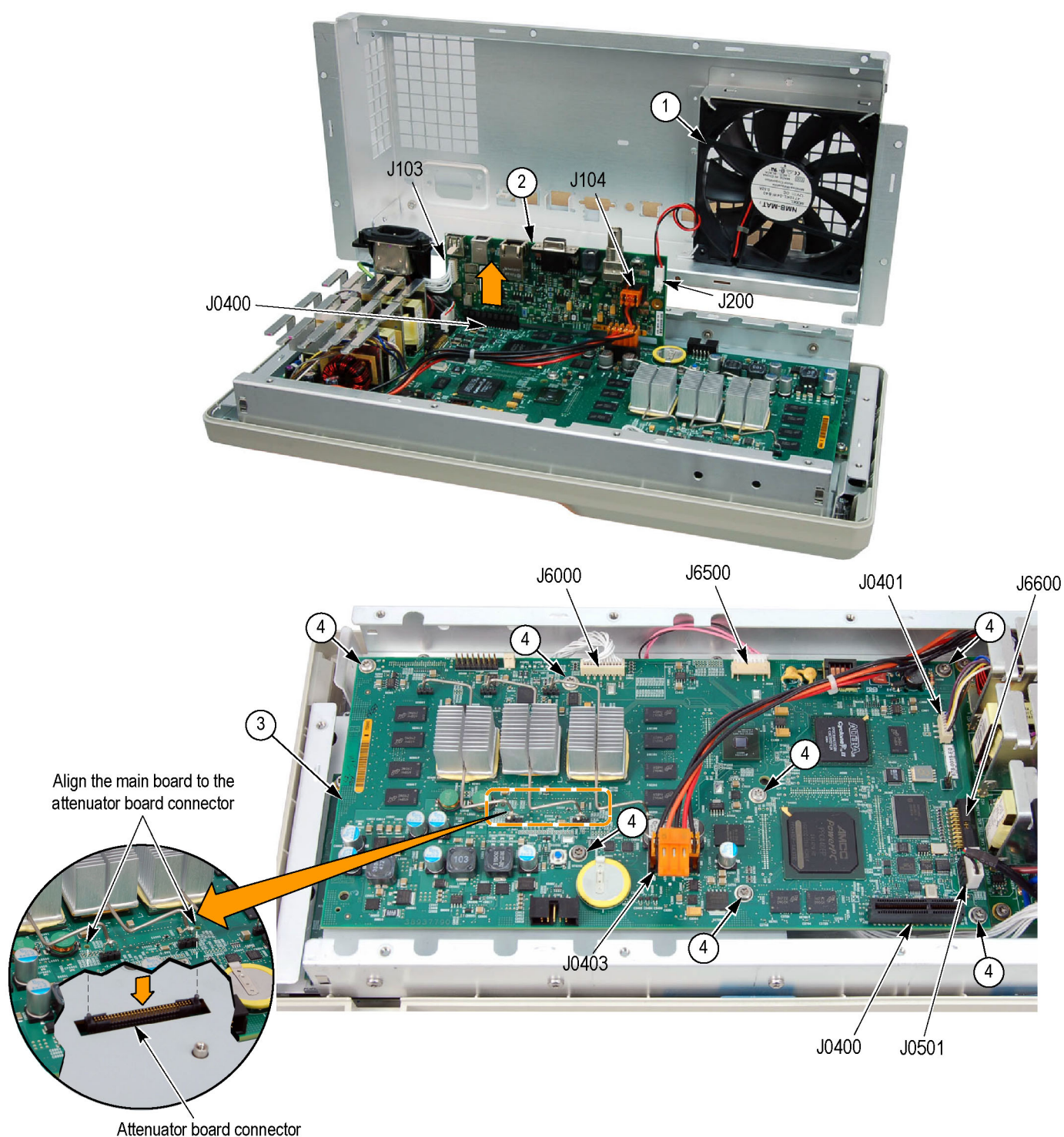
Figure 5-2: Exploded view: I/O and main boards
