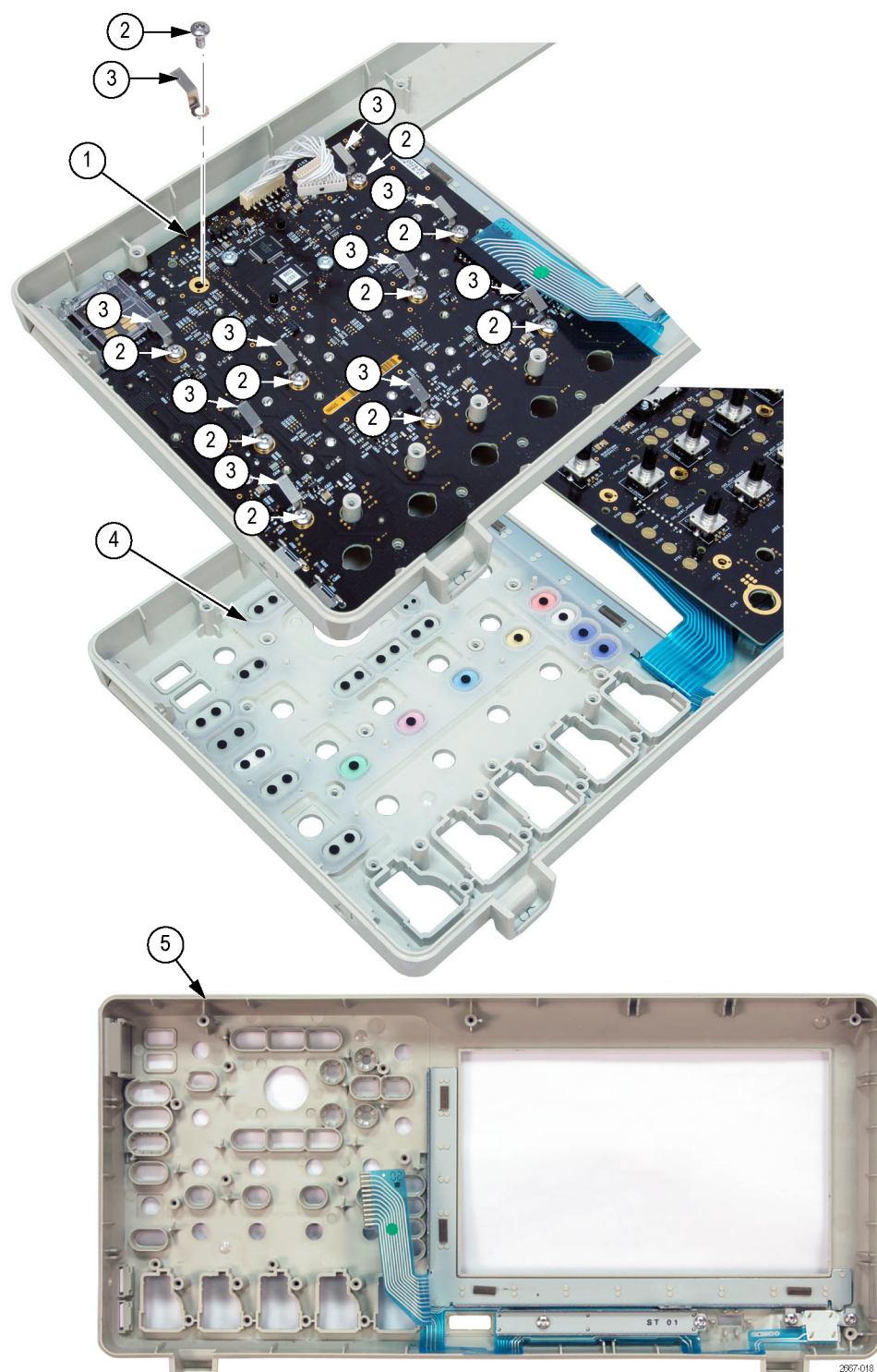
Figure 5-7: Exploded view: front panel board and front case
