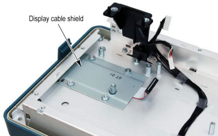
Figure 4-5: Display cable shield in place
