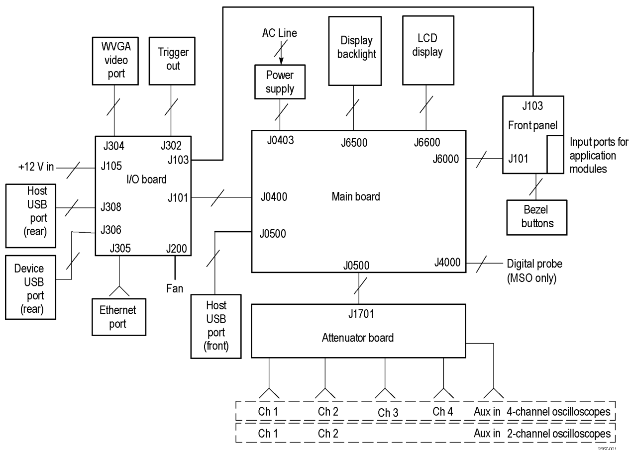
Figure 2-1: Oscilloscope module interconnections
