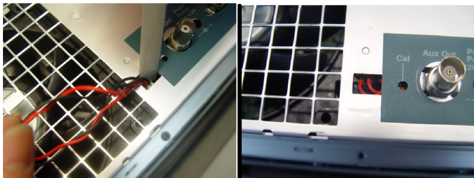
Figure 4-2: Reconnecting the fan cable
