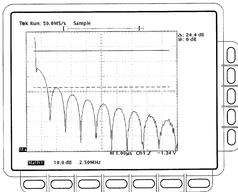
Figure 3–99: Cursor Measurement of an FFT Waveform
