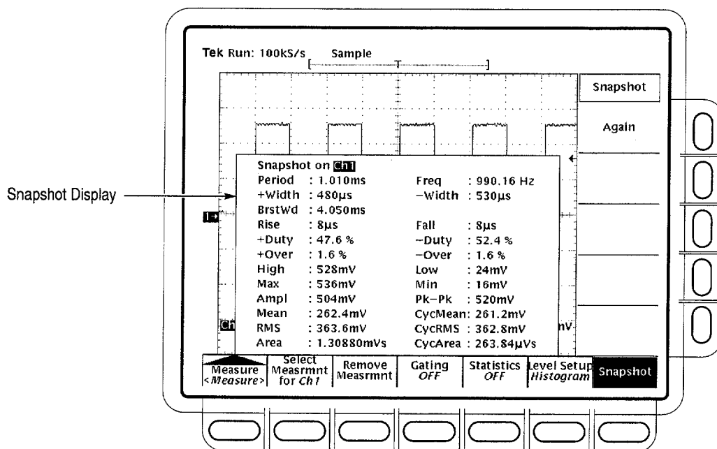
Figure 3-64: Snapshot Menu and Readout
