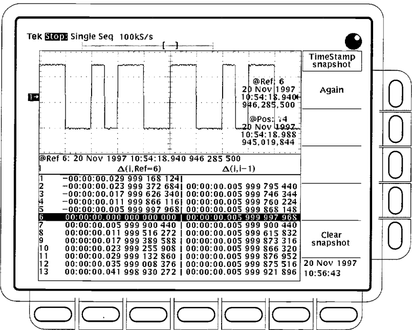
Figure 3–34: Horizontal Menu — FastFrame Snapshot
