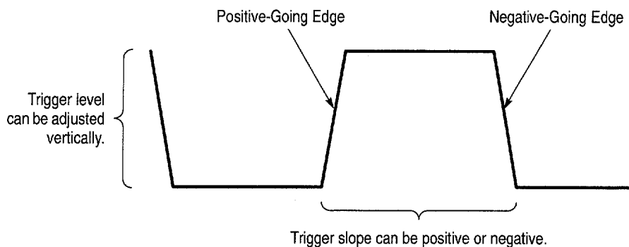
Figure 3–38: Slope and Level Controls Help Define the Trigger
