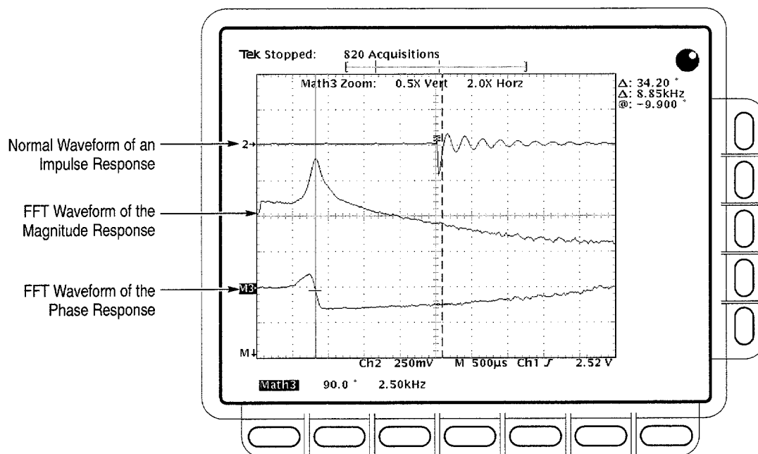
Figure 3-96: System Response to an Impulse
