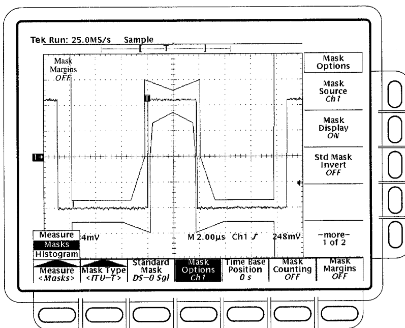
Figure 3–70: Mask menu
