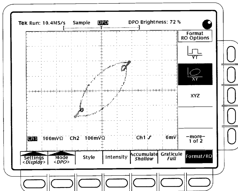
Figure 3–31: DPO XY Display
