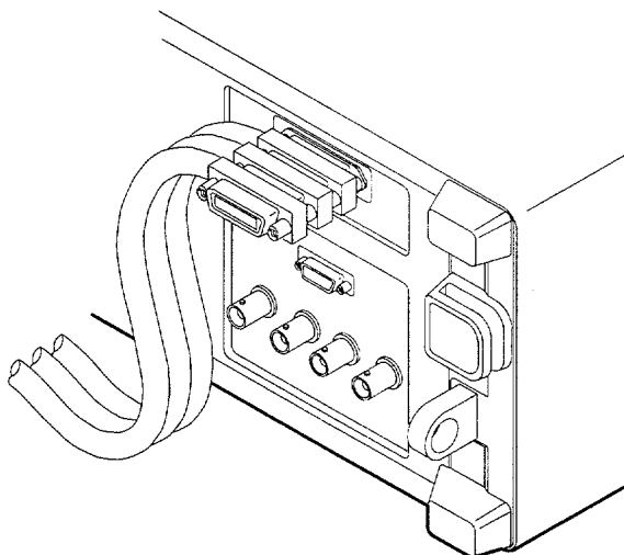
Figure 3-86: Stacking GPIB Connectors
