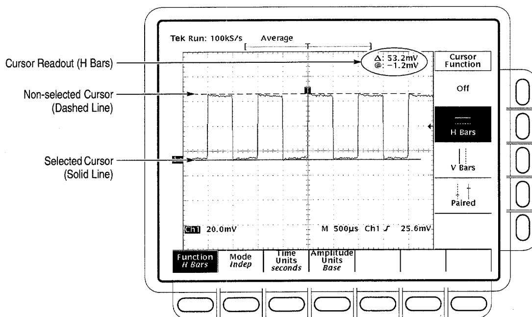
Figure 3–67: H Bars Cursor Menu and Readouts
