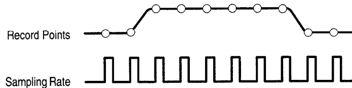
Figure 3–13: Real-Time Sampling
