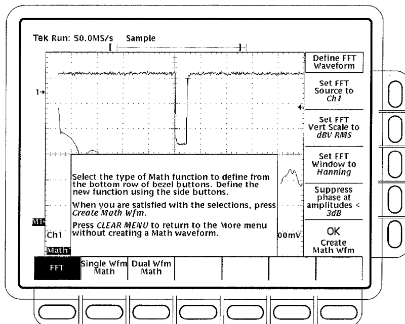
Figure 3-97: Define FFT Waveform Menu
