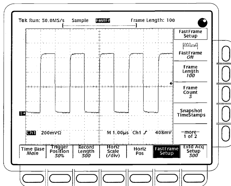
Figure 3–33: Horizontal Menu — FastFrame Setup
