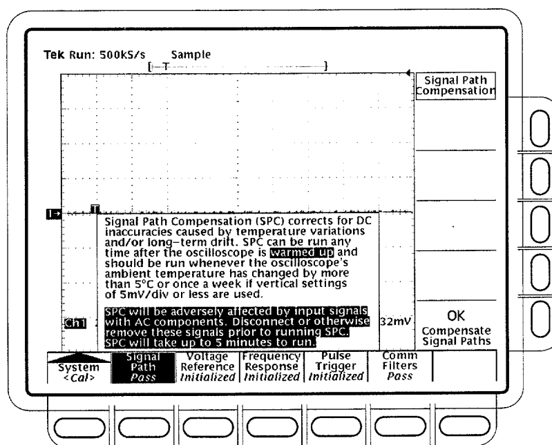
Figure 3–72: Performing a Signal Path Compensation
