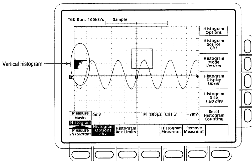
Figure 3–69: Histogram Menu and Vertical Histogram
