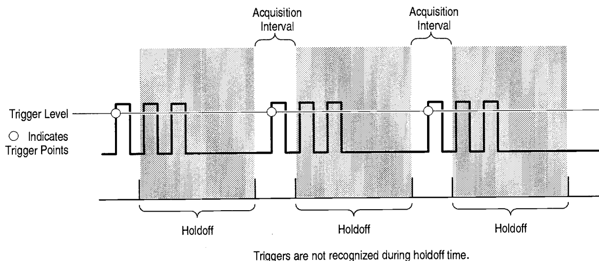
Figure 3-37: Trigger Holdoff Time Ensures Valid Triggering
