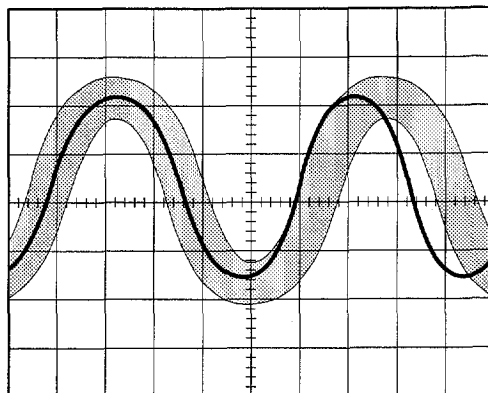
Figure 3-92: Comparing a Waveform to a Limit Template
