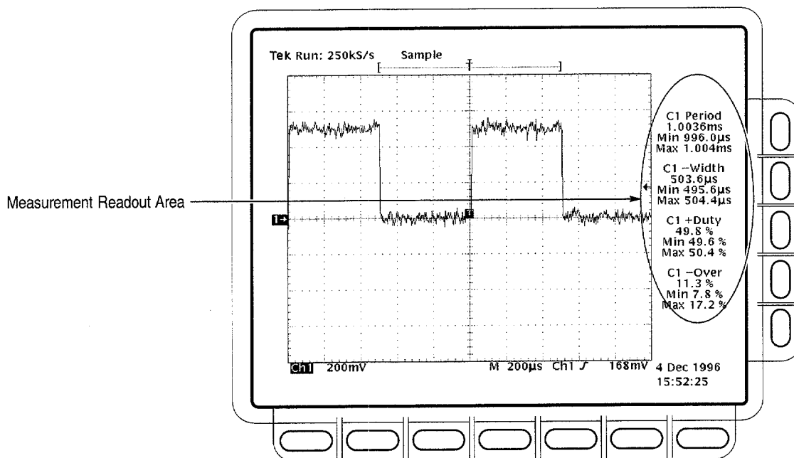
Figure 3-59: Measurement Readouts with Statistics
