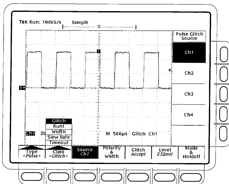
Figure 3-50: Main Trigger Menu — Glitch Class
