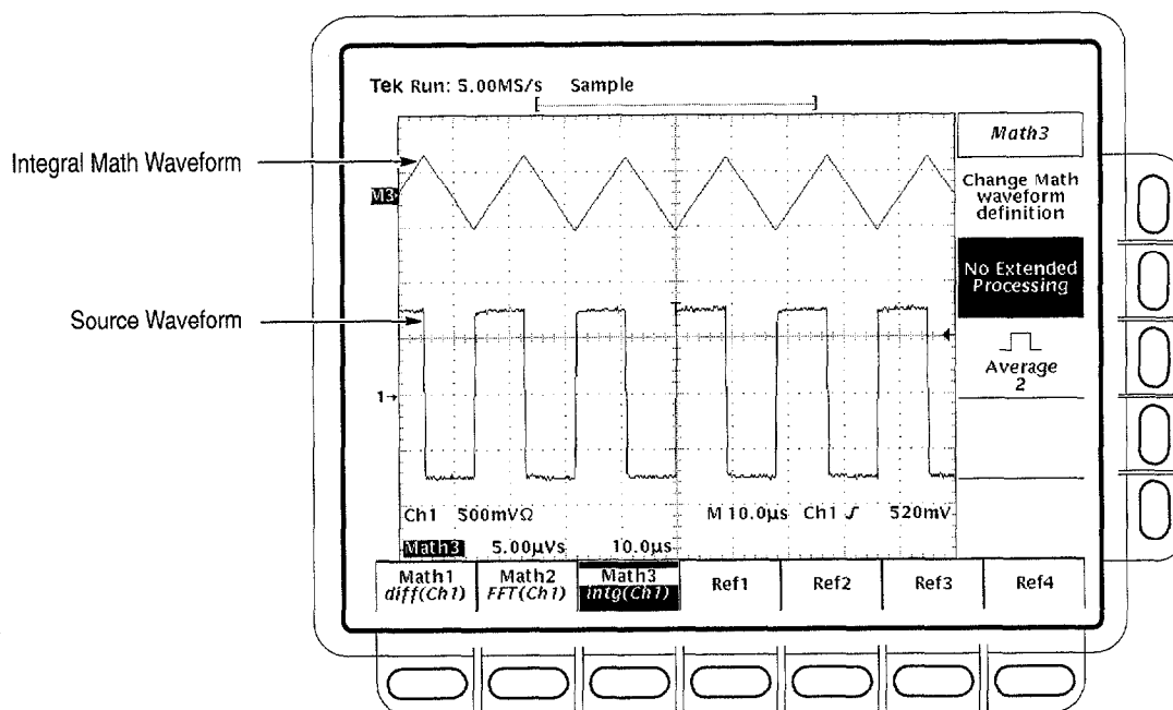
Figure 3-107: Integral Math Waveform
