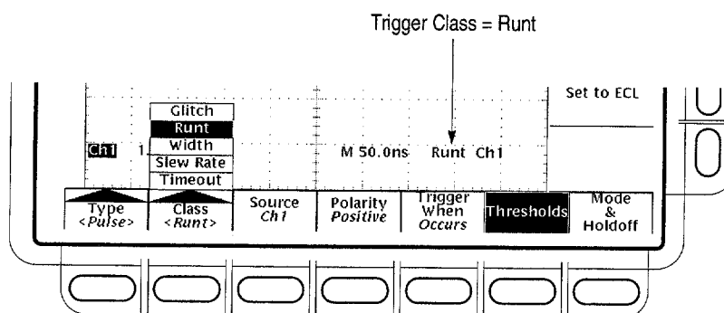
Figure 3-49: Pulse Trigger Readouts
