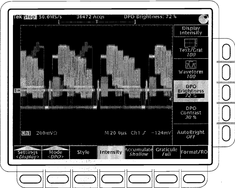
Figure 3–29: DPO Display
