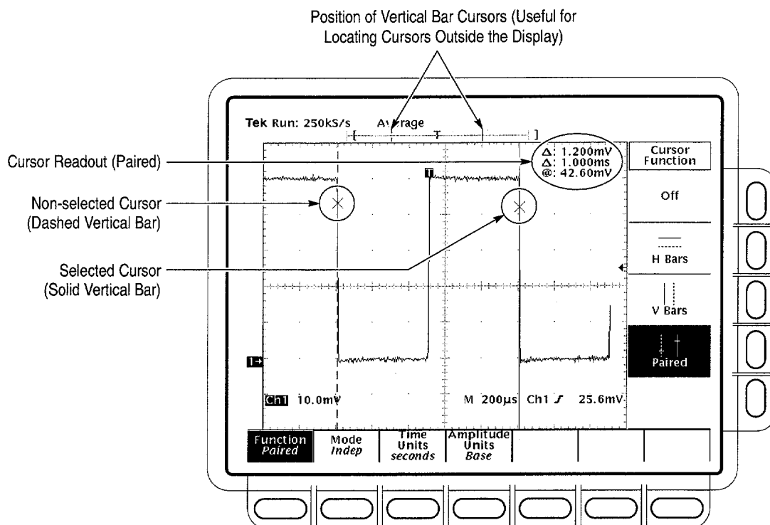
Figure 3–68: Paired Cursor Menu and Readouts
