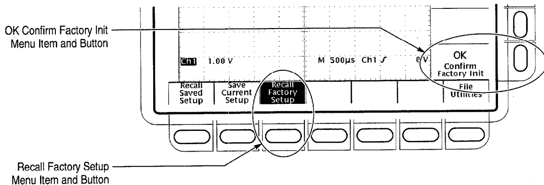
Figure 2-3: The Setup Menu
