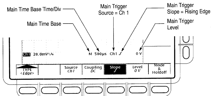
Figure 3-42: Edge Trigger Readouts
