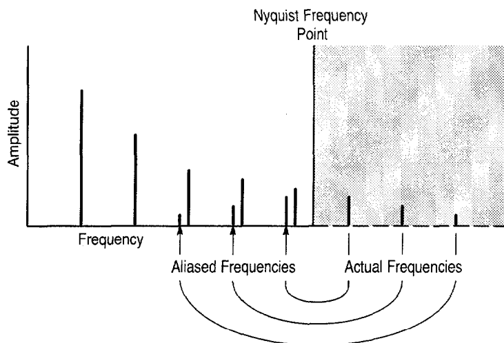
Figure 3-102: How Aliased Frequencies Appear in an FFT
