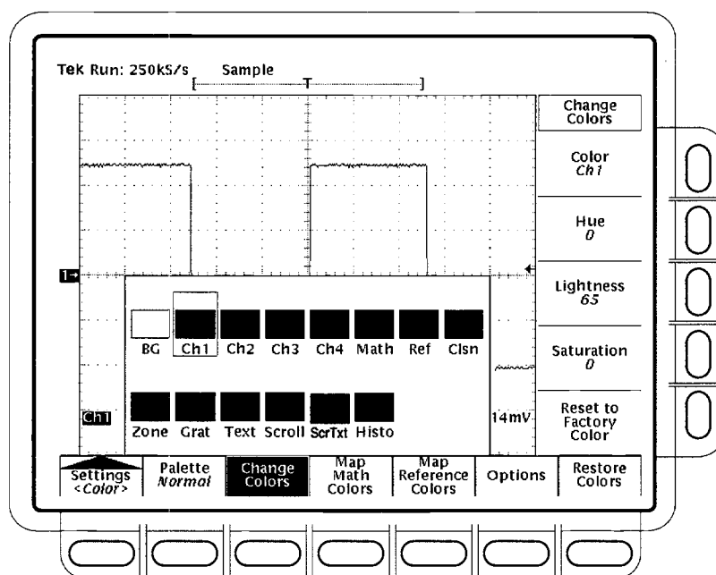
Figure 3-22: Display Menu — Palette Colors
