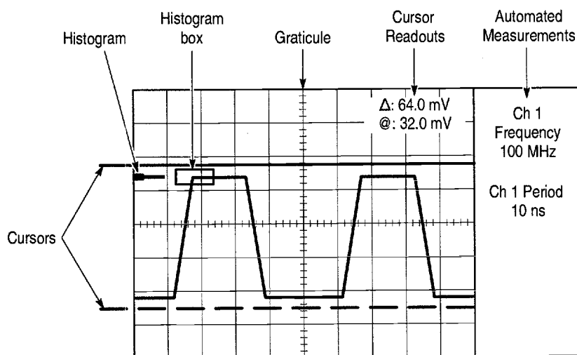
Figure 3-58: Histogram, Graticule, Cursor and Automated Measurements
