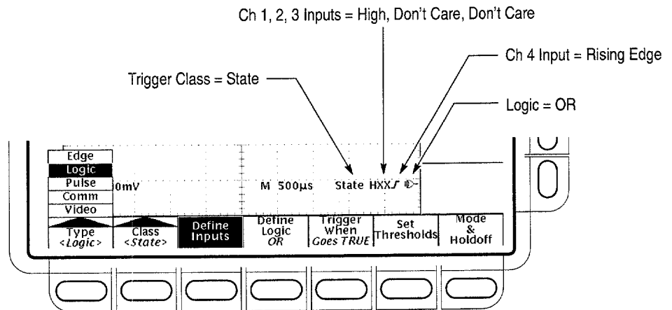
Figure 3-45: Logic Trigger Readouts — State Class Selected
