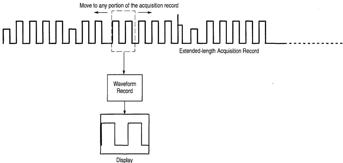
Figure 3–9: Displaying an Extended Acquisition Length Record
