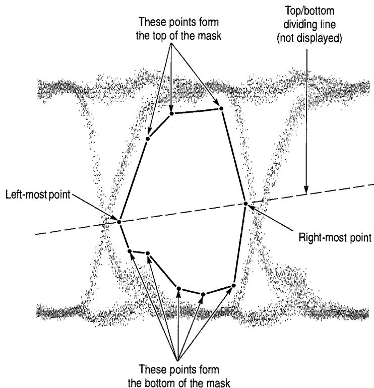
Figure 3-71: Creating a User Mask
