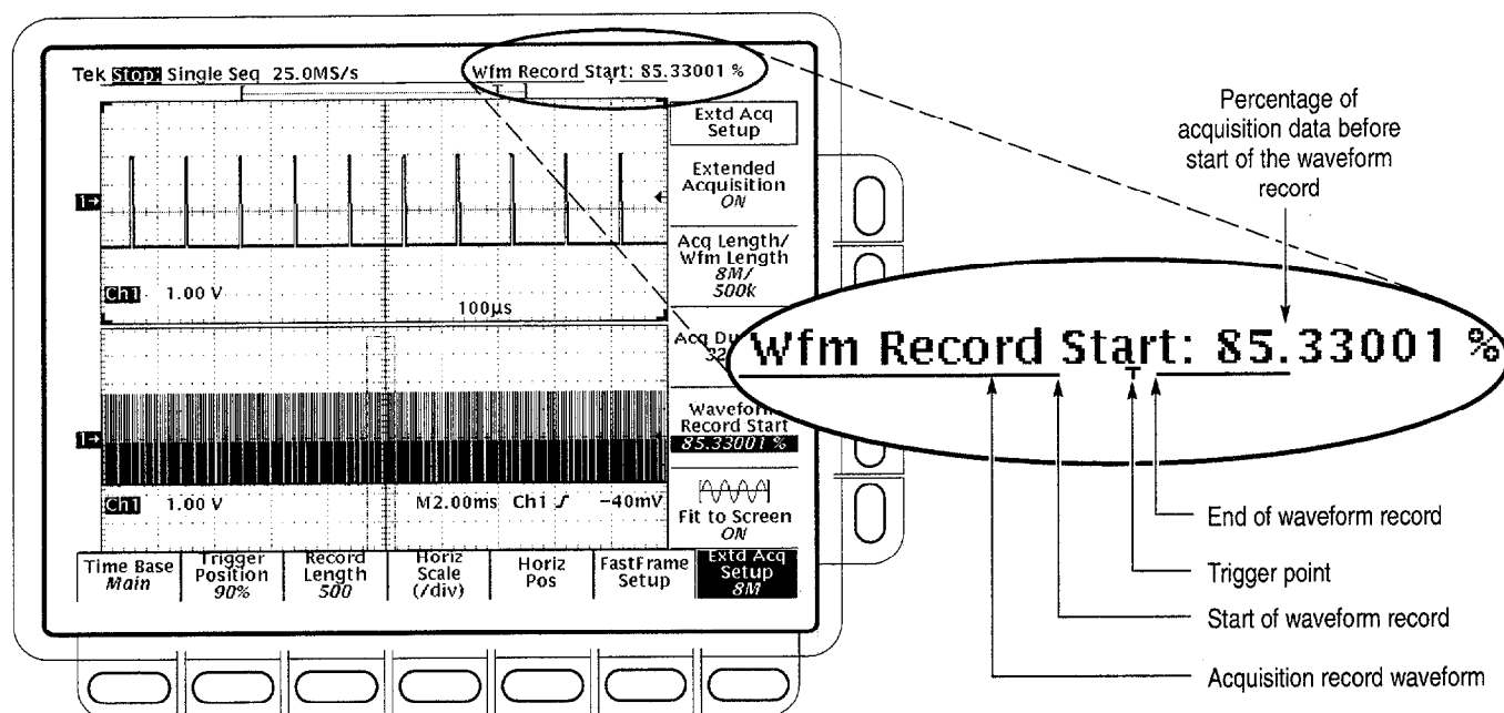
Figure 3–10: Extended Acquisition Length and Zoom
