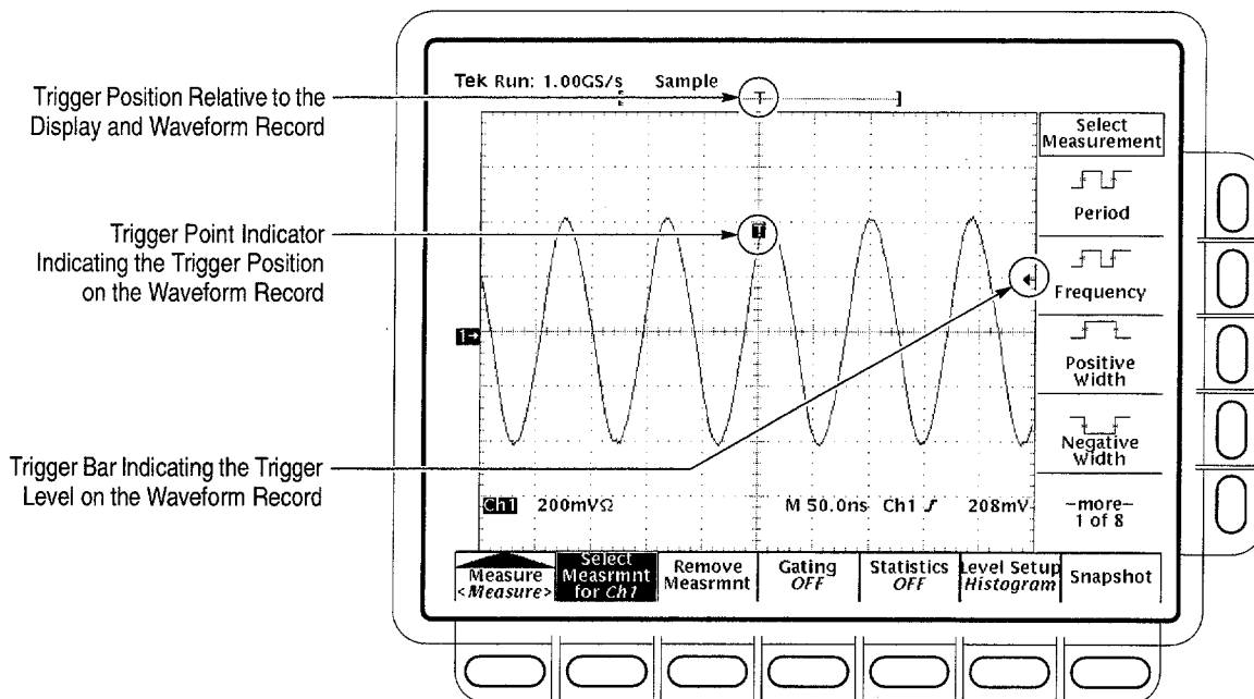
Figure 3-41: Record View, Trigger Position, and Trigger Level Bar Readouts
