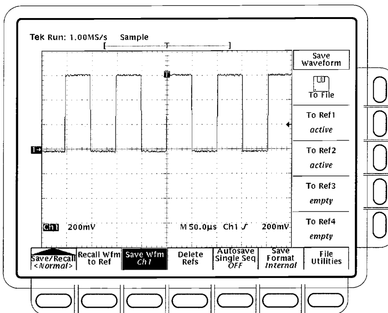
Figure 3-76: Save Waveform Menu
