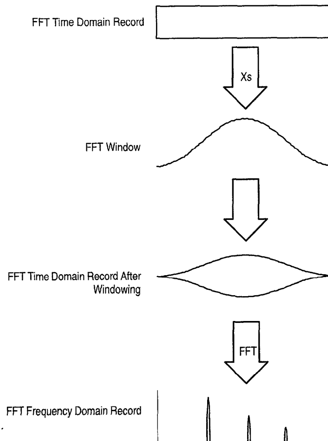
Figure 3-103: Windowing the FFT Time Domain Record
