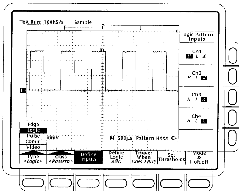
Figure 3-46: Logic Trigger Menu
