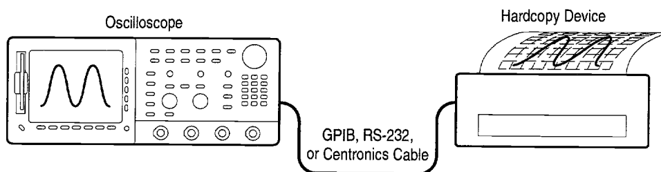
Figure 3–83: Connecting the Oscilloscope Directly to the Hardcopy Device
