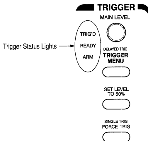
Figure 3–39: TRIGGER Controls and Status Lights
