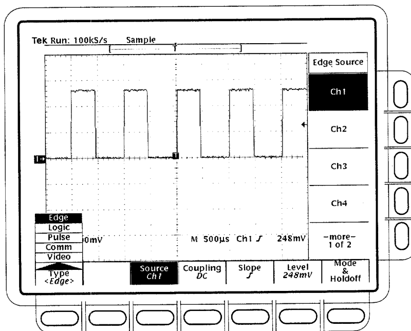
Figure 3-43: Main Trigger Menu — Edge Type
