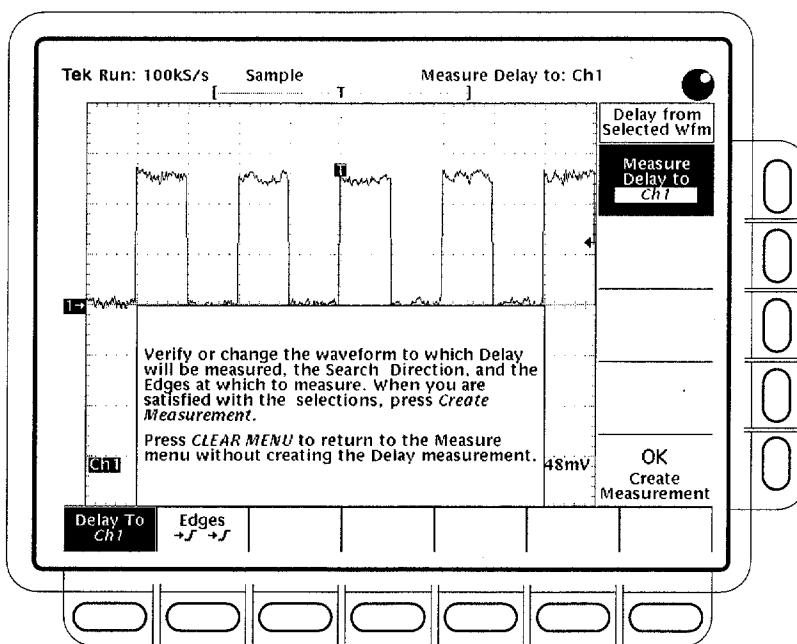
Figure 3-63: Measure Delay Menu — Delay To
