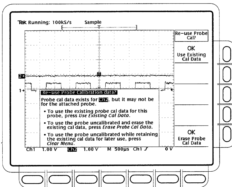
Figure 3–74: Re-use Probe Calibration Data Menu
