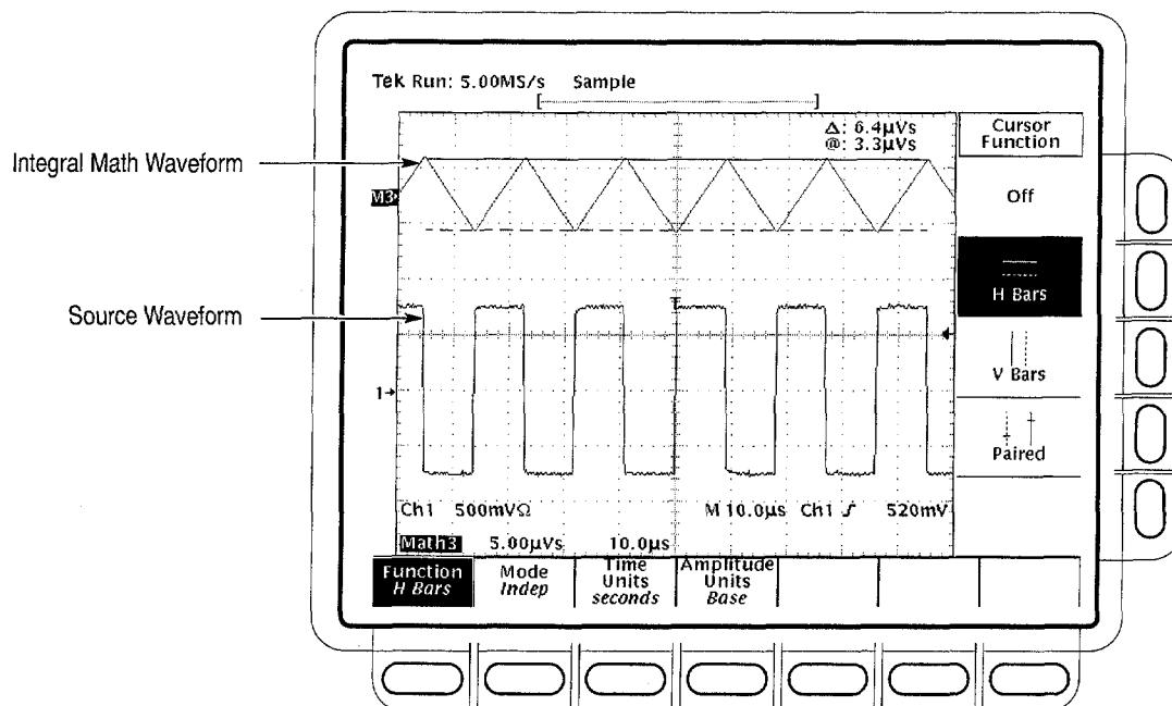
Figure 3-108: H Bars Cursors Measure an Integral Math Waveform
