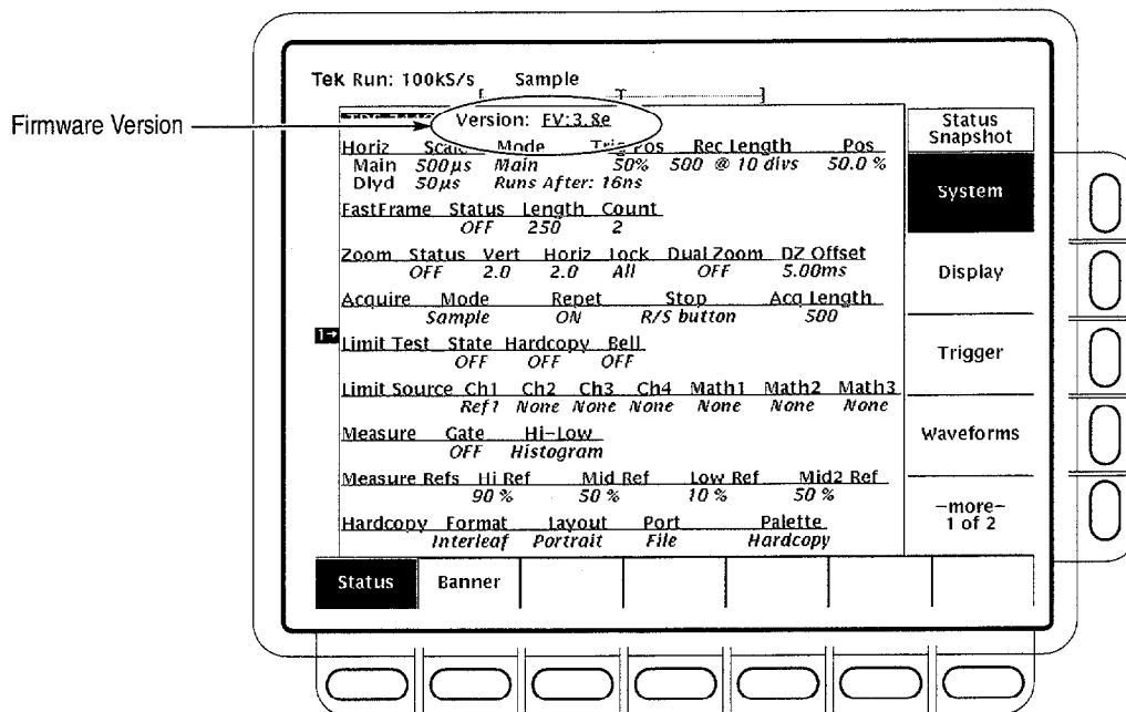
Figure 3-89: Status Menu — System
