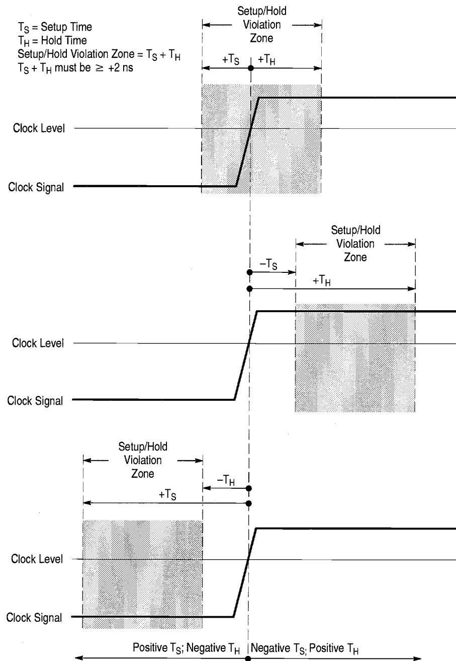
Figure 3-44: Violation Zones for Setup/Hold Triggering
