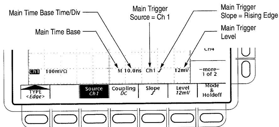
Figure 3–40: Example Trigger Readouts — Edge Trigger Selected
