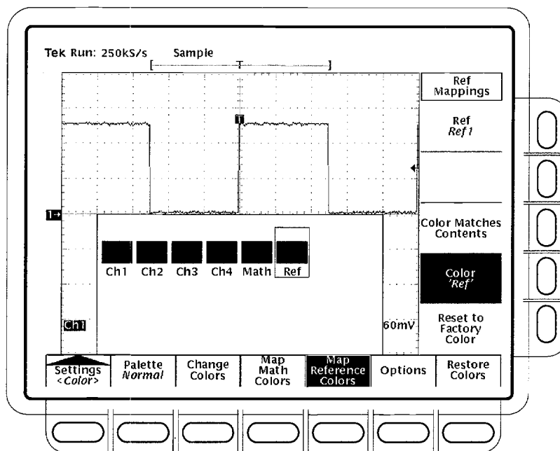
Figure 3-23: Display Menu — Map Reference Colors
