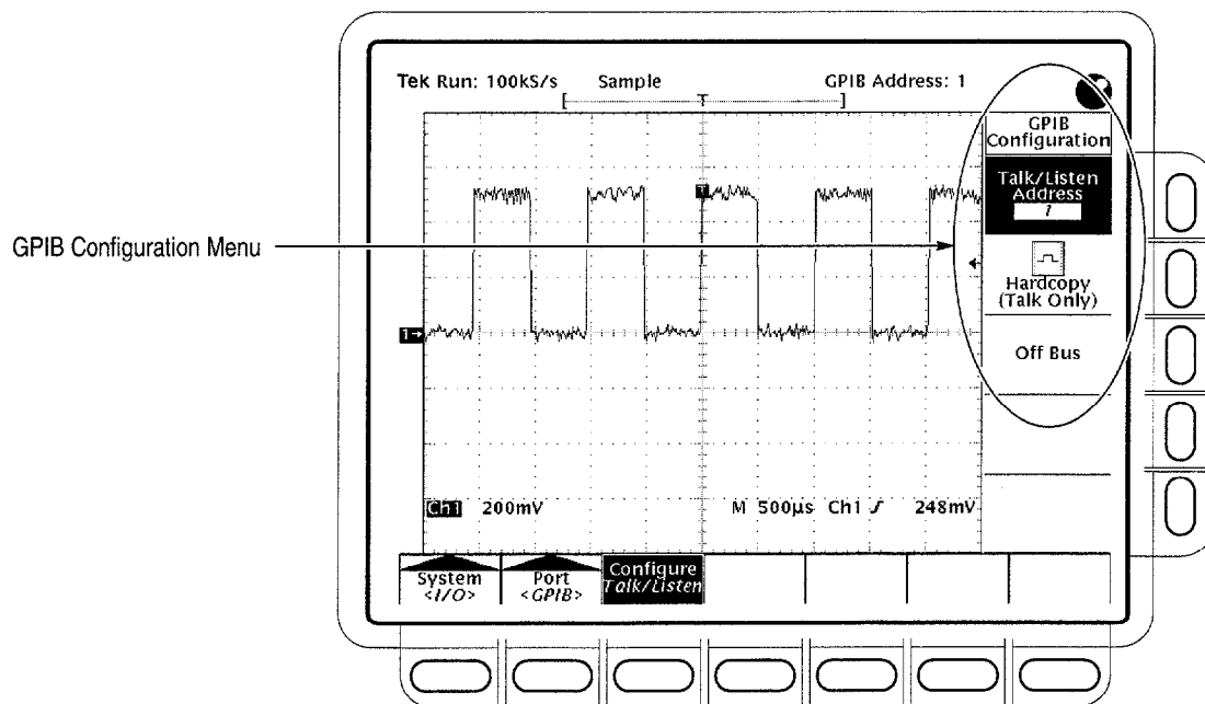
Figure 3-88: Utility Menu
