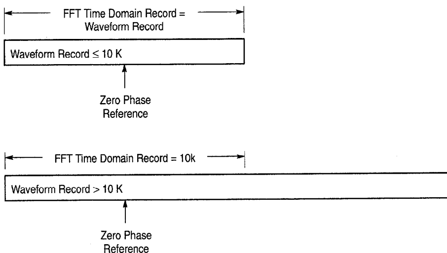
Figure 3–100: Waveform Record vs. FFT Time Domain Record
