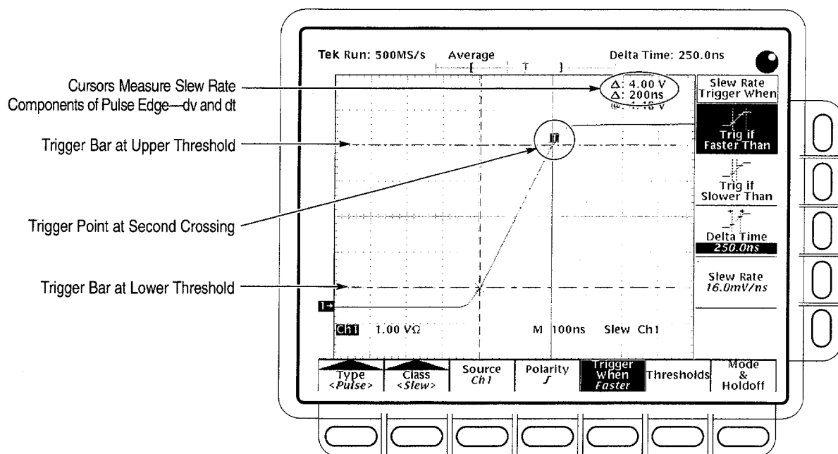
Figure 3-52: Main Trigger Menu — Slew Rate Class
