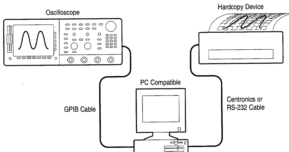
Figure 3–84: Connecting the Oscilloscope and Hardcopy Device Via a PC
