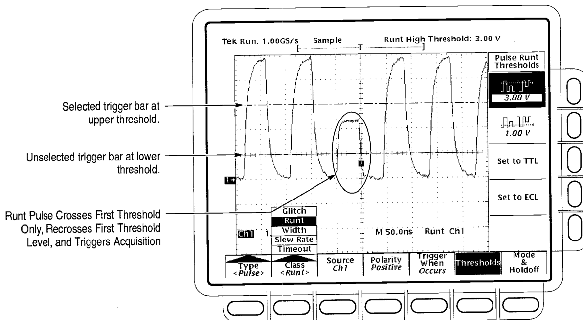
Figure 3-51: Main Trigger Menu — Runt Class
