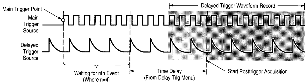
Figure 3-56: How the Delayed Triggers Work
