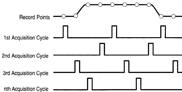
Figure 3–14: Equivalent-Time Sampling
