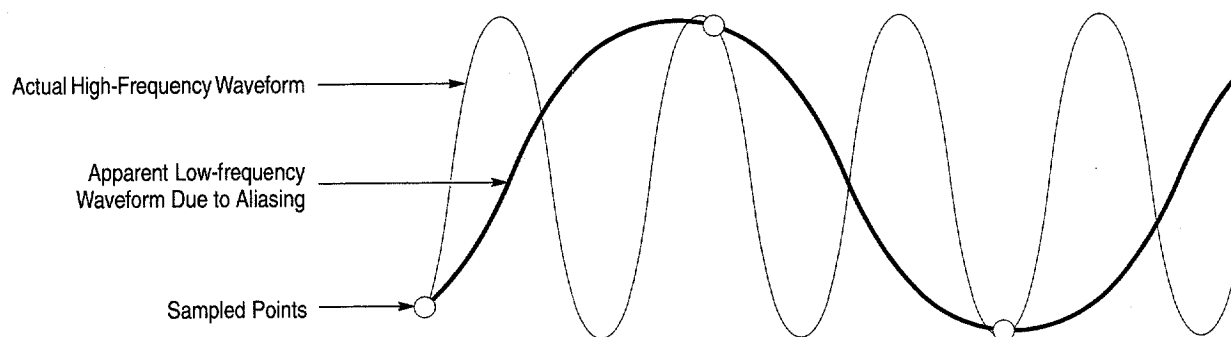
Figure 3–18: Aliasing
