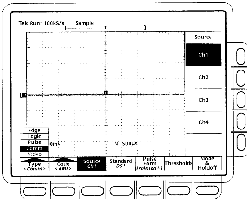
Figure 3–53: Main Trigger Menu — Comm Type
