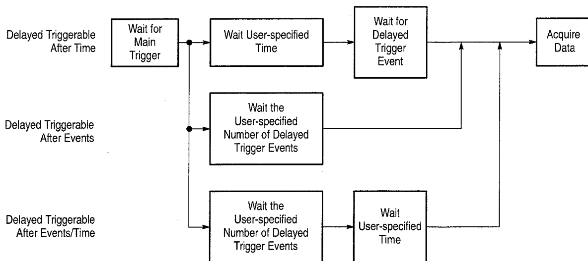
Figure 3–55: Delayed Triggerable
