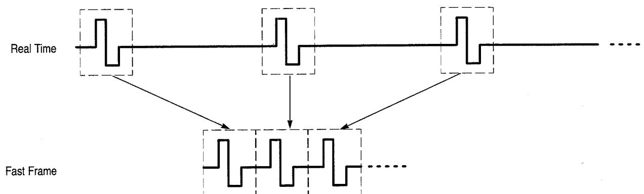
Figure 3–32: Fast Frame
