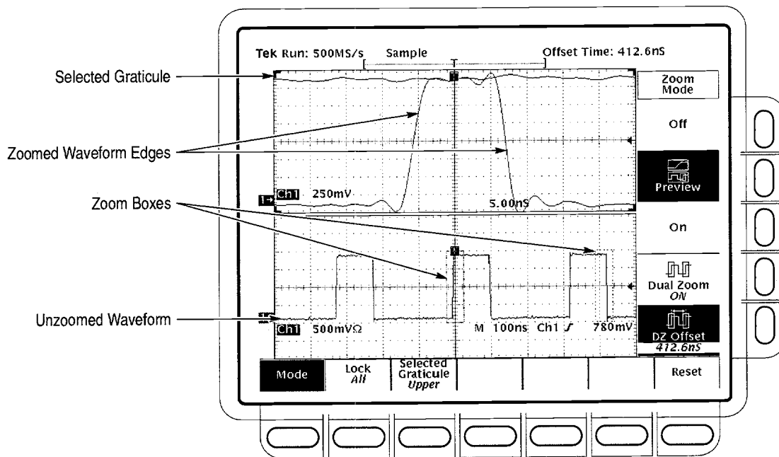
Figure 3-27: Dual Zoom — Shown Dual Window (Preview) Mode
