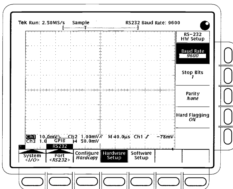
Figure 3–80: Utility Menu — System I/O
