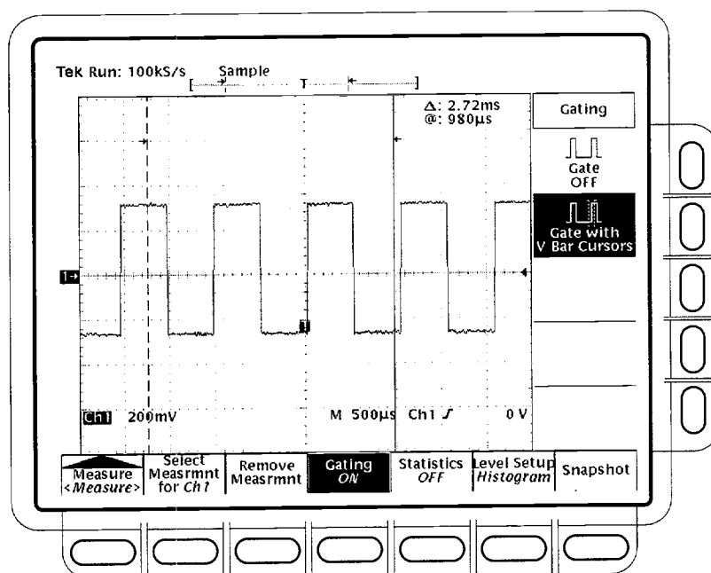
Figure 3–61: Measure Menu — Gating
