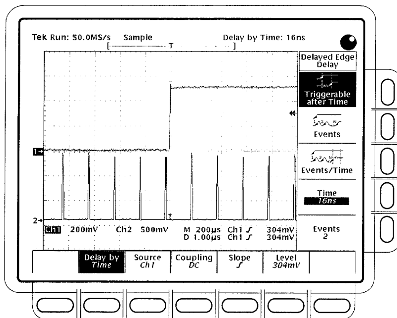
Figure 3–57: Delayed Trigger Menu
