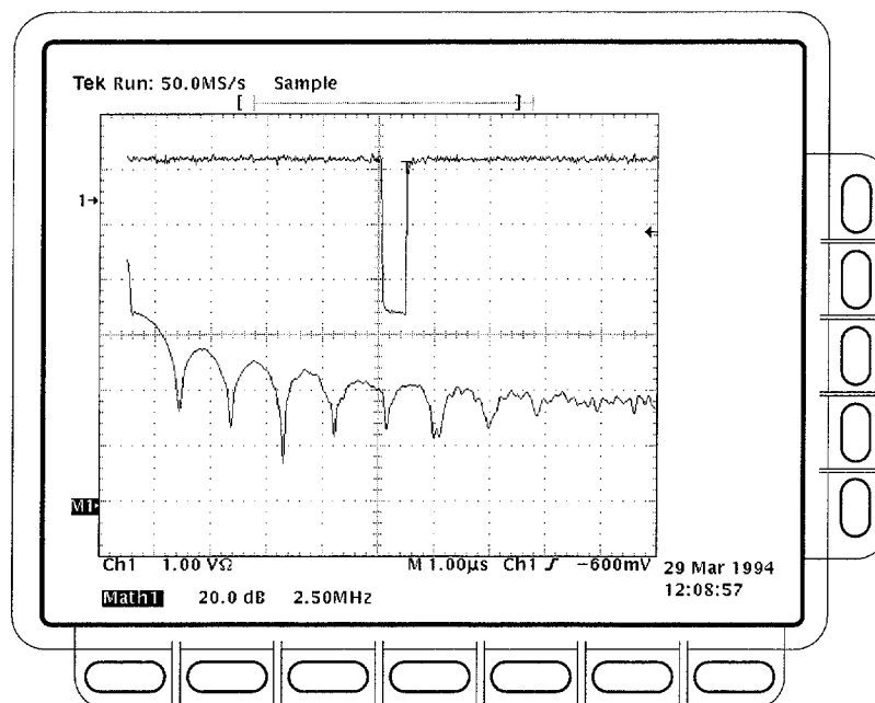
Figure 3-98: FFT Math Waveform in Math1
