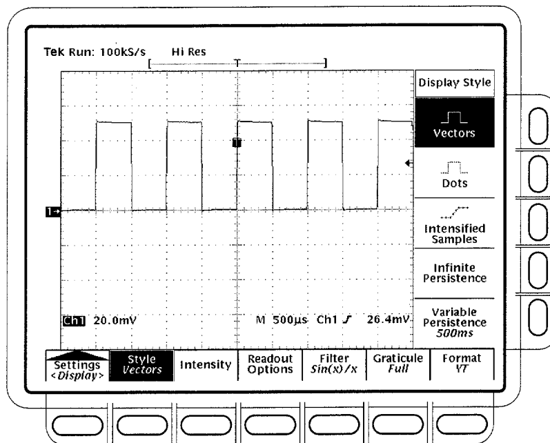
Figure 3-19: Display Menu — Style
