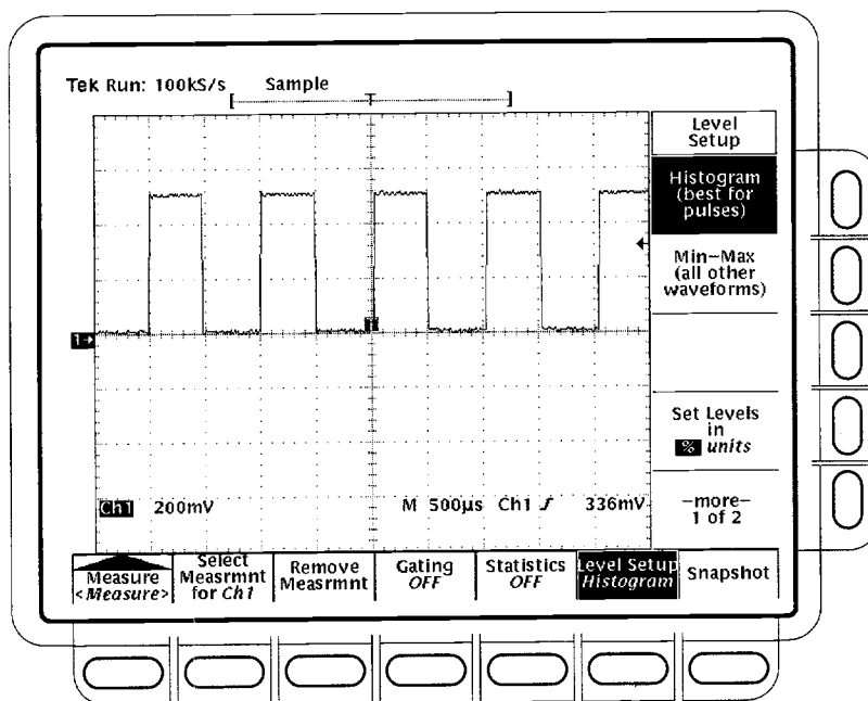
Figure 3-62: Measure Menu — Reference Levels
