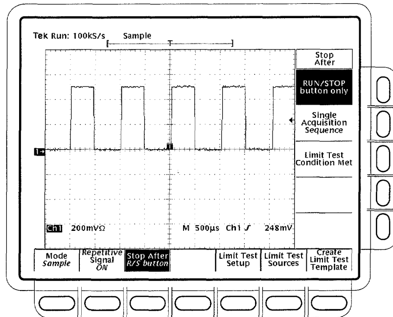
Figure 3-17: Acquire Menu — Stop After
