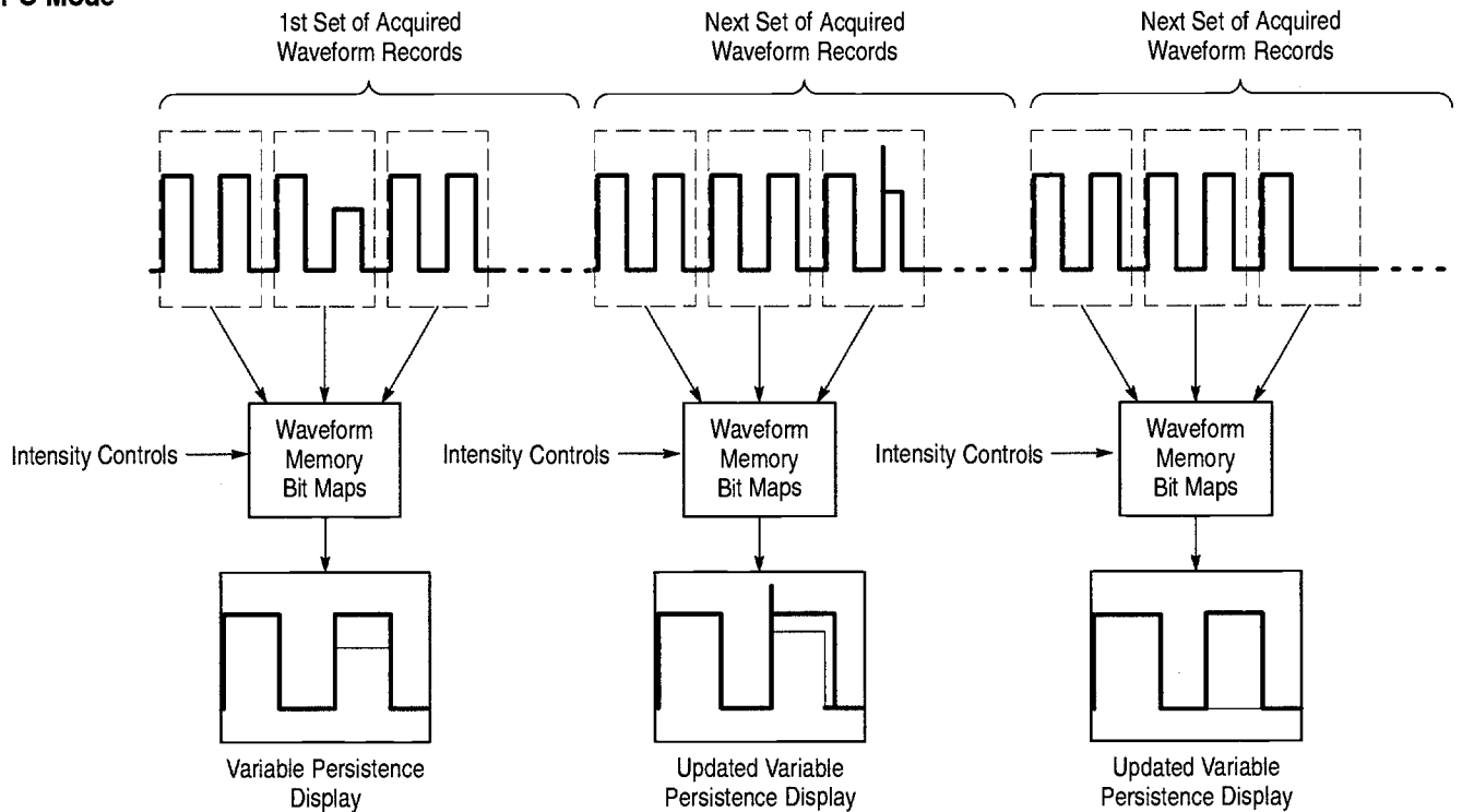
Figure 3–28: Normal DSO Acquisition and Display Mode Versus DPO Mode
