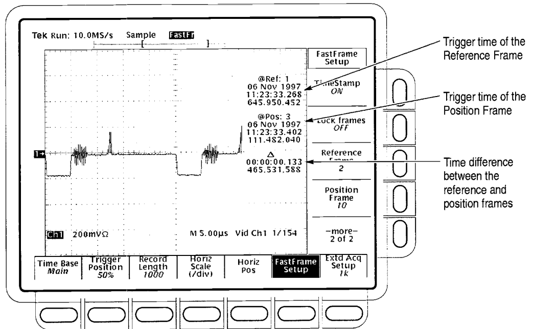
Figure 3-35: FastFrame TimeStamp
