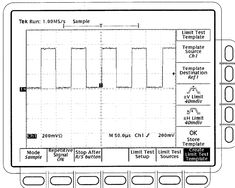
Figure 3-93: Acquire Menu — Create Limit Test Template
