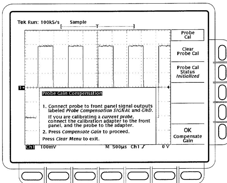
Figure 3–73: Probe Cal Menu and Gain Compensation Display
