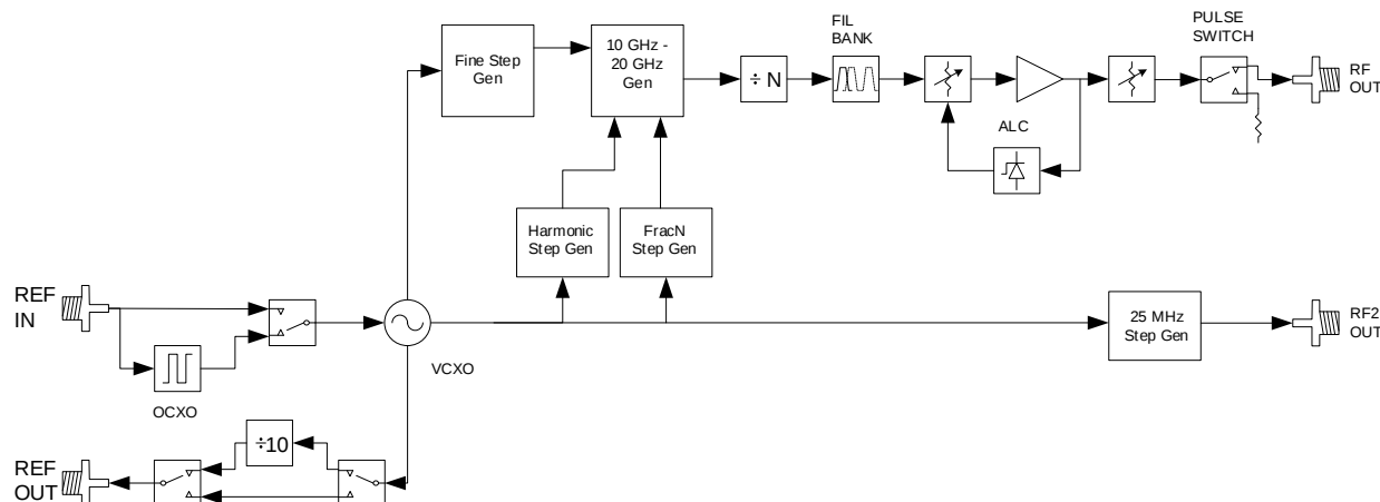
Figure 1. SC5510B/SC5511B Block Diagram
