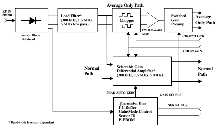
Figure 11 Simplified Sensor Block Diagram
