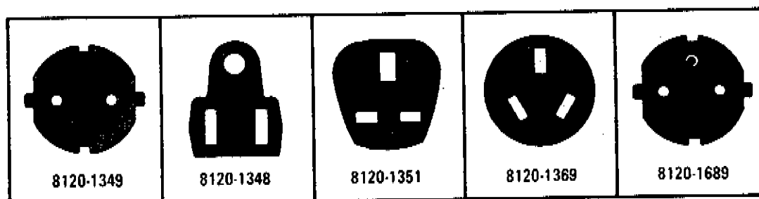
Figure 2-1. Power Cable Line Connector Labels
