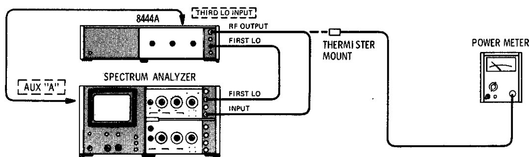
Figure 5-8. Level Control Calibration Check and Adjustment Test Setup
