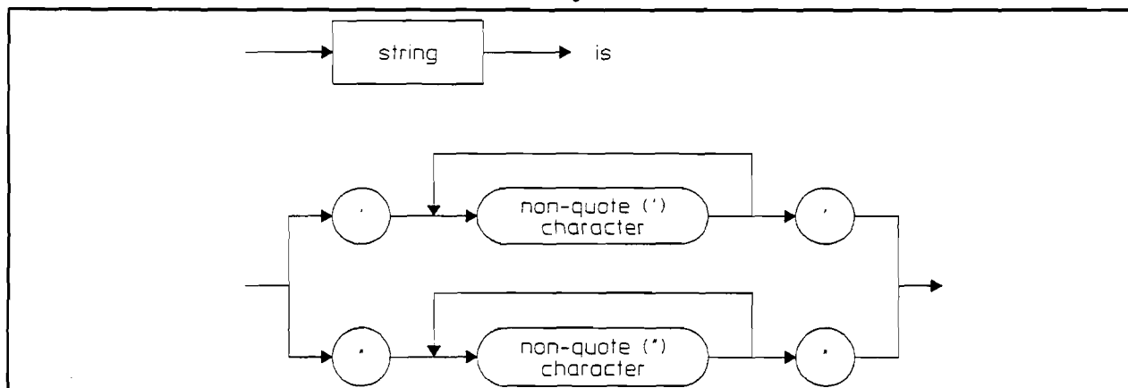
Figure 2-5. Definition of "String"
