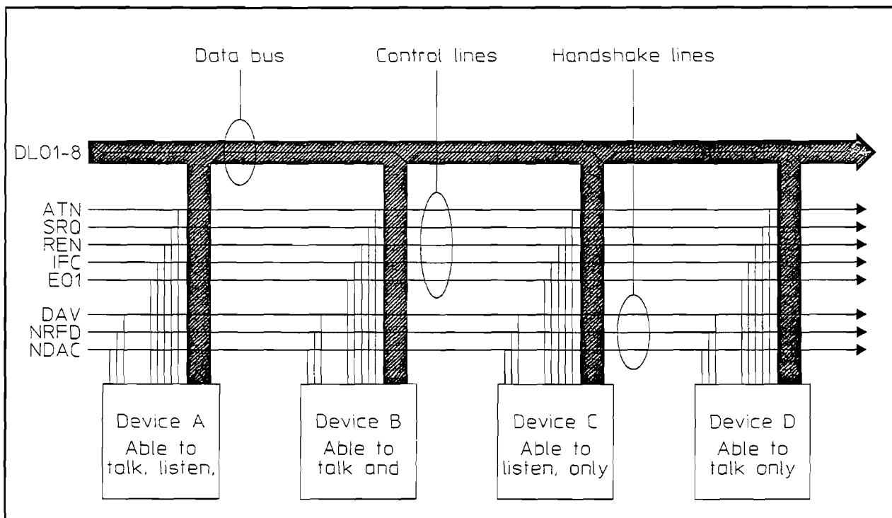
Figure 2-1. HP-IB Structure
