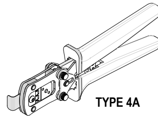
Hand Crimp Tool Order No. 63825-8800
