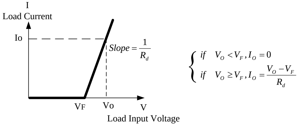
The V-I Fragments Similar to Curve of LED
