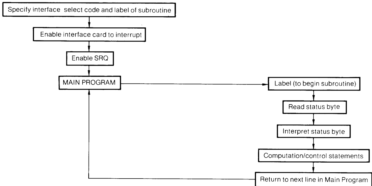
FIGURE 4-5. INTERRUPT SETUP
