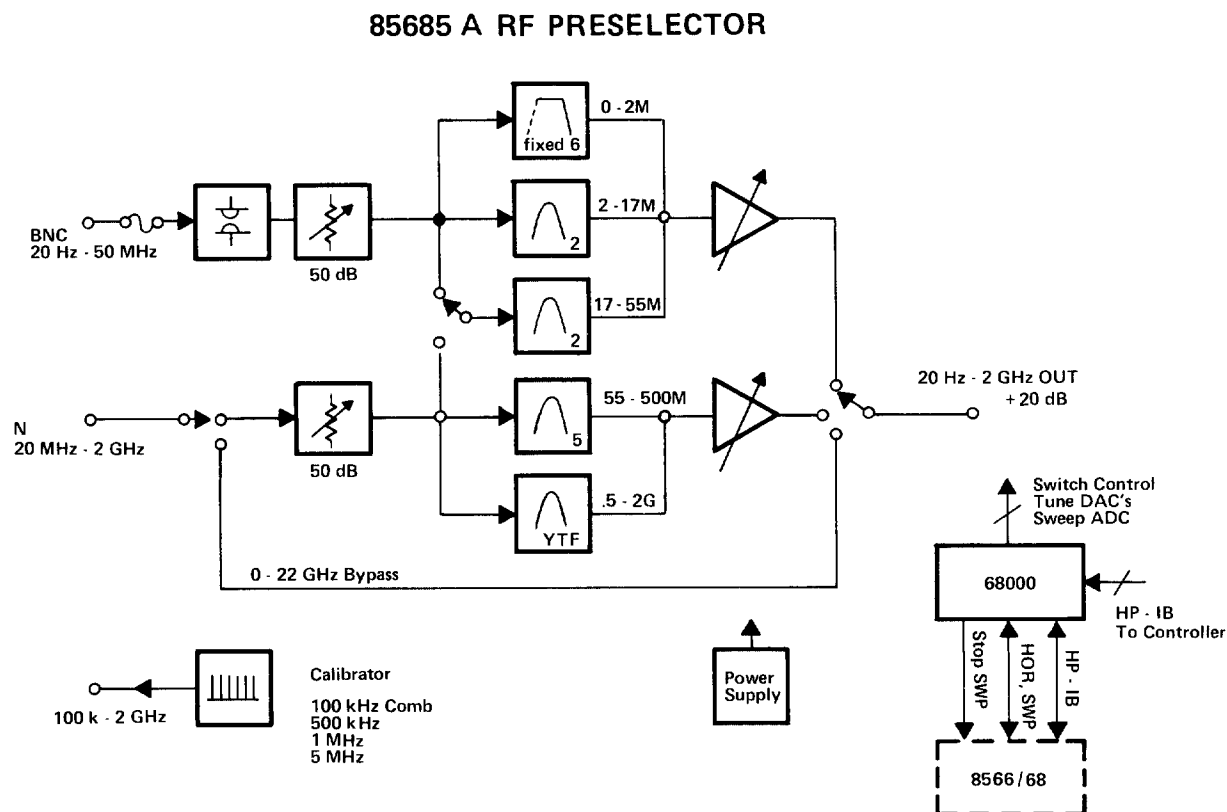
FIGURE 1-3. PRESELECTOR BLOCK DIAGRAM
