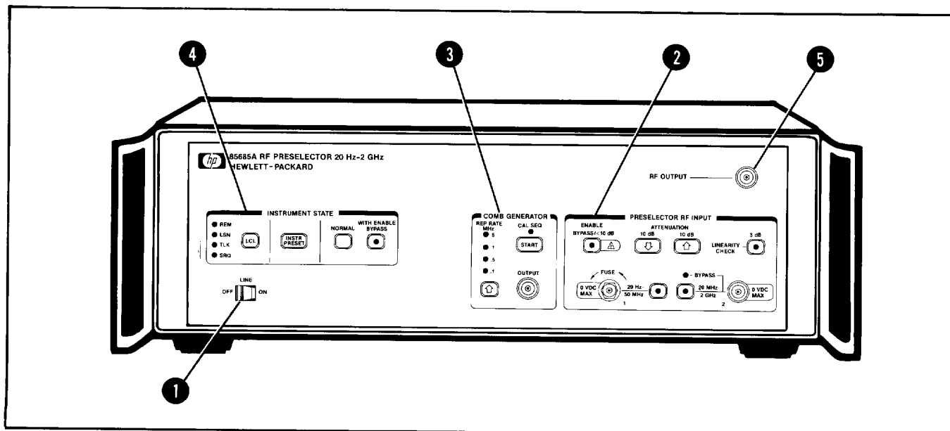
FIGURE 3-3. PRESELECTOR FRONT PANEL
