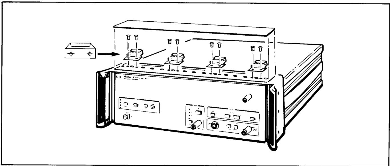
FIGURE 2-2. LOCK-LINK INSTALLATION
