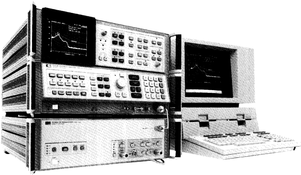
FIGURE 1-1. AUTOMATIC SPECTRUM ANALYZER/TEST RECEIVER
