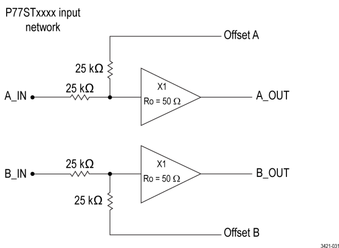
Figure 5: Simplified drawing of input attenuation factor of the P7700 Series buffers
