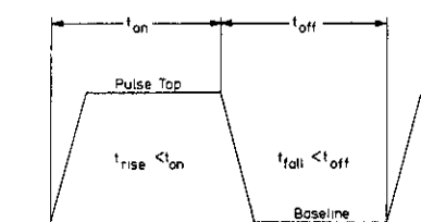
Figure 3-11. Transition Time Limits
