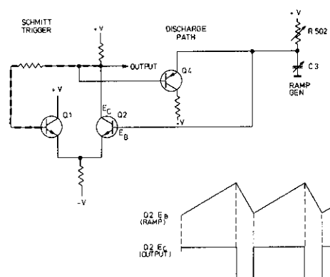
Figure 4-1. Simplified Rep. Rate Generator
