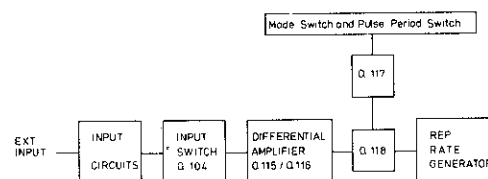
Figure 4–2. Gating Elements
