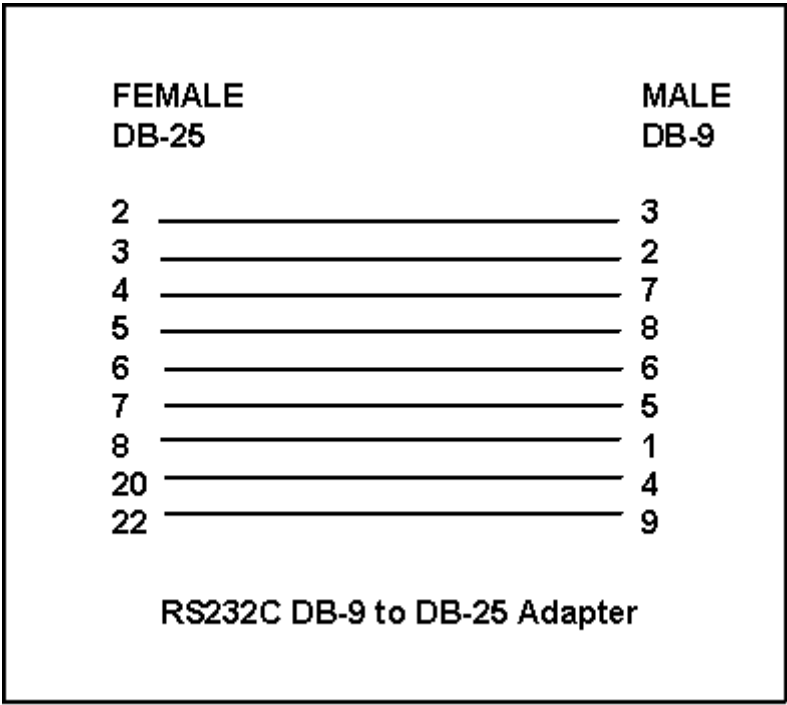
Figure 3-2 : DB9 to DB25 Adaptor Wiring Diagram
