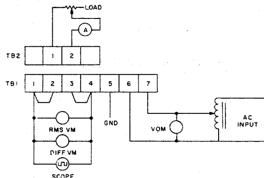
Figure 5-1 Test Equipment Setup
