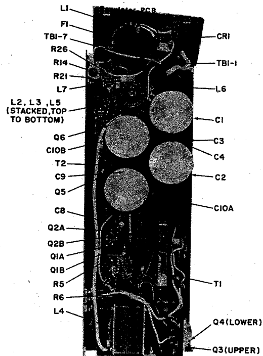
Figure 5-5 Module IIIA-Typical Component Location Photo
