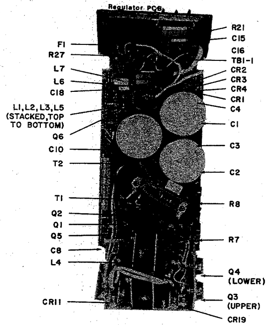
Figure 5-4 Module III-Typical Component Location Photo
