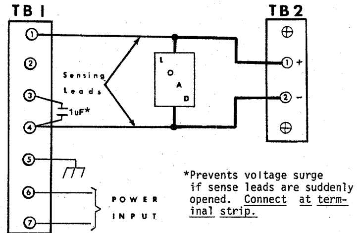
Figure 3-1 Remote Sensing Connections
