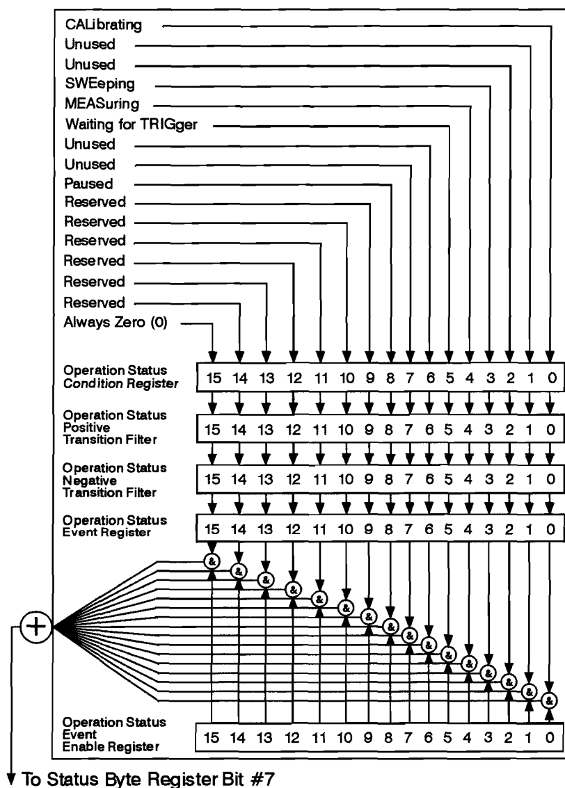
Figure 2-10 STATUS:OPERation Register
