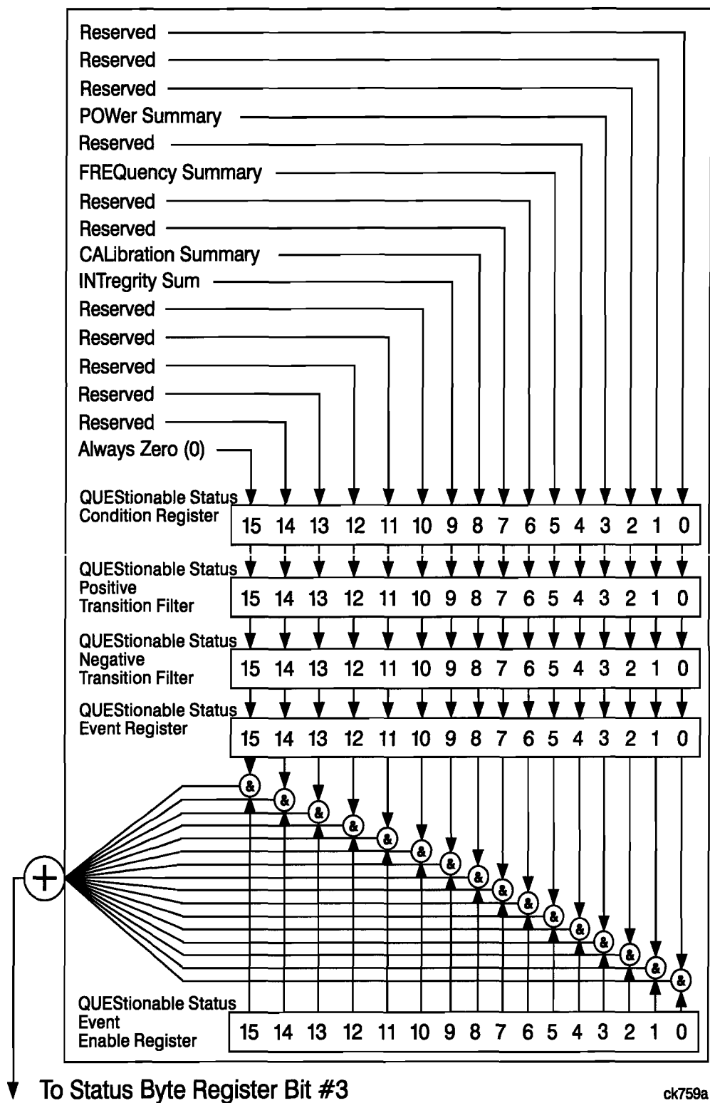
Figure 2-13 STATUS:QUEStionable Register
