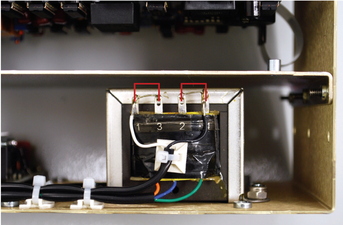
Figure 5. ATRT-01 S2 100 – 120 Vac Jumper Settings
