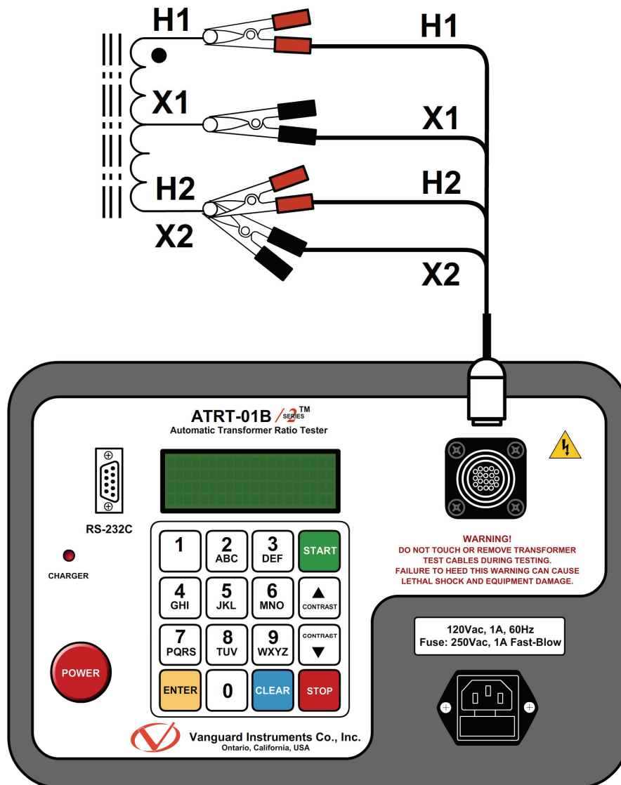
Figure 8. Typical Auto Transformer Connection
