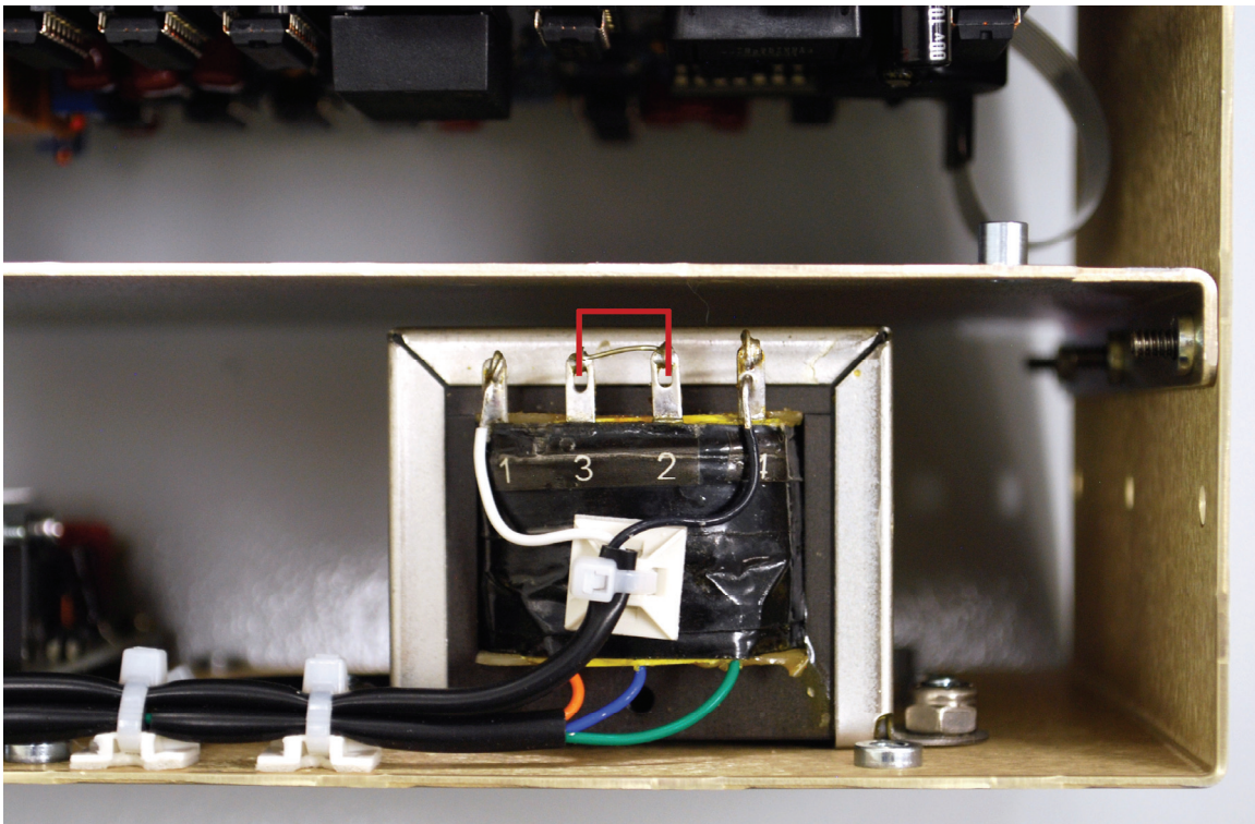
Figure 6. ATRT-01 S2 200 – 240 Vac Jumper Settings
