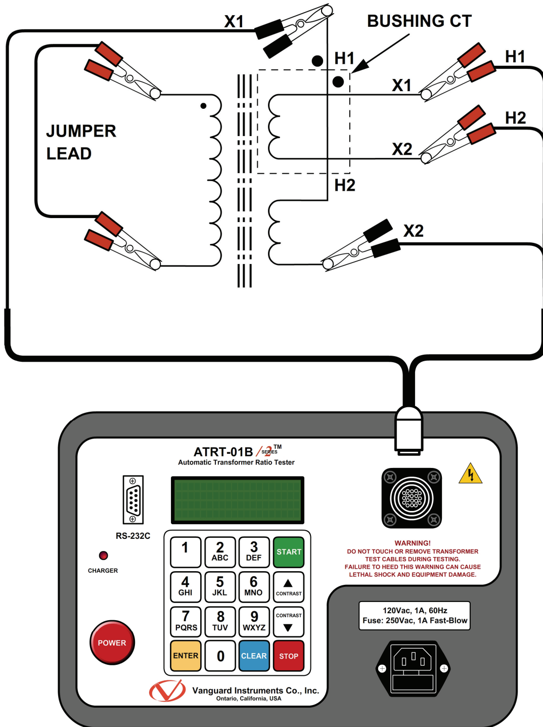
Figure 10. Typical Bushing CT Connection on a Single Transformer
