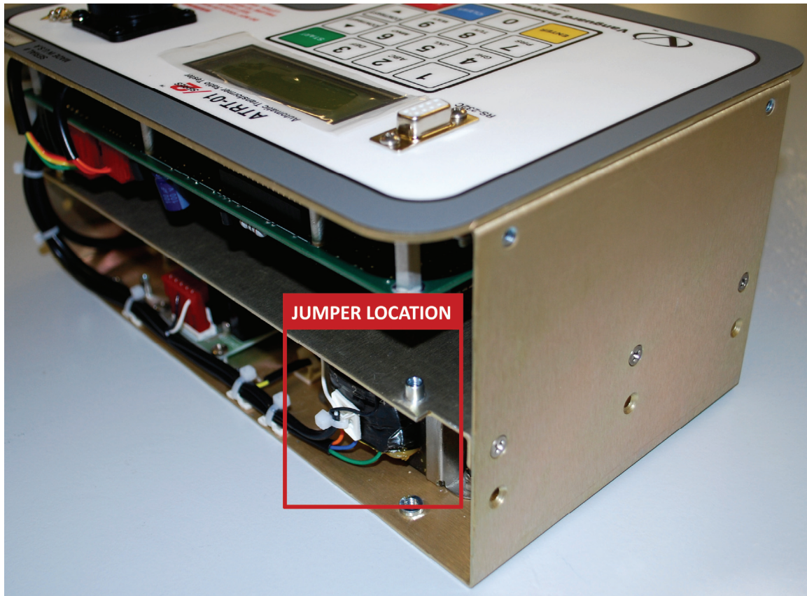
Figure 4. ATRT-01 S2 Voltage Selection Jumper Location
