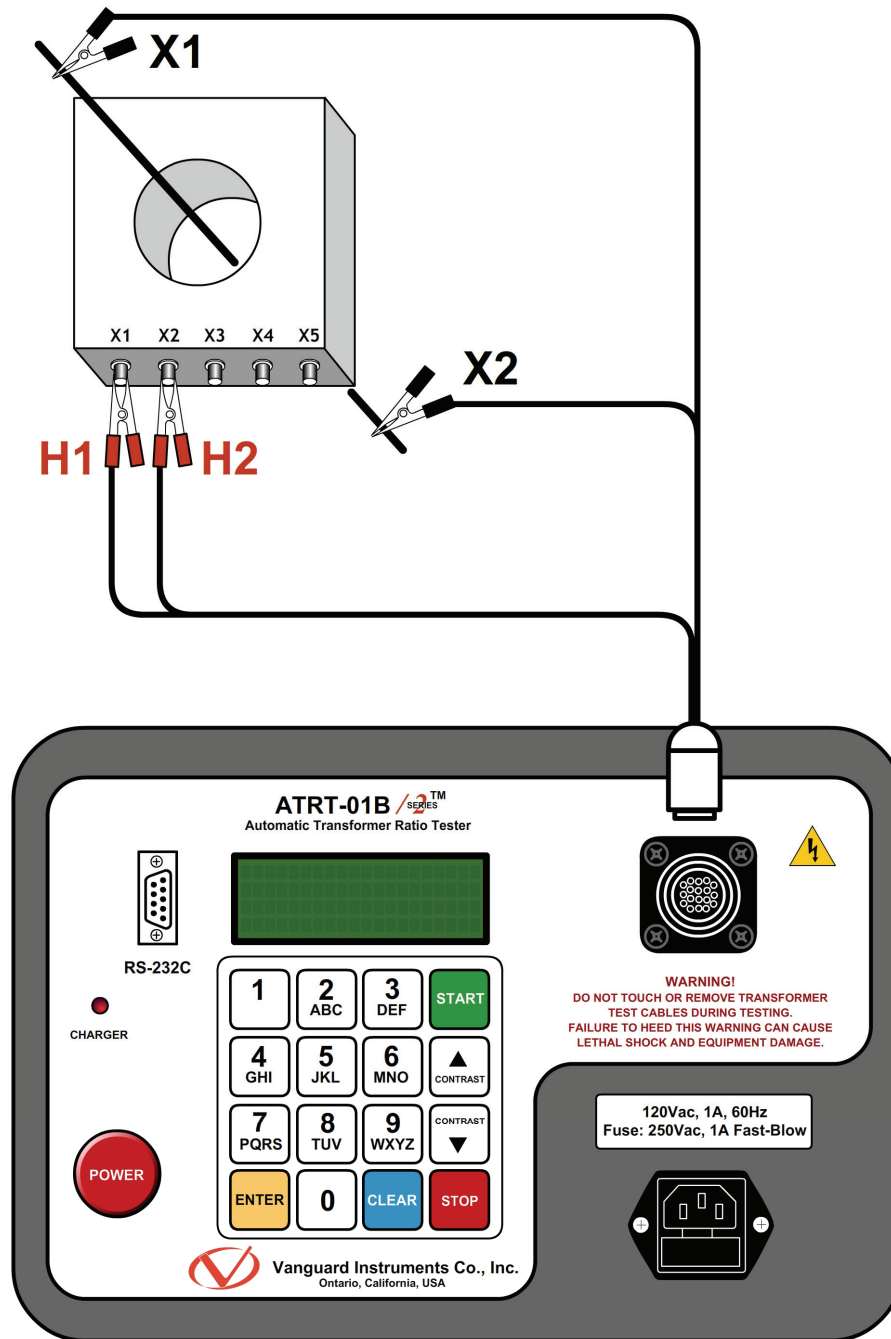
Figure 9. Typical CT Connection
