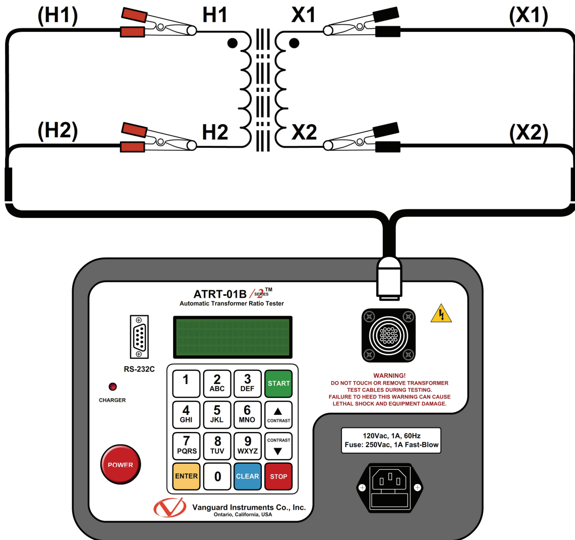
Figure 7. Typical Single-Phase Transformer Connection
