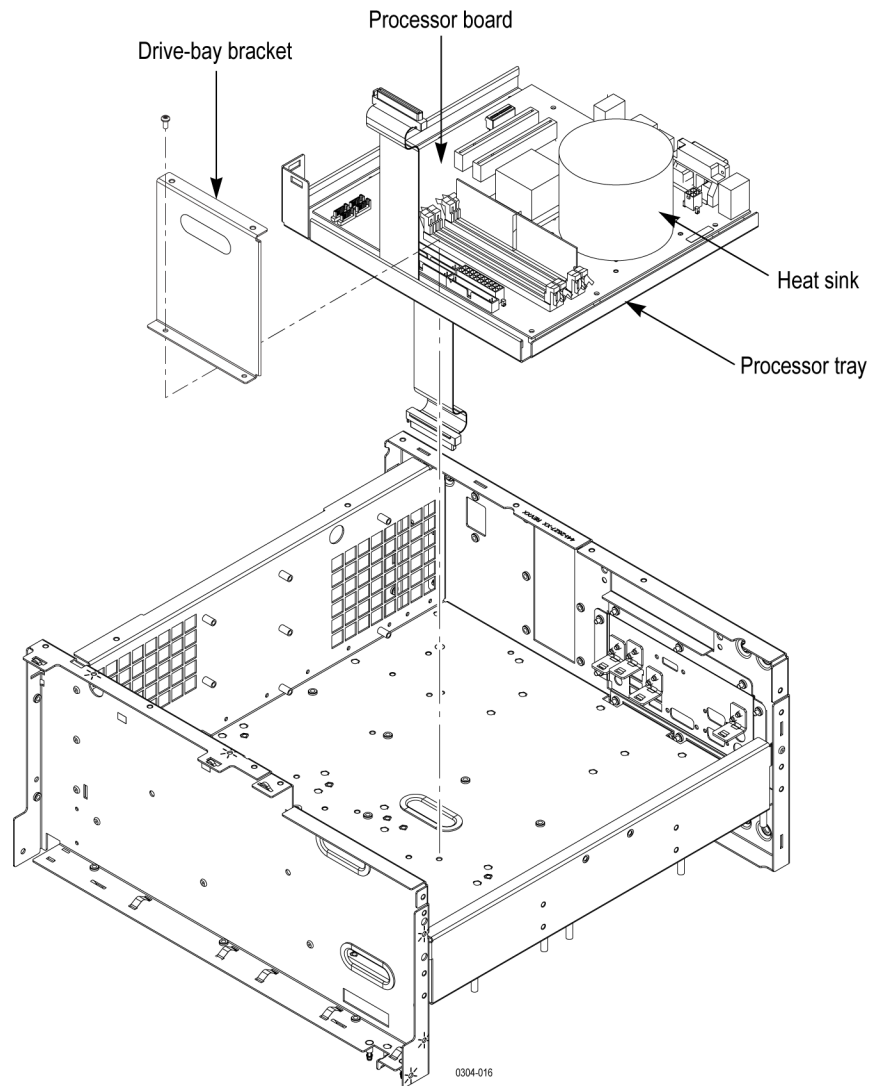
Figure 4-11: Processor module removal (AWG7000C Series)
