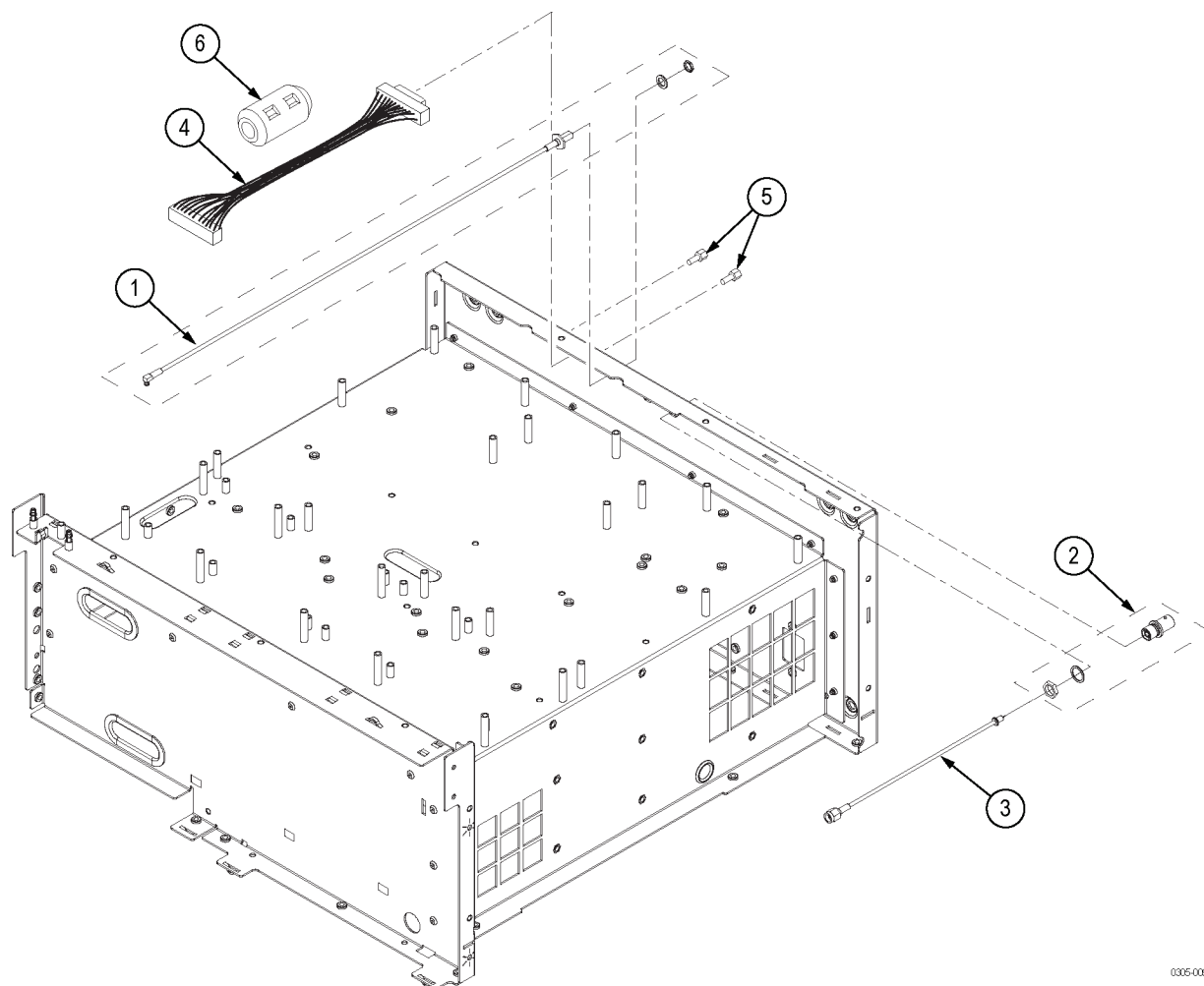
Figure 5-22: Rear connectors
