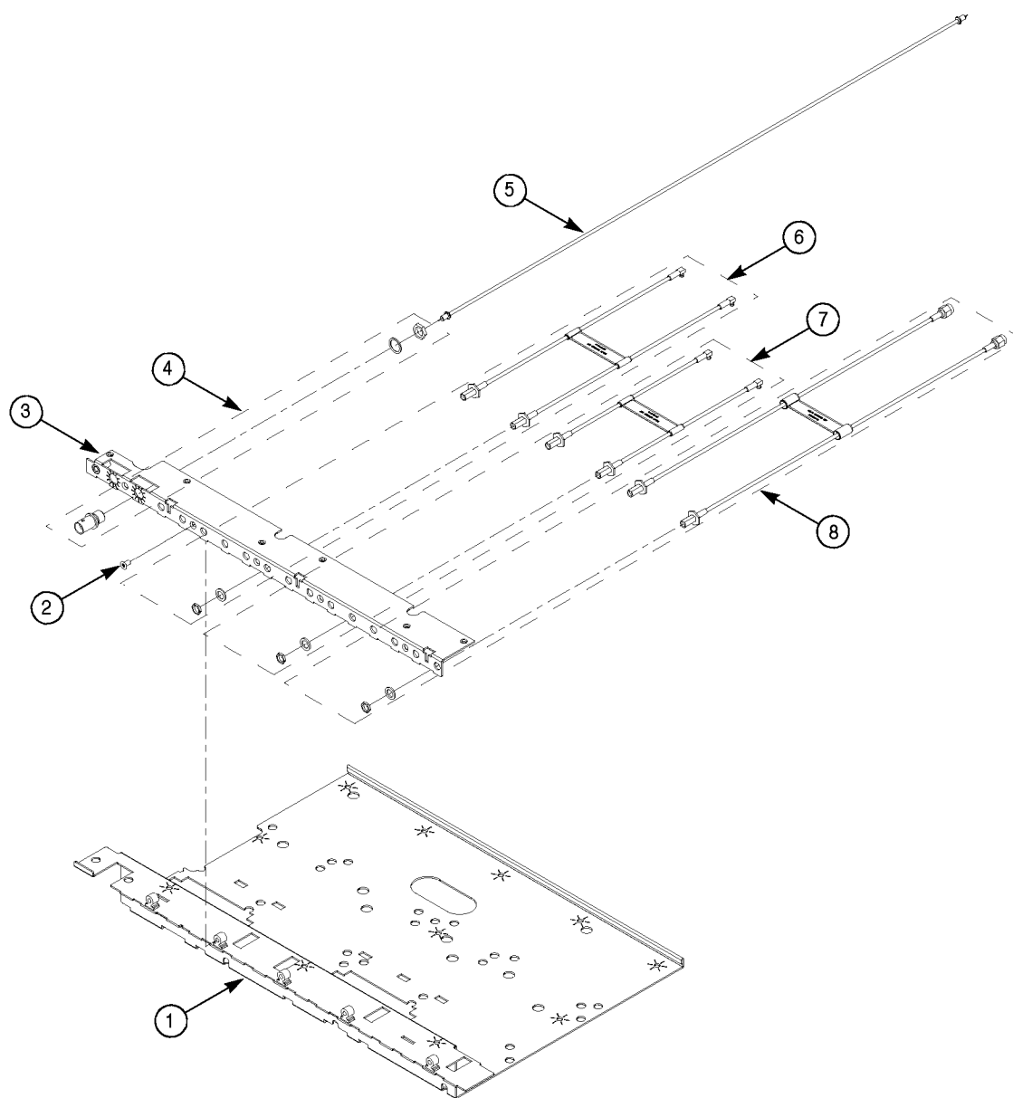
Figure 5-20: SMA bracket
