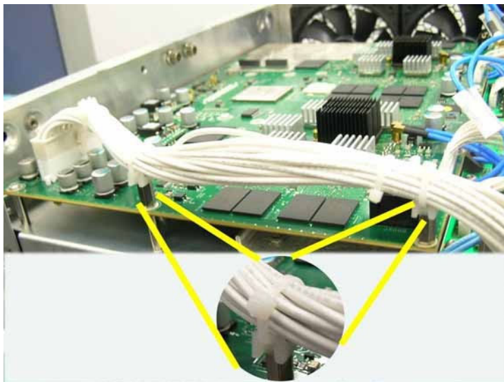
Figure 4-23: Cable ties
