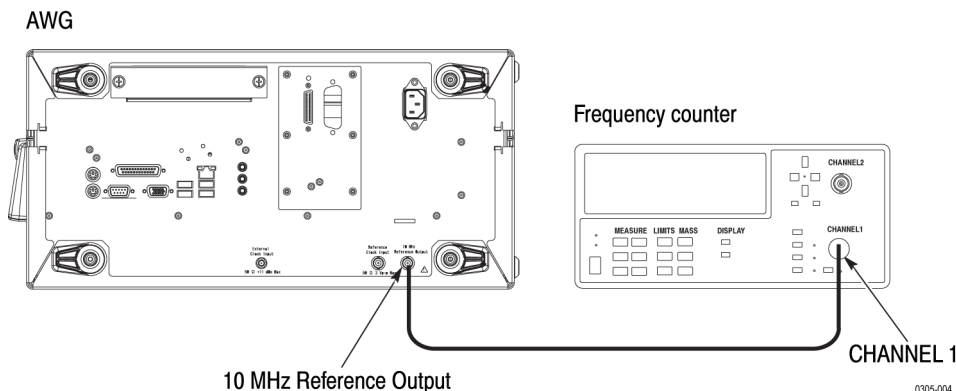
Figure 3-2: 10 MHz Reference calibration initial test hookup
