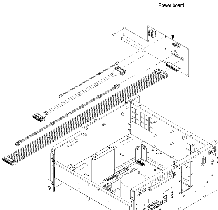
Figure 4-18: Power board removal (AWG7000B Series)
