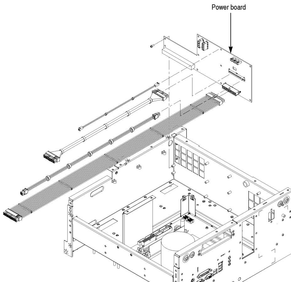
Figure 4-13: Power board removal (AWG7000C Series)
