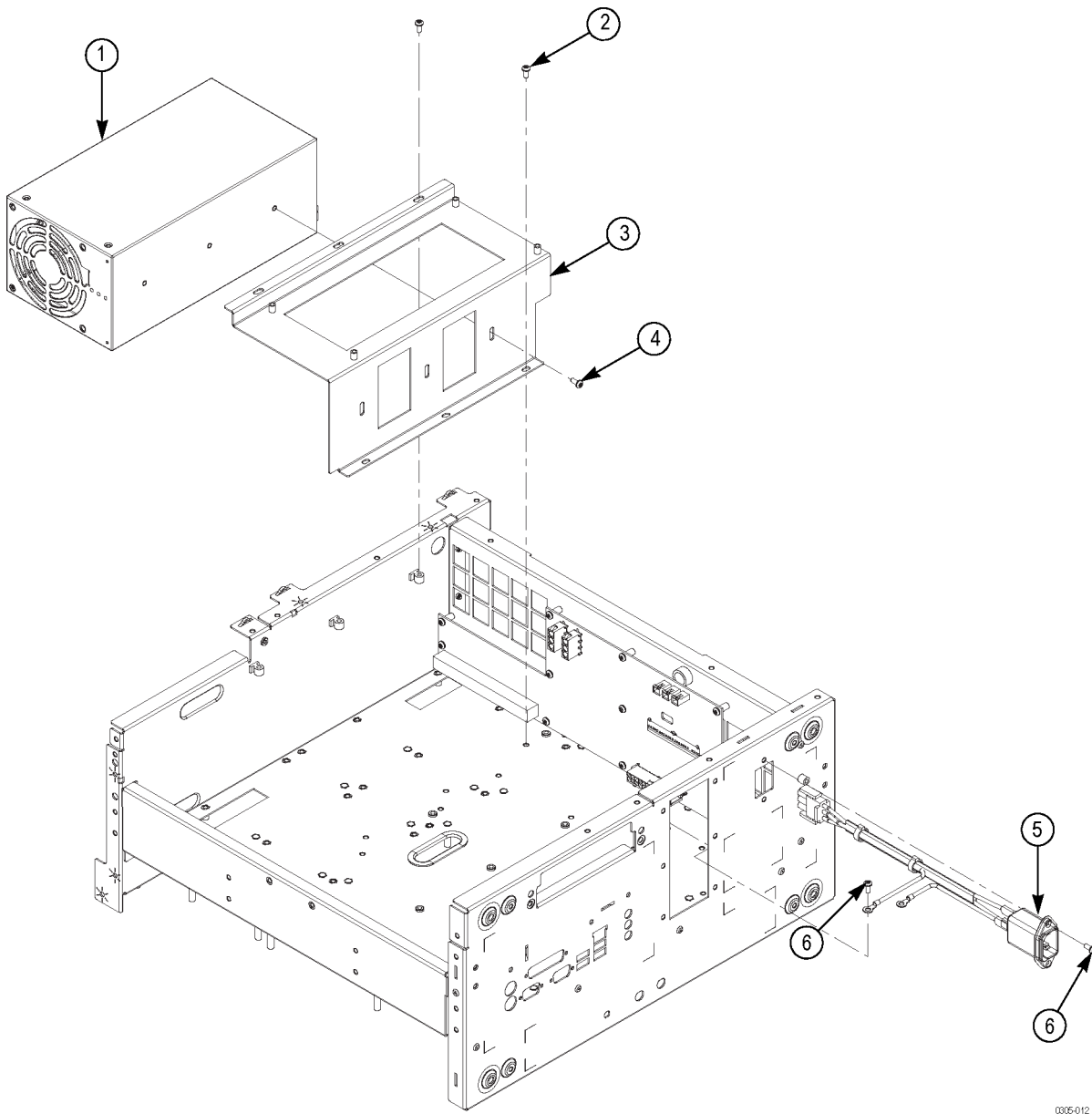
Figure 5-11: AWG7000C Series power supply assembly
