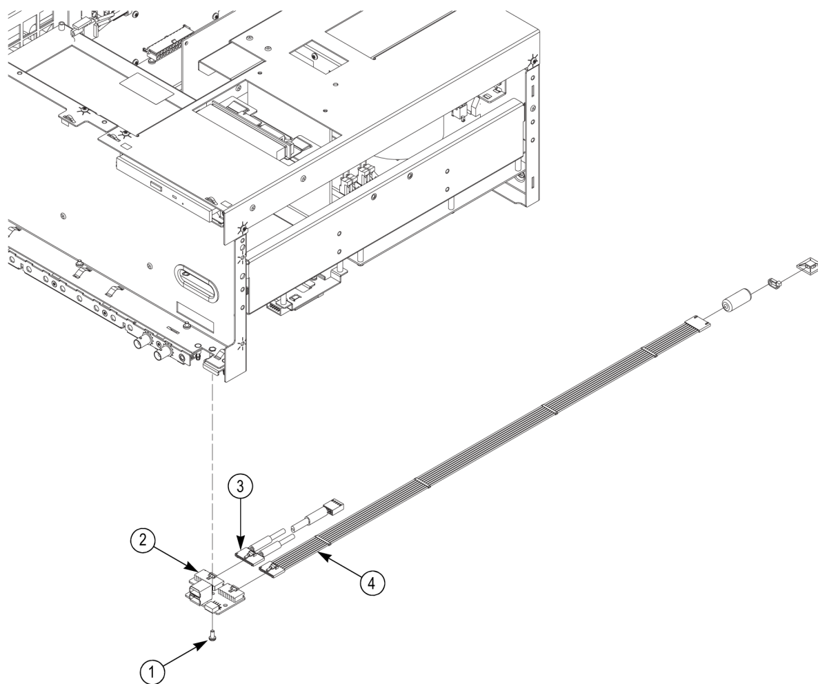
Figure 5-16: USB module
