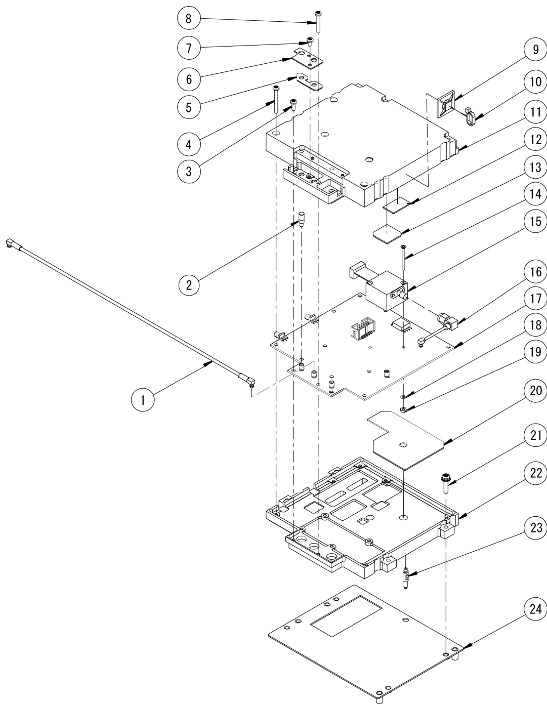
Figure 5-18: CLK12G module
