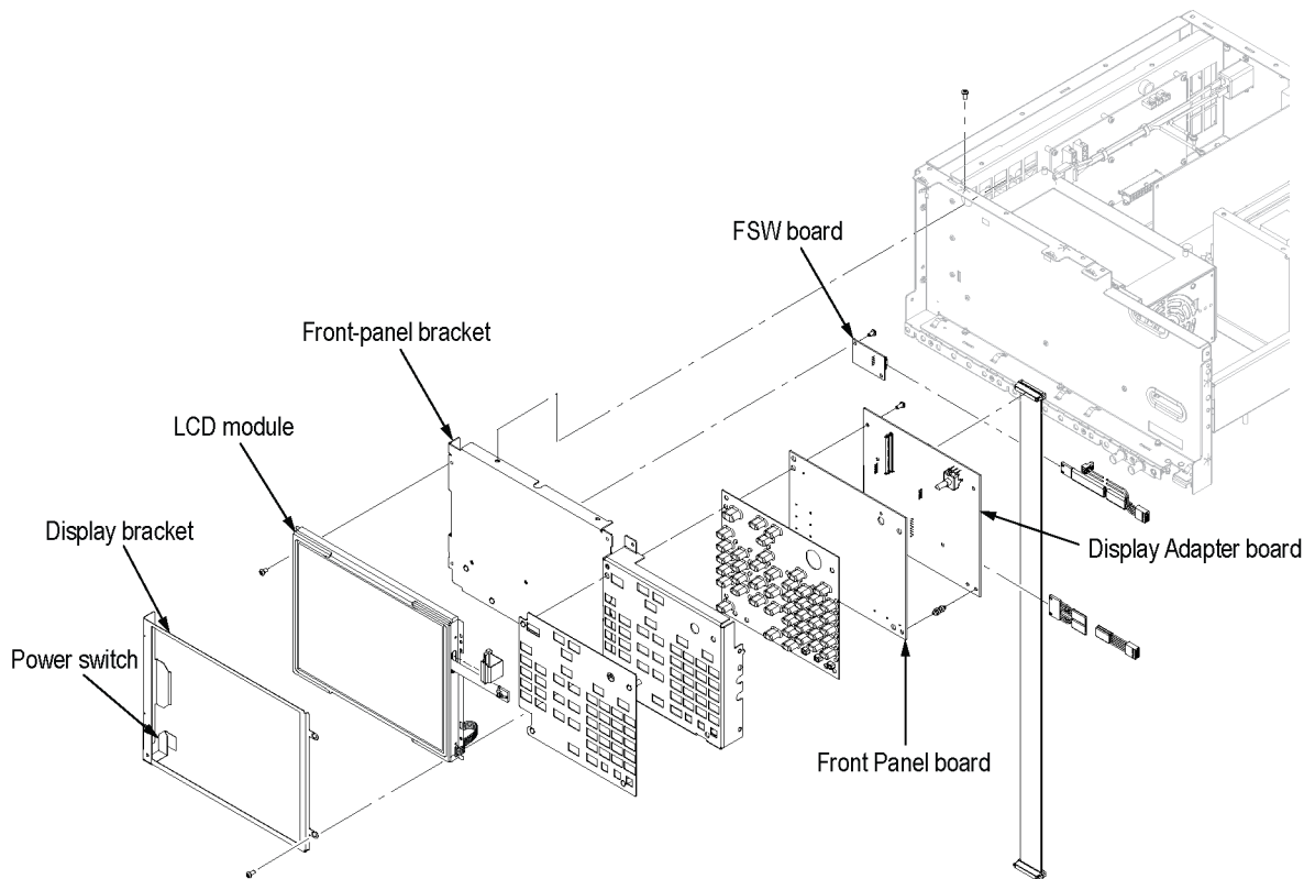
Figure 4-7: Disassembly of front-panel assembly (AWG7000C Series)
