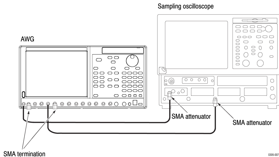
Figure 3-6: Interleave calibration initial hookup
