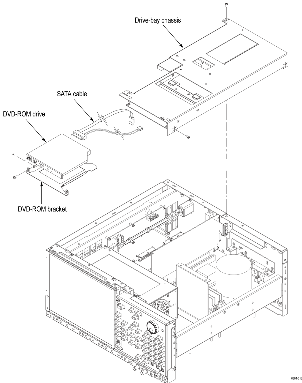
Figure 4-9: Drive module removal (AWG7000C Series)
