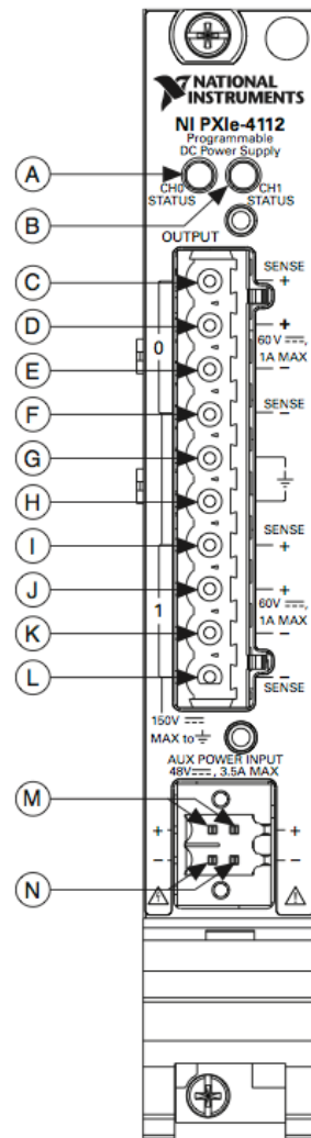
Figure 3. NI PXle-4112 Front Panel
