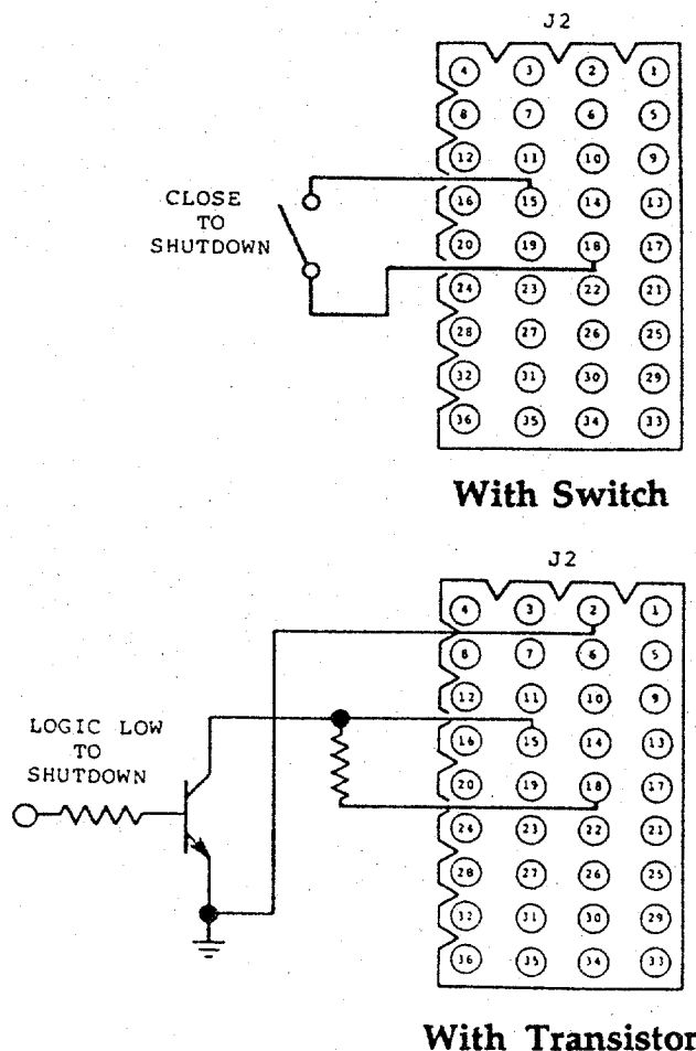
Figure 3.11 Remote Shutdown
