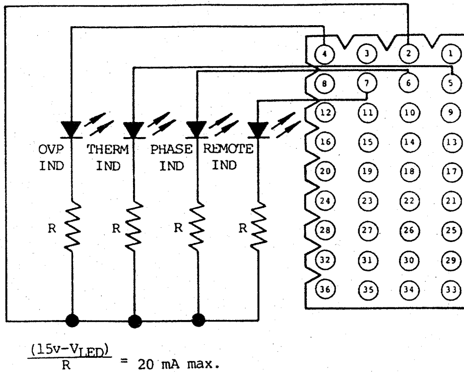
With Remote Led Indicators
