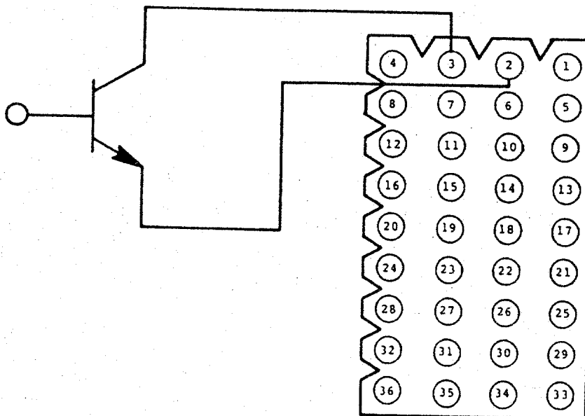
With Transistor Switch
