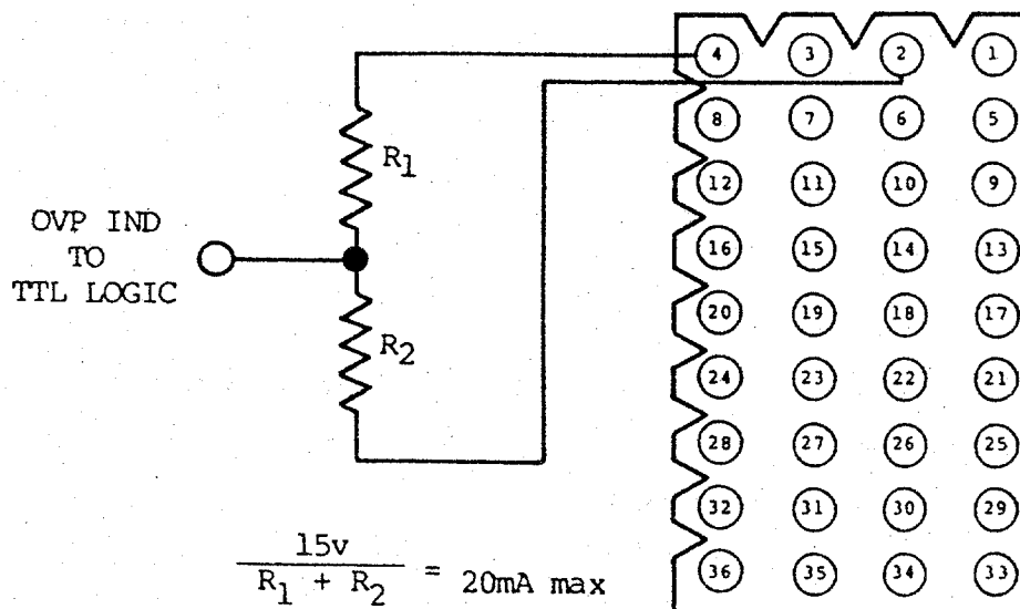
Interface to TTL
