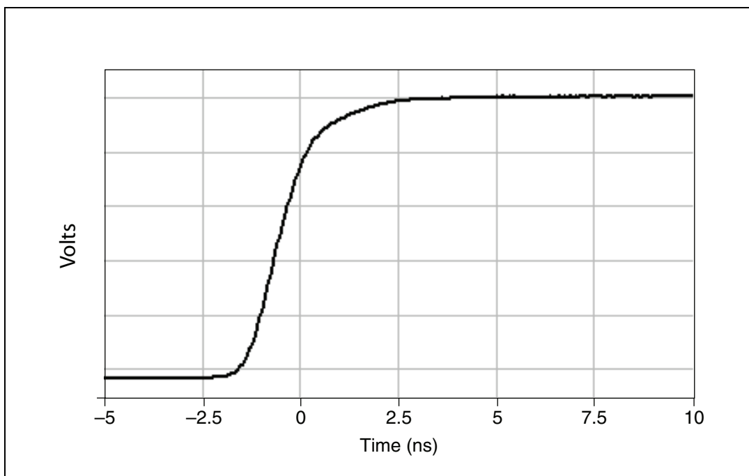
Figure 4. NI 5152 Step Response, 50 \Omega , 0.1 V pk=pk Range, Typical
