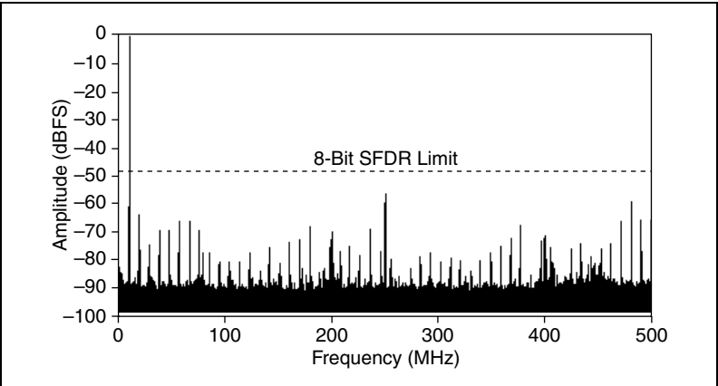
Figure 5. NI 5152 Dynamic Performance, 50 Ω, 1 V pk=pk Range, 9.425 MHz, –1 dBFS Input Signal, Typical
