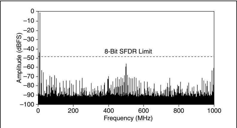
Figure 6. NI 5152 TIS Dynamic Performance, 50 Ω, 1 V pk=pk Range, 9.425 MHz, –1 dBFS Input Signal, Typical
