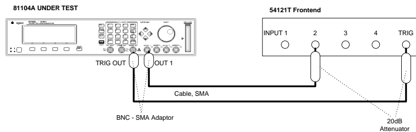
Connecting Agilent 81104A to the Scope
