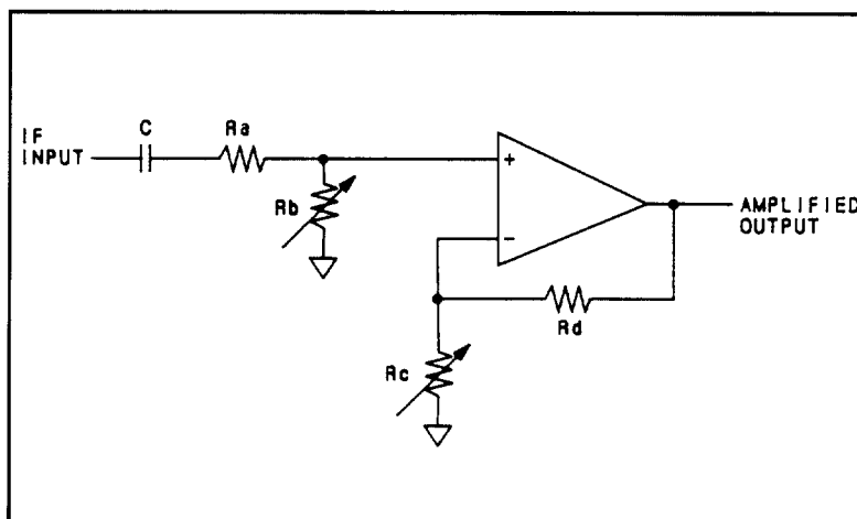
Figure 8F-10. Simplified Diagram of the Current-Variable Amplifier
