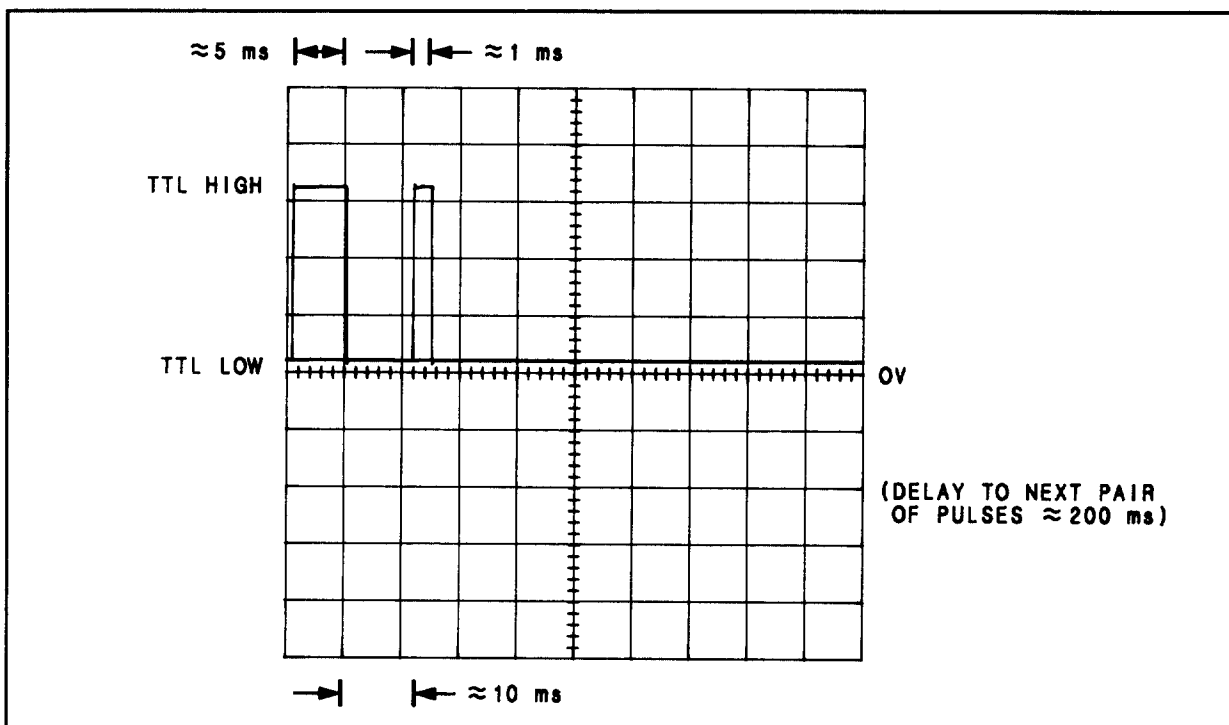
Figure 8F-23. Waveform for \langle \sqrt{2} \rangle Step 4
