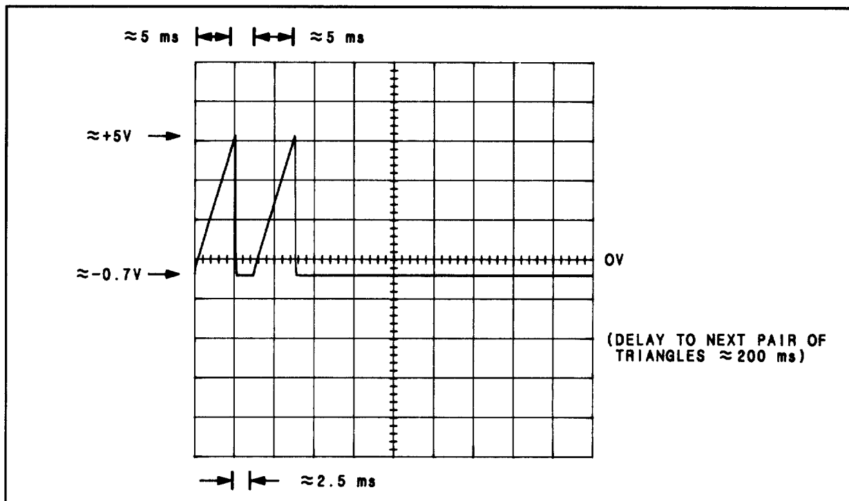
Figure 8F-22. Waveform for \langle \sqrt{2} \rangle Step 3
