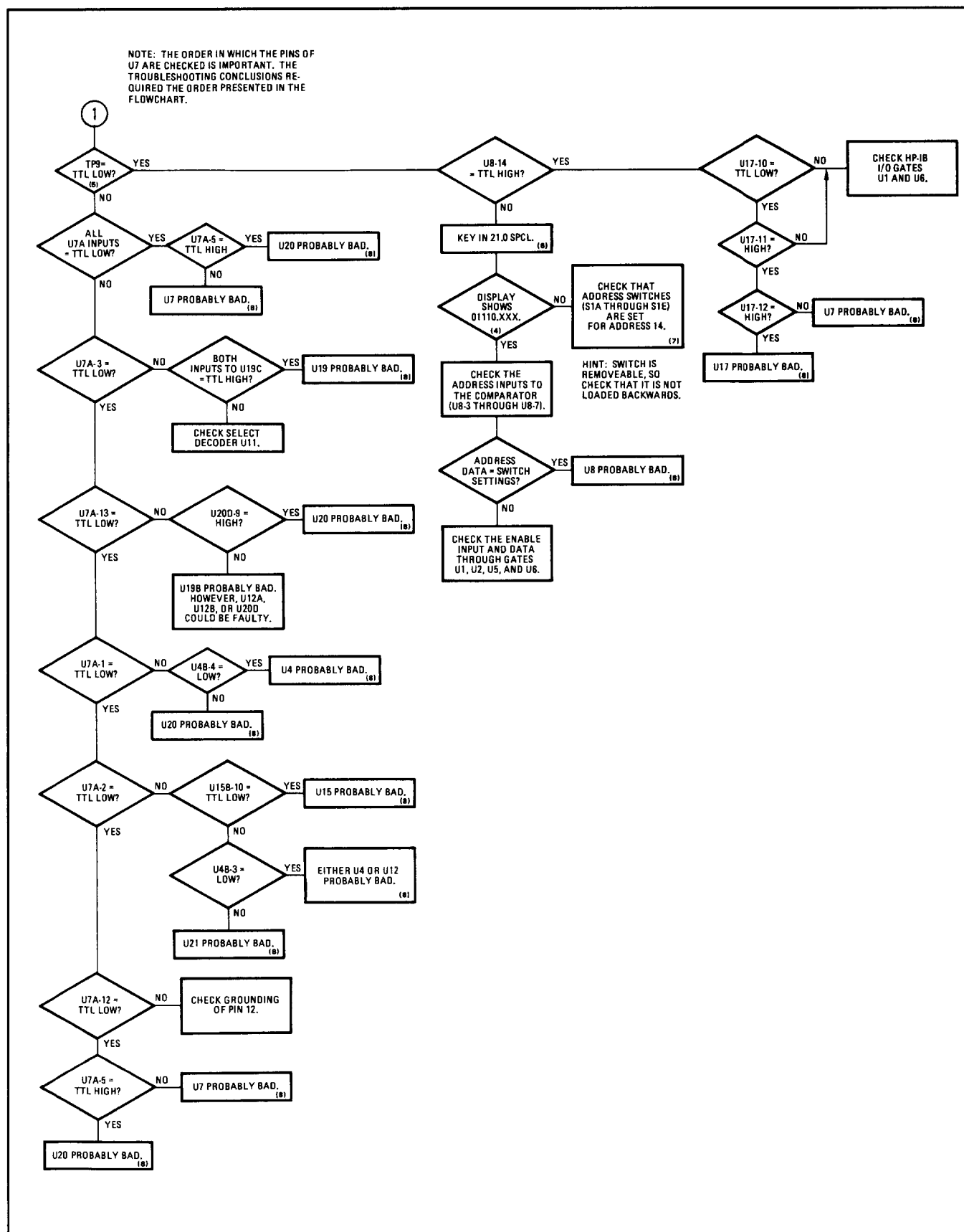
Figure 8F-35. Address Recognition Check Troubleshooting Flowchart, (2 of 2)
