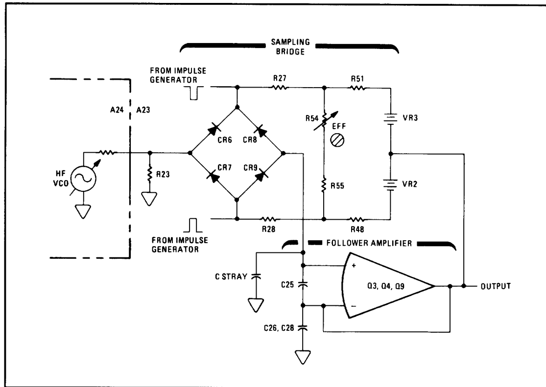
Figure 8F-26. Simplified Schematic of Sampler Amplifier
