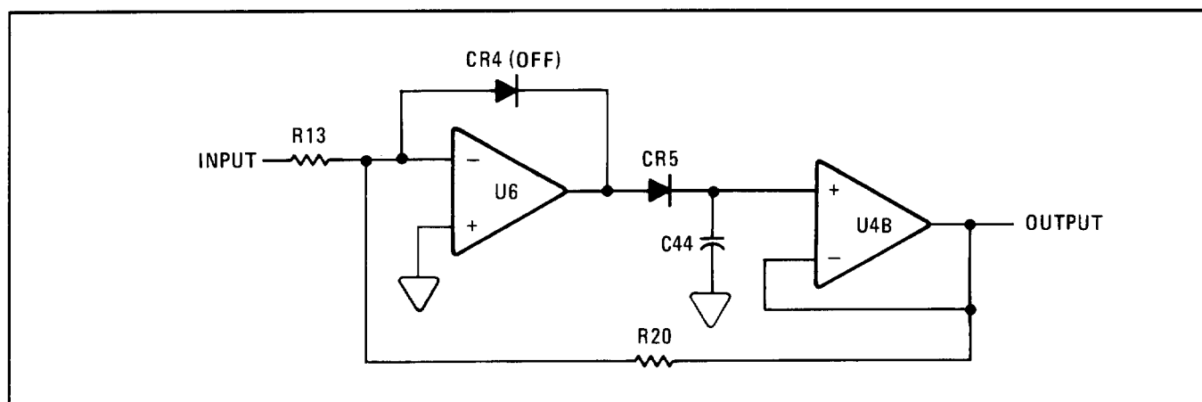
Figure 8F-16. The Absolute Peak Detector Shown as an Inverting, Negative-Peak Detector
