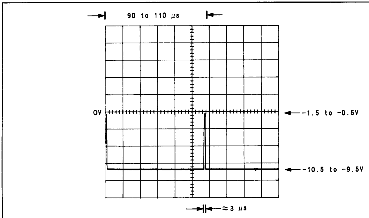
Figure 8F-39. Waveform for \sqrt{1} Step 4 (U5A pins 4 and 6)
