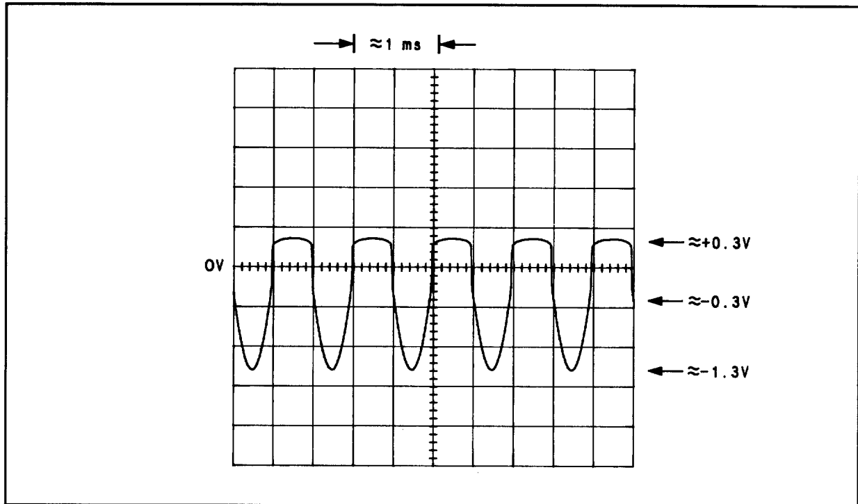
Figure 8F-21. Waveform for \sqrt{3} Step 4
