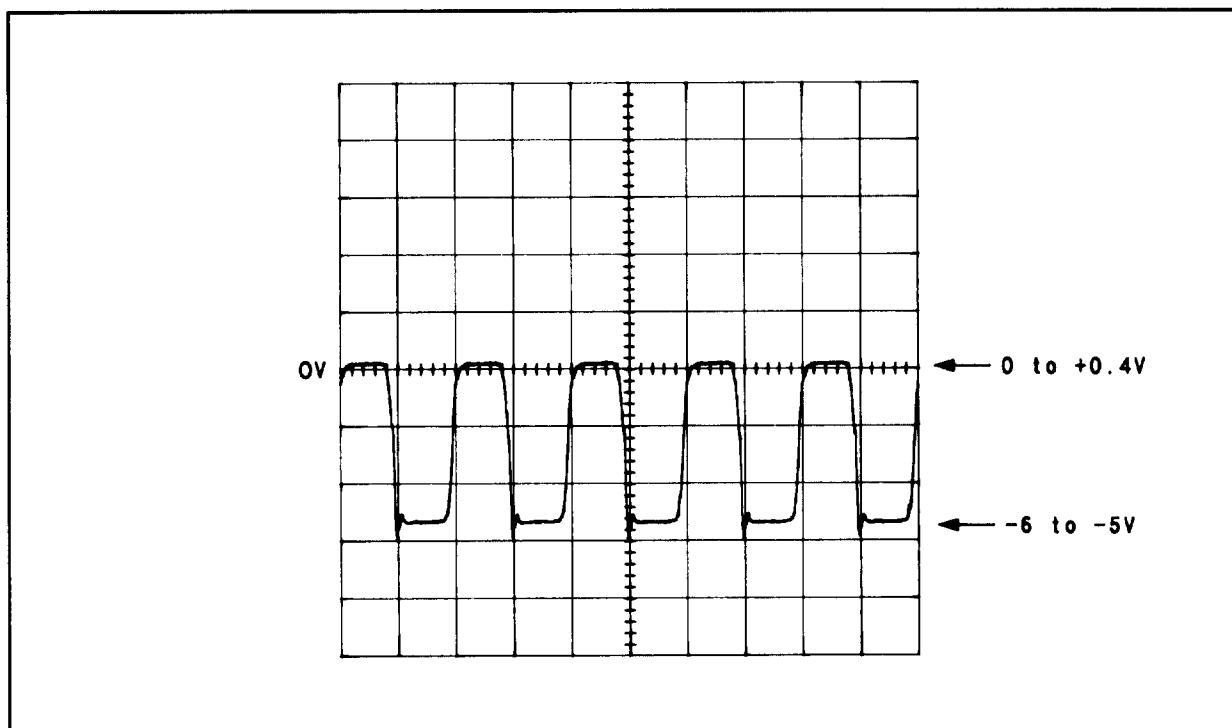
Figure 8F-29. Waveform for \sqrt{4} Step 3
