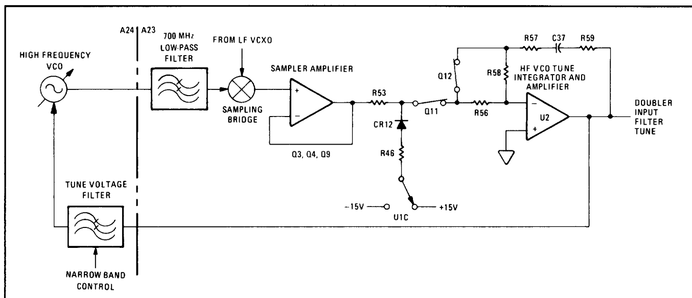
Figure 8F-28. Simplified Schematic of LO Configuration: DAC to LF VCXO (DAC Connection Not Shown)
