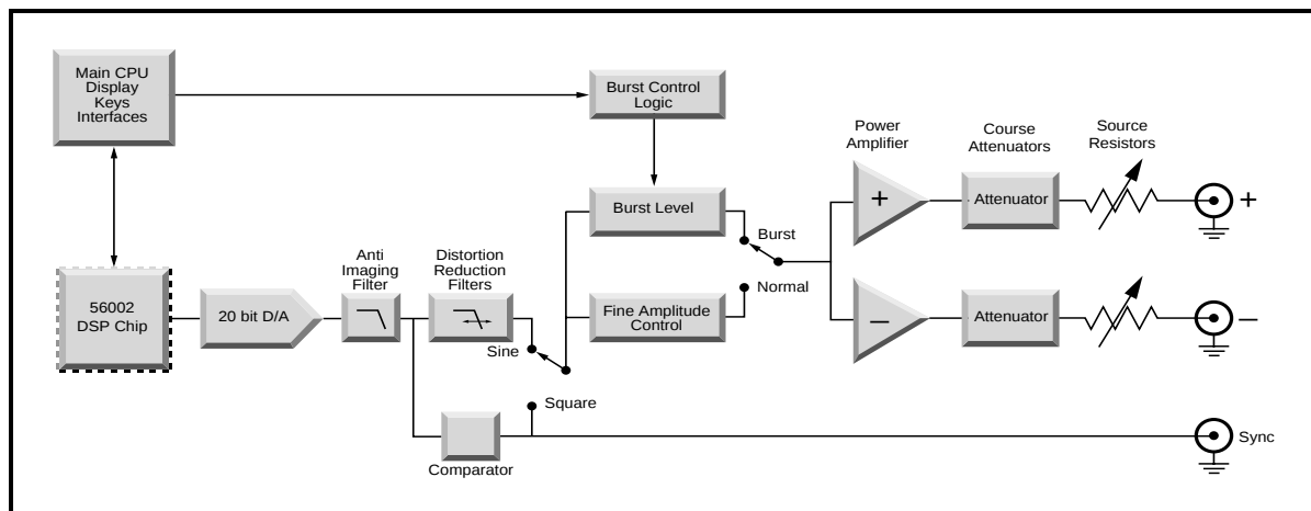
Figure 2-1 DS360 Block Diagram
