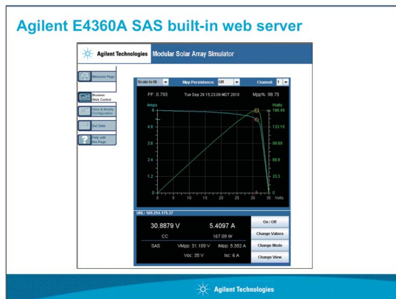
Figure 4: Agilent E4360A built-in web server
