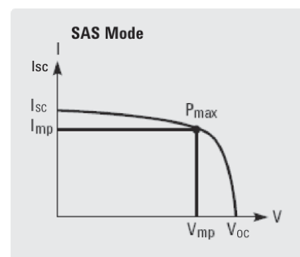
Figure 1: Power supply output characteristic in SAS mode
