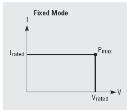
Figure 2: Power supply output characteristic in Fixed mode
