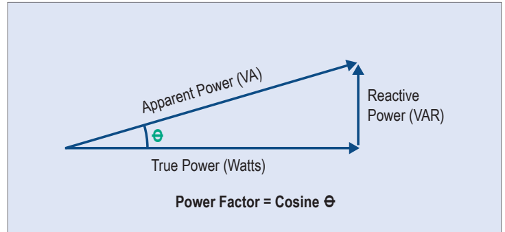
Figure 2 - The Power Triangle.
