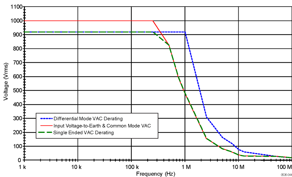
Figure 6: P5200A and P5205A voltage derating curves
