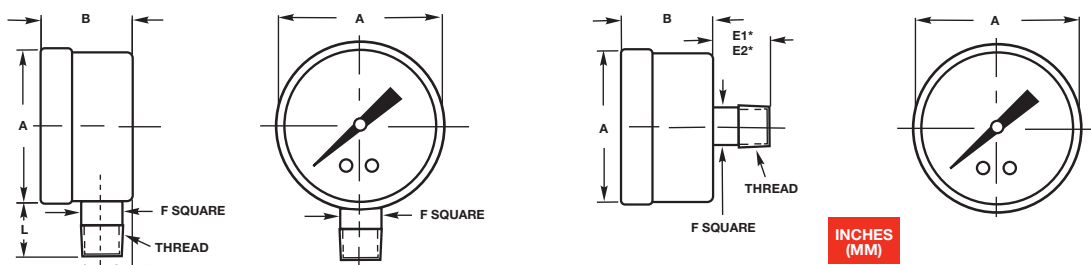
Model P-500 Center-Back Mount (left) and Lower Mount
