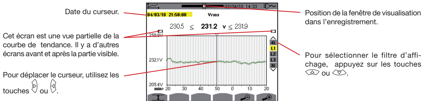
Figure 104 : Vrms (L1) sans MIN-AVG-MAX
