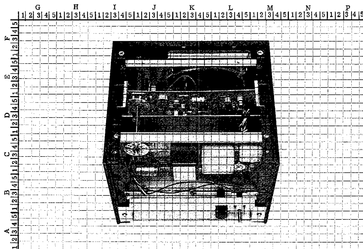
Figure 5-1. FINAL ASSEMBLY
