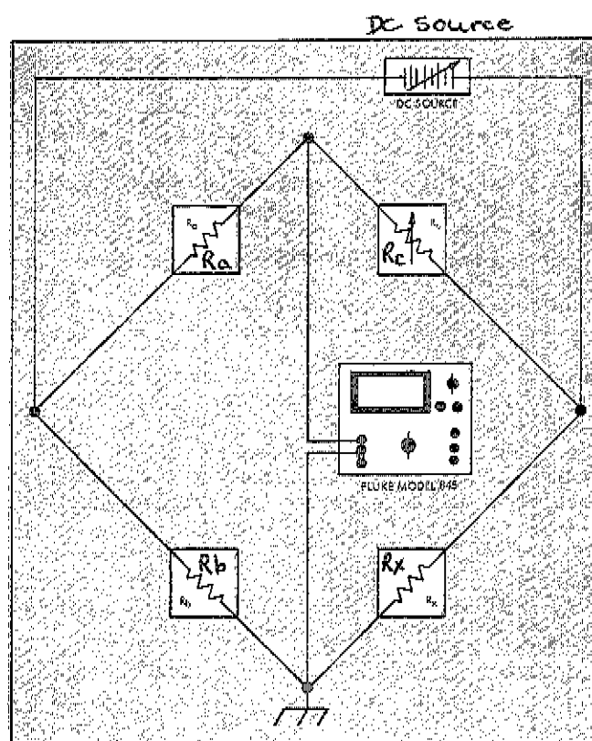
Figure 2-2. BRIDGE DETECTOR-FLOATING SUPPLY
