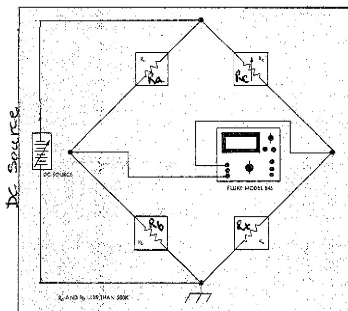
Figure 2-4. BRIDGE DETECTOR-FLOATING NULL DETECTOR
