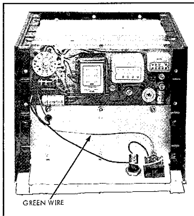
Figure 2-6. CHASSIS GROUND-WIRE LOCATION
