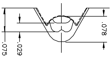
GAGING DIMENSIONS SCALE 10X
