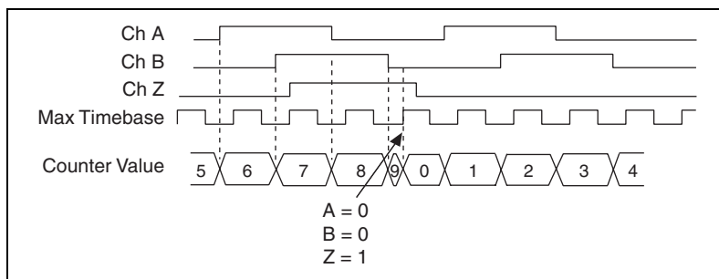
Figure 7-17. Channel Z Reload with X4 Decoding
