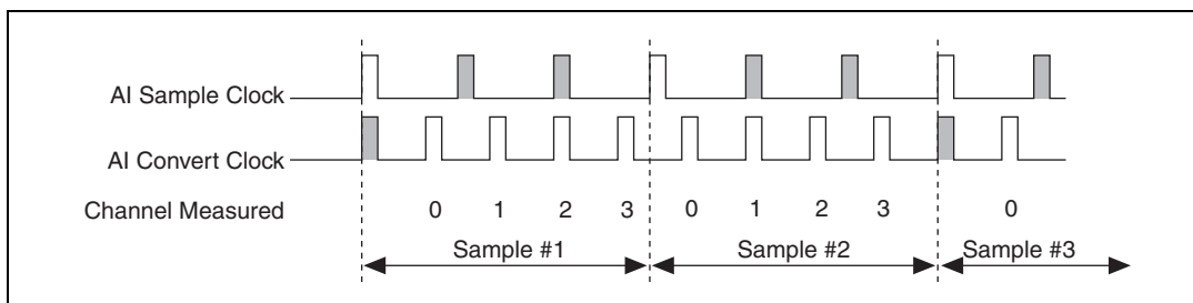
Figure 4-20. AI Sample Clock and AI Convert Clock Improperly Matched; Leads to Aperiodic Sampling
