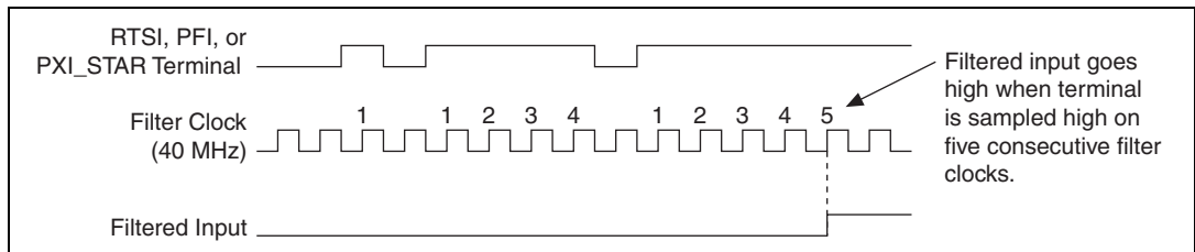
Figure 7-30. Filter Example
