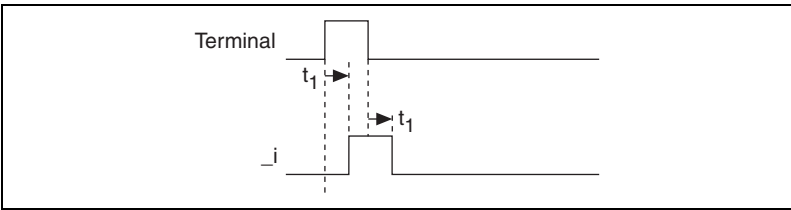
Figure B-3. Input Timing Diagram
