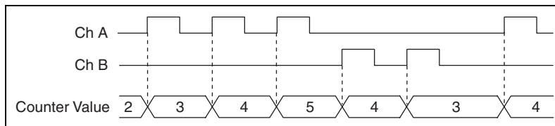
Figure 7-18. Measurements Using Two Pulse Encoders
