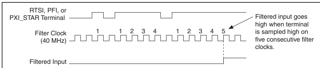
Figure 9-3. Filter Example
