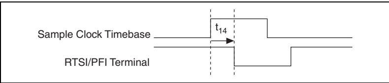
Figure B-36. Sample Clock Delay Timing Diagram
