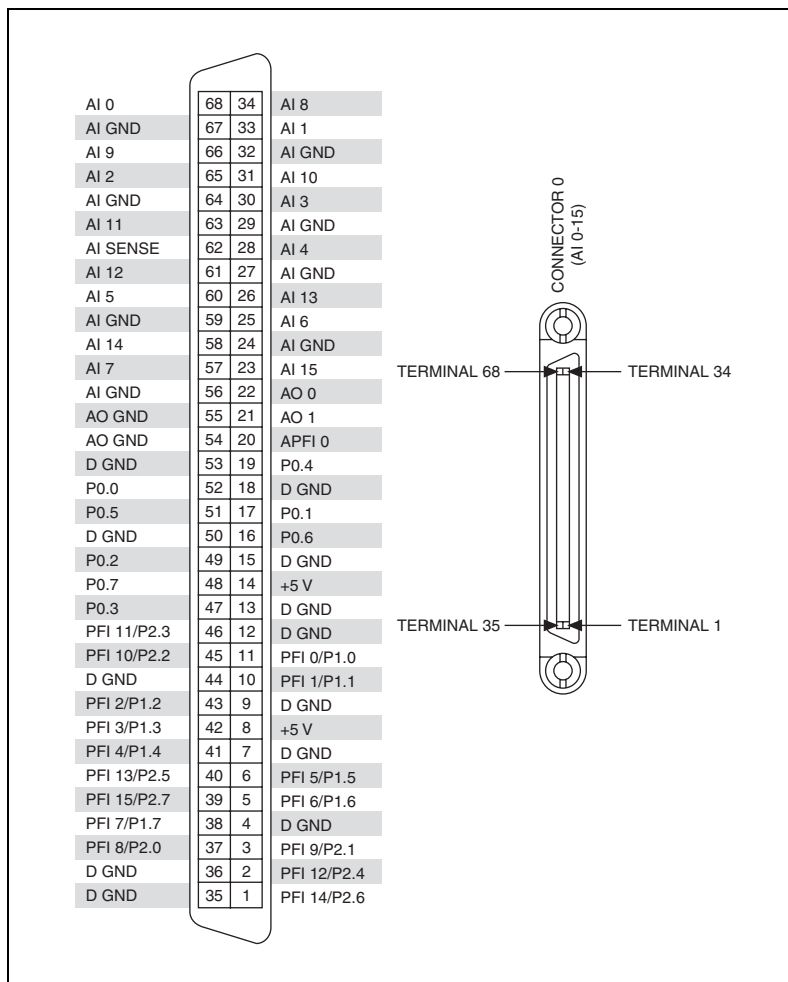
Figure A-57. PCI/PXI-6281 Pinout
