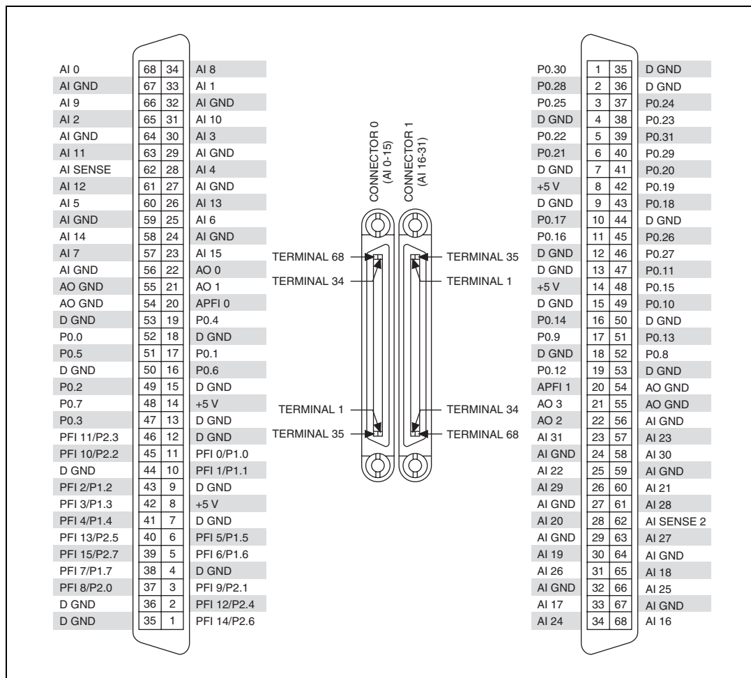
Figure A-44. NI PCI/PCIe/PXI/PXle-6259 Pinout
