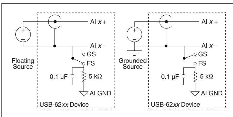
Figure A-48. Analog Input Circuitry
