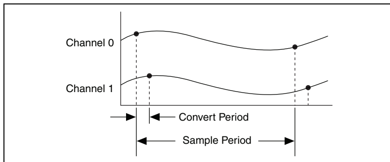
Figure 4-13. Interval Sampling
