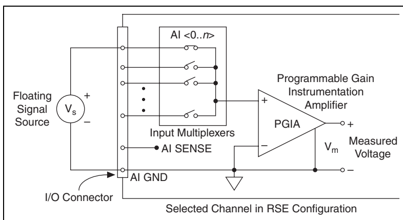
Figure 4-9. RSE Connections for Floating Signal Sources
