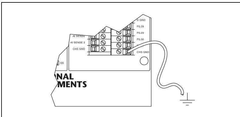
Figure 3-3. Grounding a USB-62xx BNC Device through the CHS GND Screw Terminal
