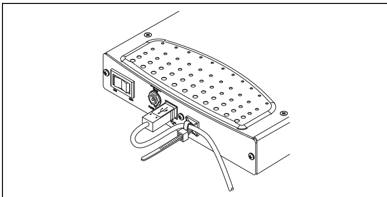
Figure 1-2. USB Cable Strain Relief on USB-62xx Screw Terminal and USB-62xx Mass Termination Devices
