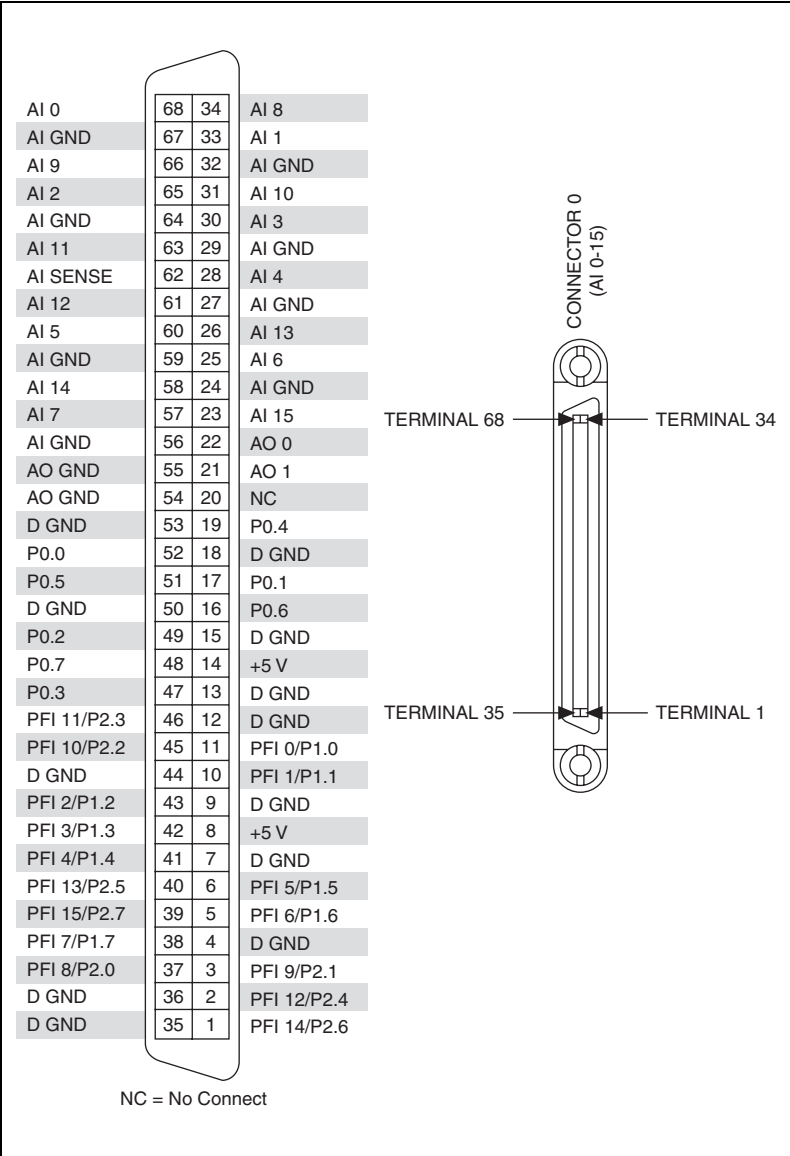
Figure A-2. PCI/PXI-6221 (68-Pin) Pinout
