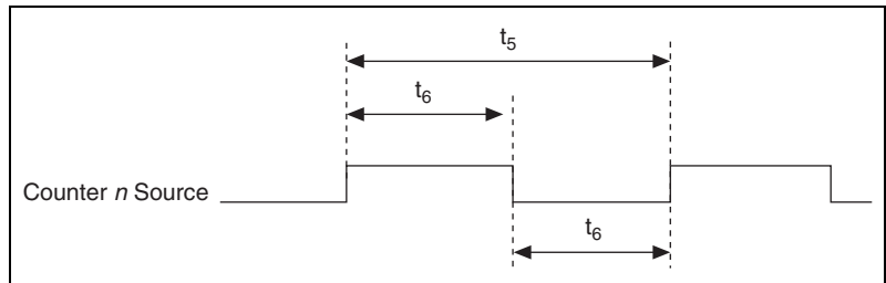
Figure B-46. Counter n Source Timing Requirements
