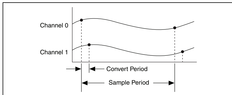
Figure C-1. AI Sample Clock and AI Convert Clock
