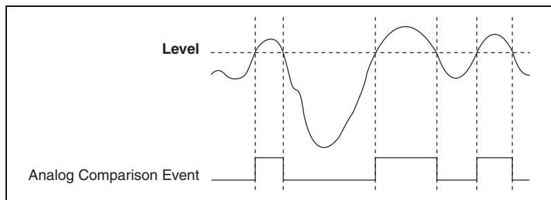
Figure 11-4. Above-Level Analog Triggering Mode
