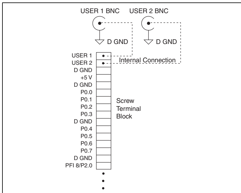
Figure A-11. USER 1 and USER 2 BNC Connections
