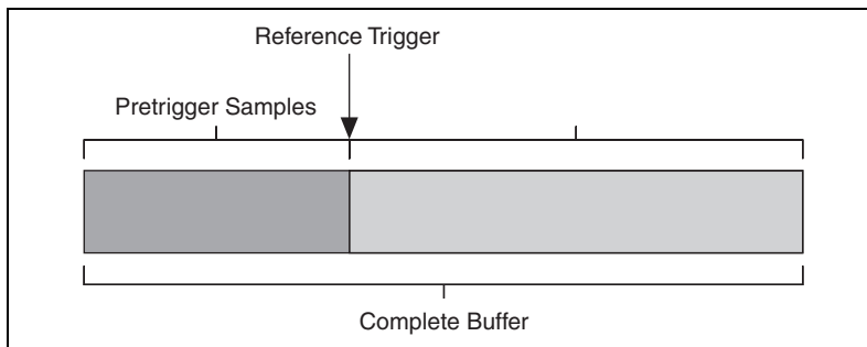
Figure 4-23. Reference Trigger Final Buffer
