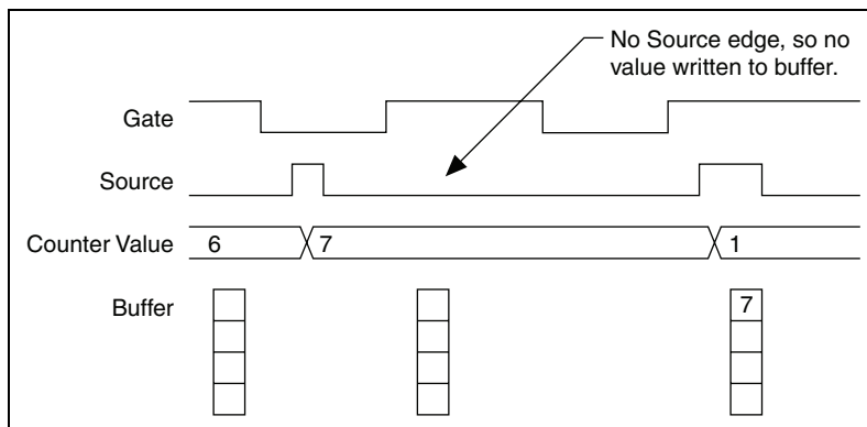
Figure 7-33. Duplicate Count Example
