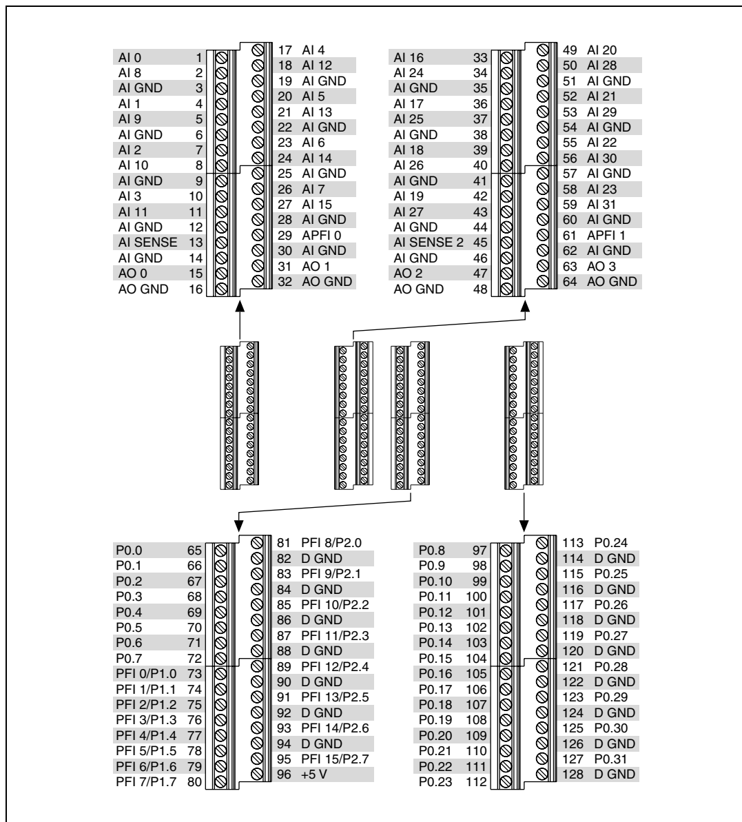
Figure A-45. USB-6259 Screw Terminal Pinout
