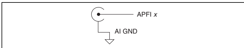
Figure A-52. Analog Programmable Function Interface Circuitry
