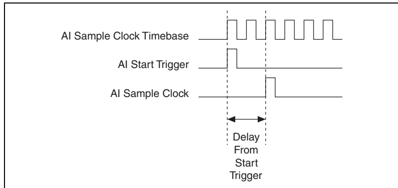
Figure 4-16. AI Sample Clock and AI Start Trigger
