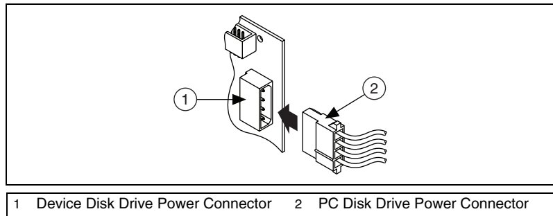
Figure 3-4. Connecting to the Disk Drive Power Connector
