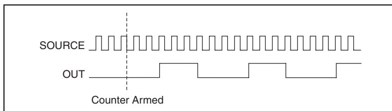
Figure 7-25. Continuous Pulse Train Generation
