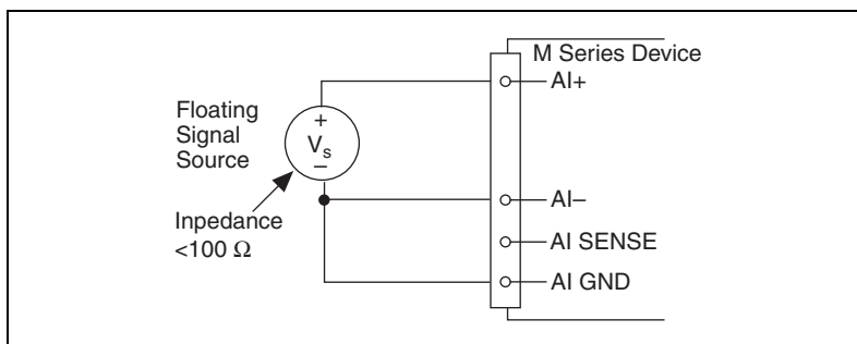
Figure 4-4. Differential Connections for Floating Signal Sources without Bias Resistors
