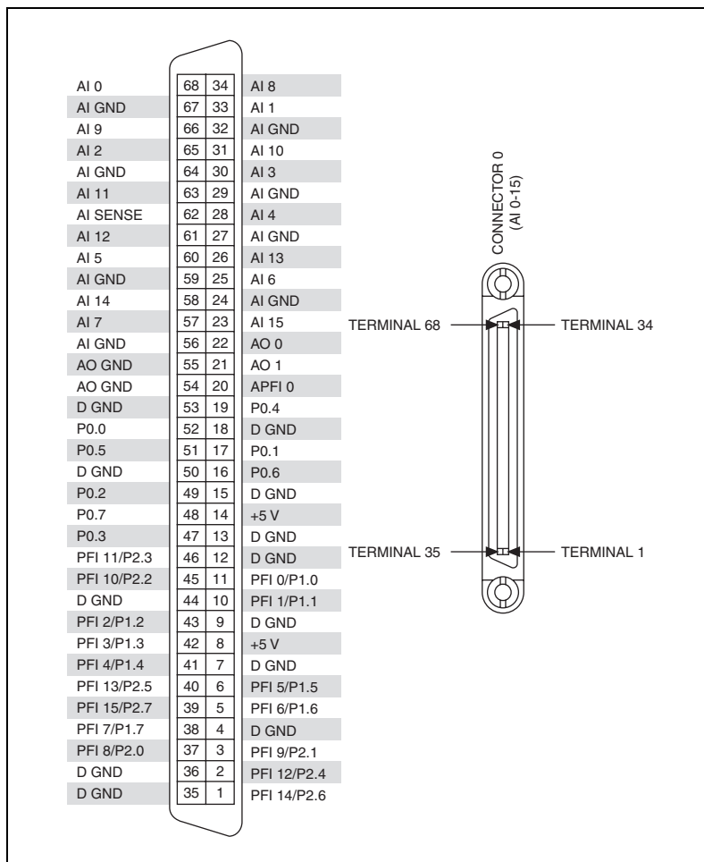
Figure A-28. NI PCI/PCIe/PXI/PXle-6251 Pinout
