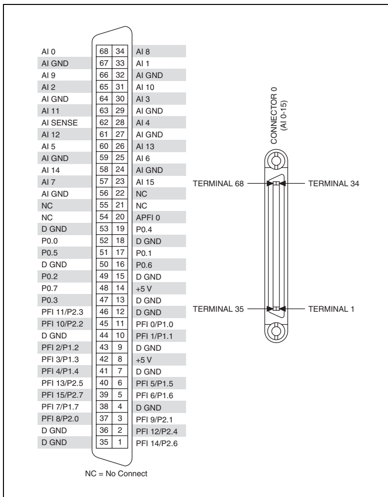
Figure A-27. PCI/PXI-6250 Pinout
