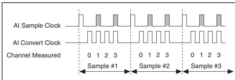
Figure 4-18. AI Sample Clock Pulses Are Gated Off; AI Sample Clock Too Fast For Convert Clock
