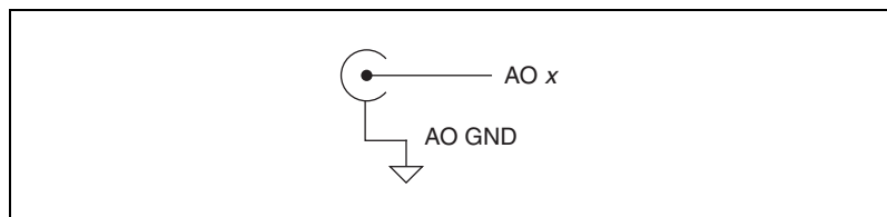
Figure A-9. Analog Output Circuitry
