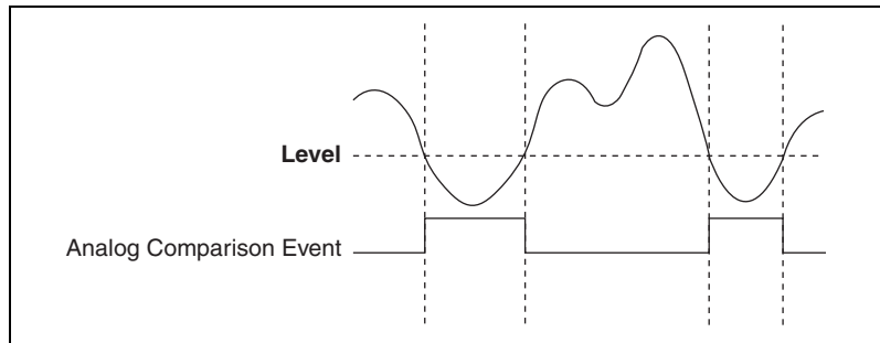
Figure 11-3. Below-Level Analog Triggering Mode
