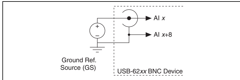
Figure A-8. Single-Ended Channels
