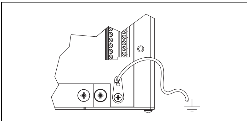
Figure 3-2. Grounding a USB-62xx Screw Terminal Device through the Chassis Ground Lug
