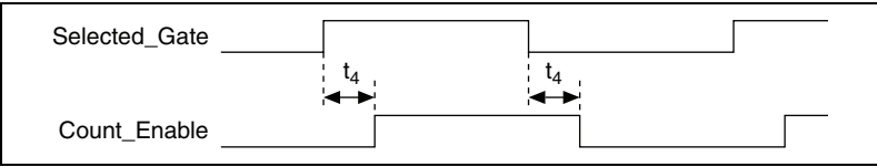
Figure B-45. Count Enable Delays
