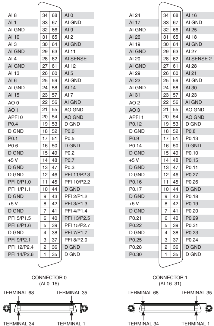
Figure A-63. USB-6289 Mass Termination Pinout
