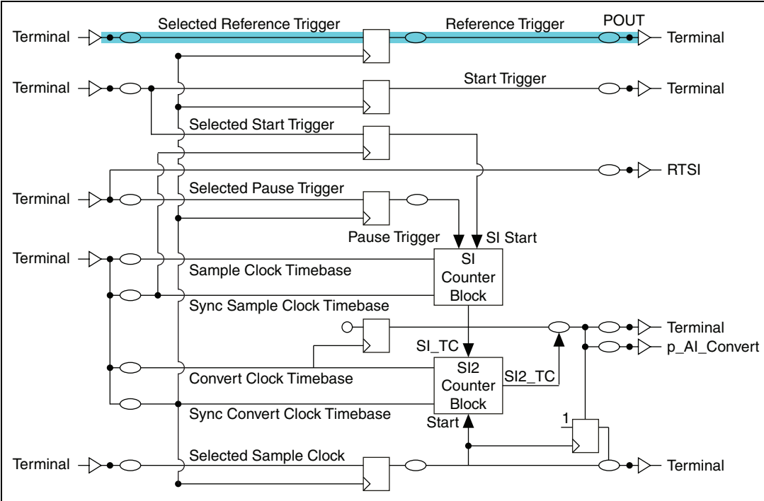
Figure B-13. Reference Trigger and the Analog Input Timing Engine
