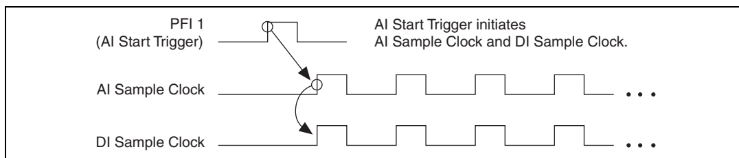
Figure 6-2. Digital Waveform Triggering
