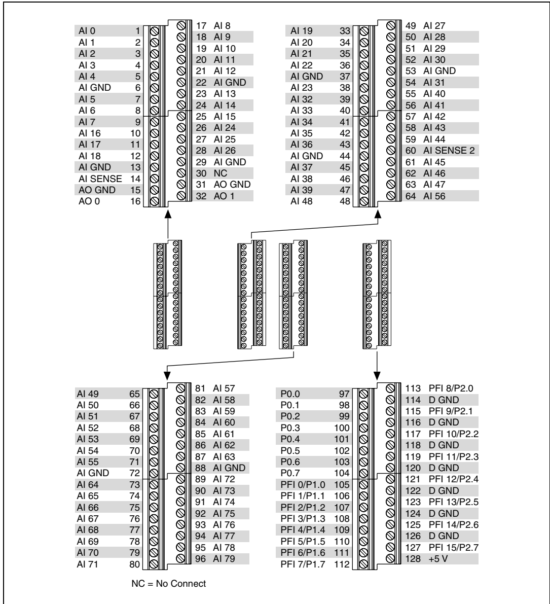
Figure A-15. USB-6225 Screw Terminal Pinout
