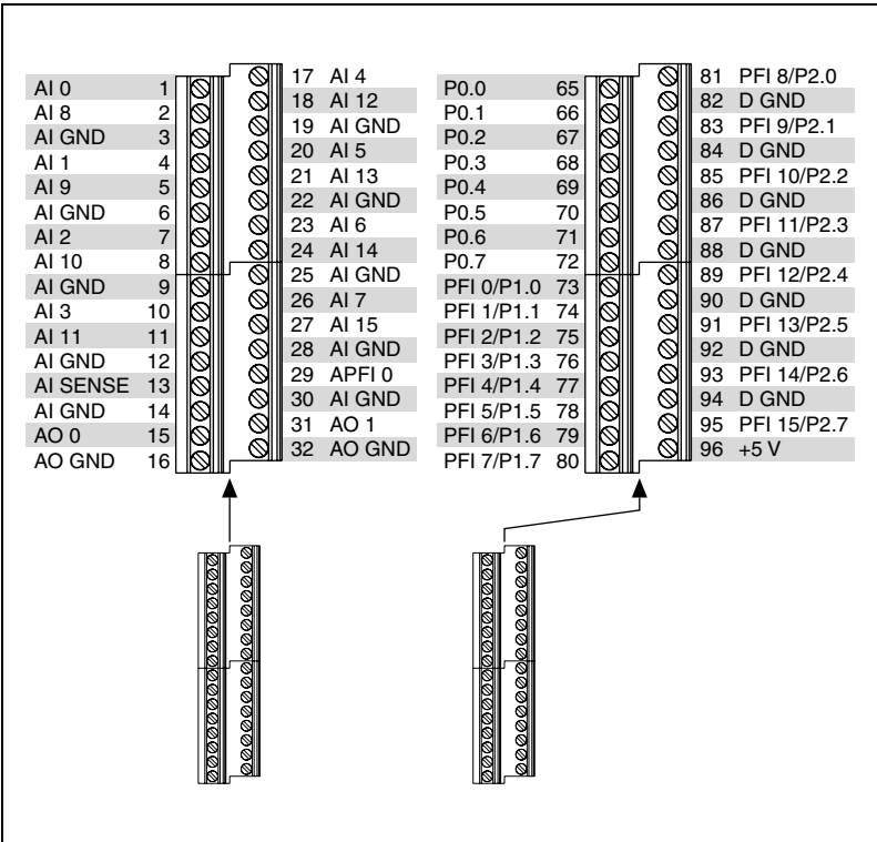
Figure A-29. USB-6251 Screw Terminal Pinout
