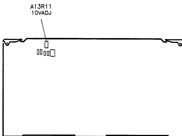
Figure 3-11. YO Driver +10V Reference Adjustment Location
