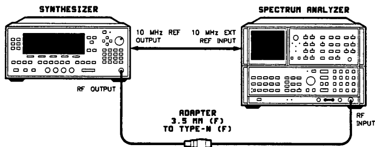
Figure 2-9. Spurious Signals (Harmonic) Test Setup
