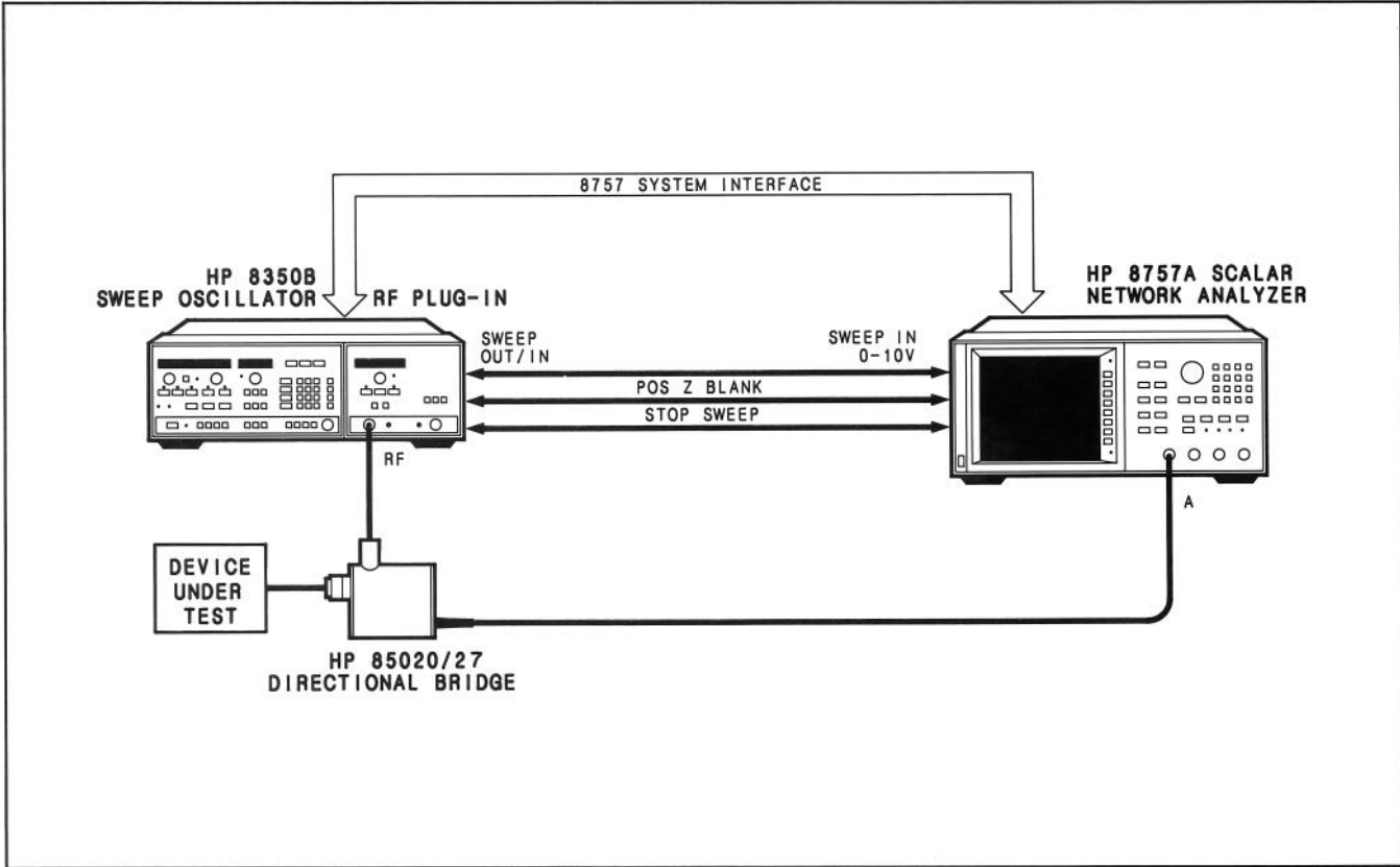
Figure 26. Measurement Setup for Reflection Measurements in AC or DC Mode
