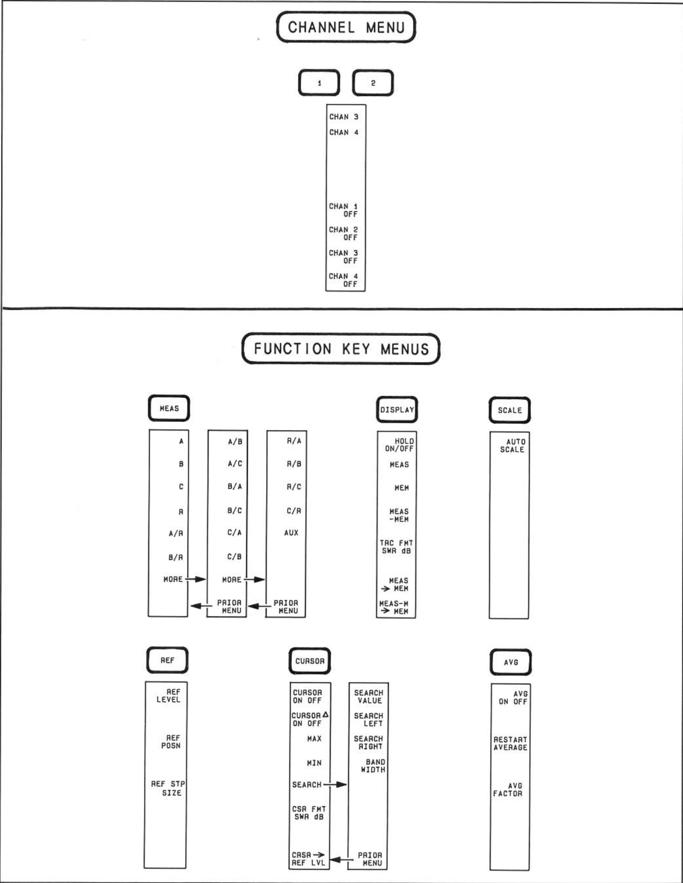
Figure 33. HP 8757A Menu Structure (1 of 3)
