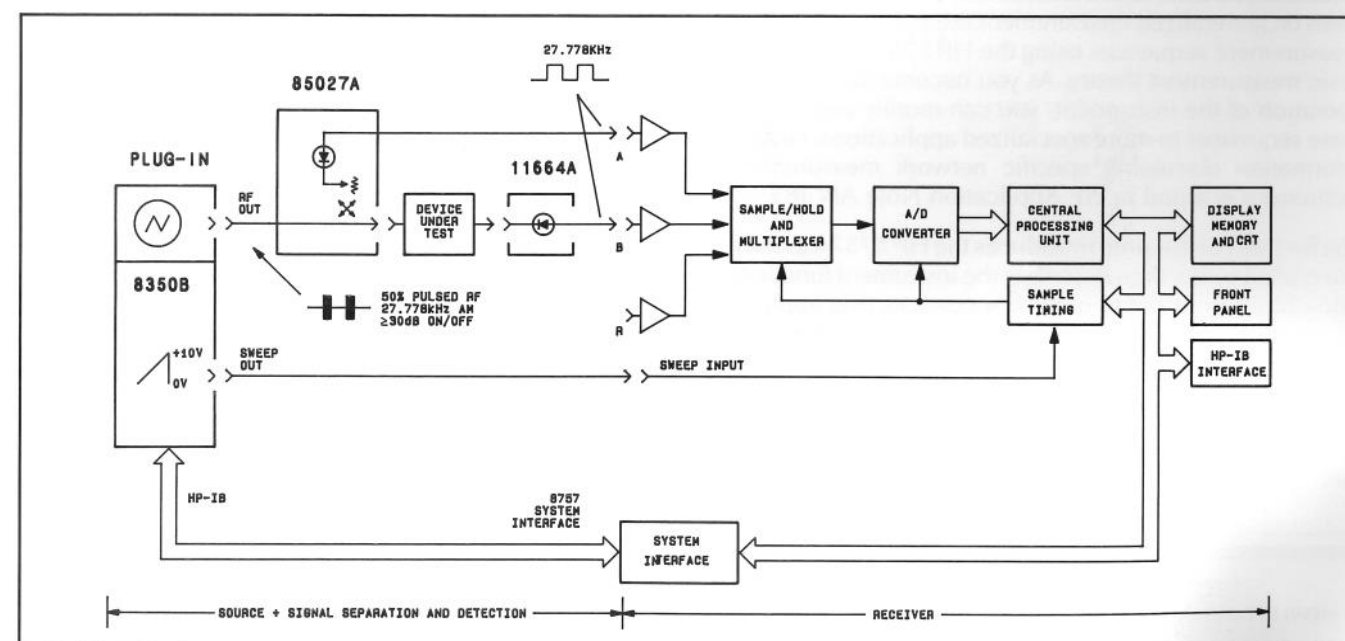
Figure 2. Source, Detectors, and Receiver Block Diagram
