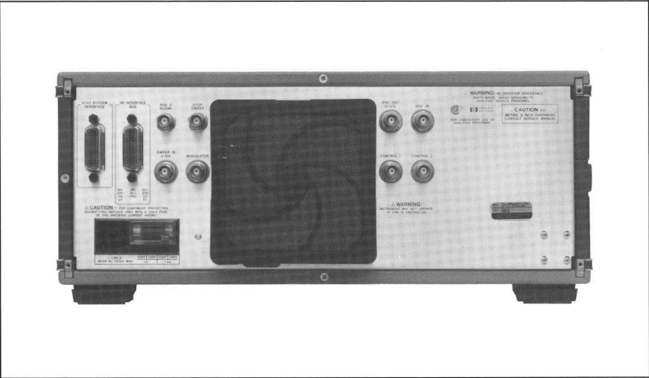
Figure 32. HP 8757A Rear Panel Connections
