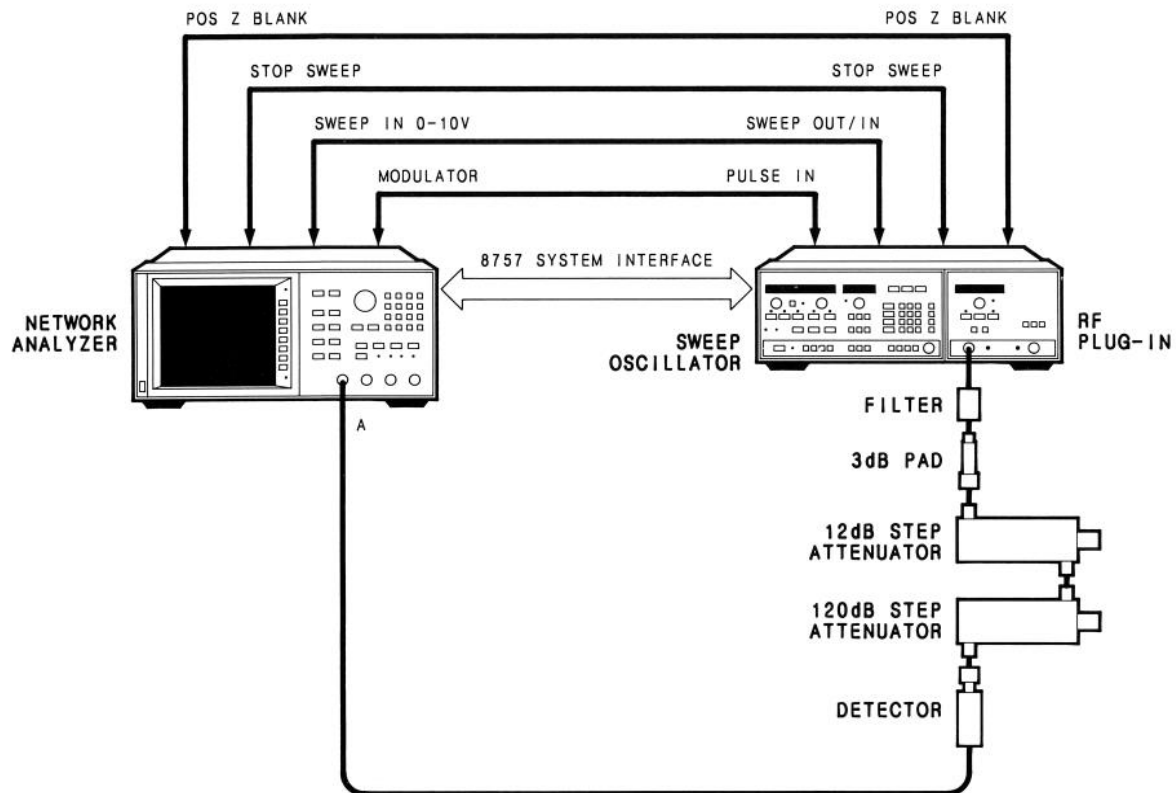
Figure 4-3. Dynamic Power Accuracy Test Setup
