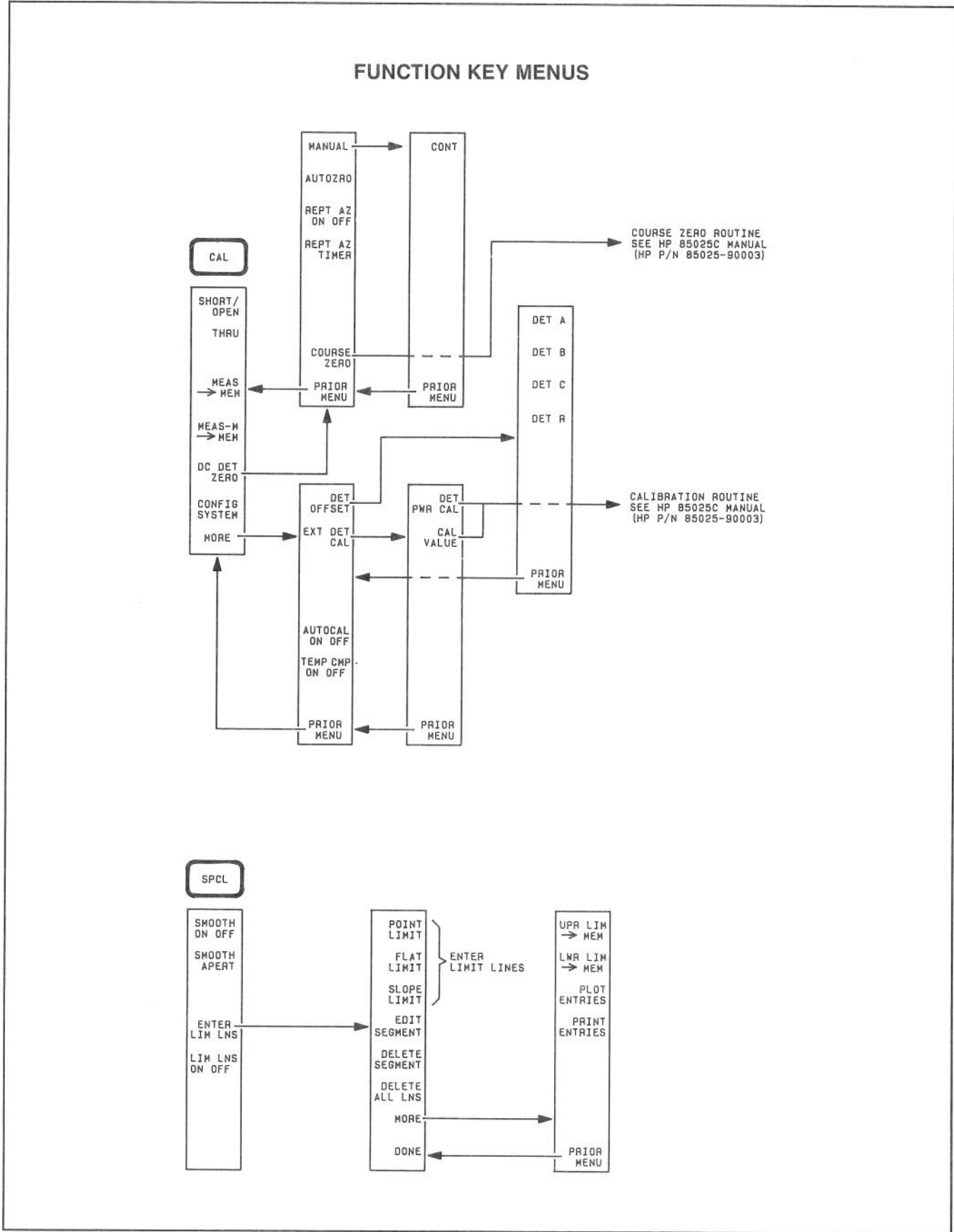
Figure 3-30. HP 8757A Menu Structure (2 of 3)
