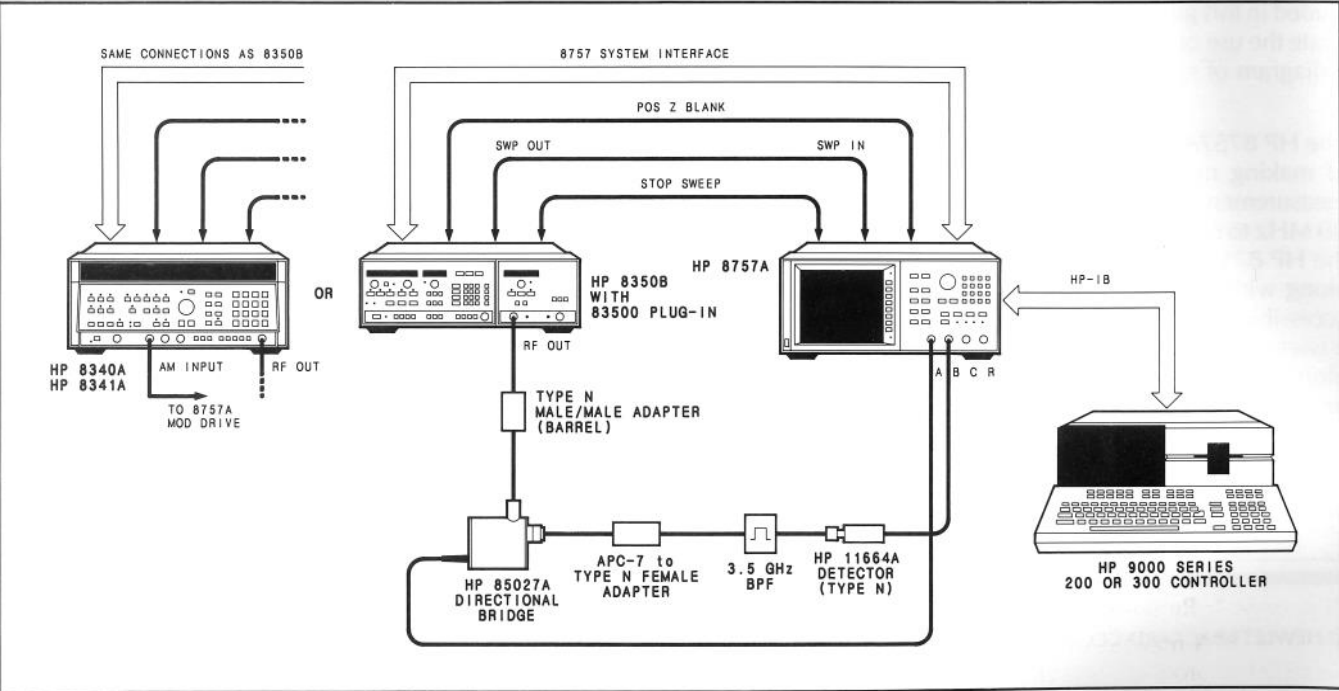
Figure 1. System Connections
