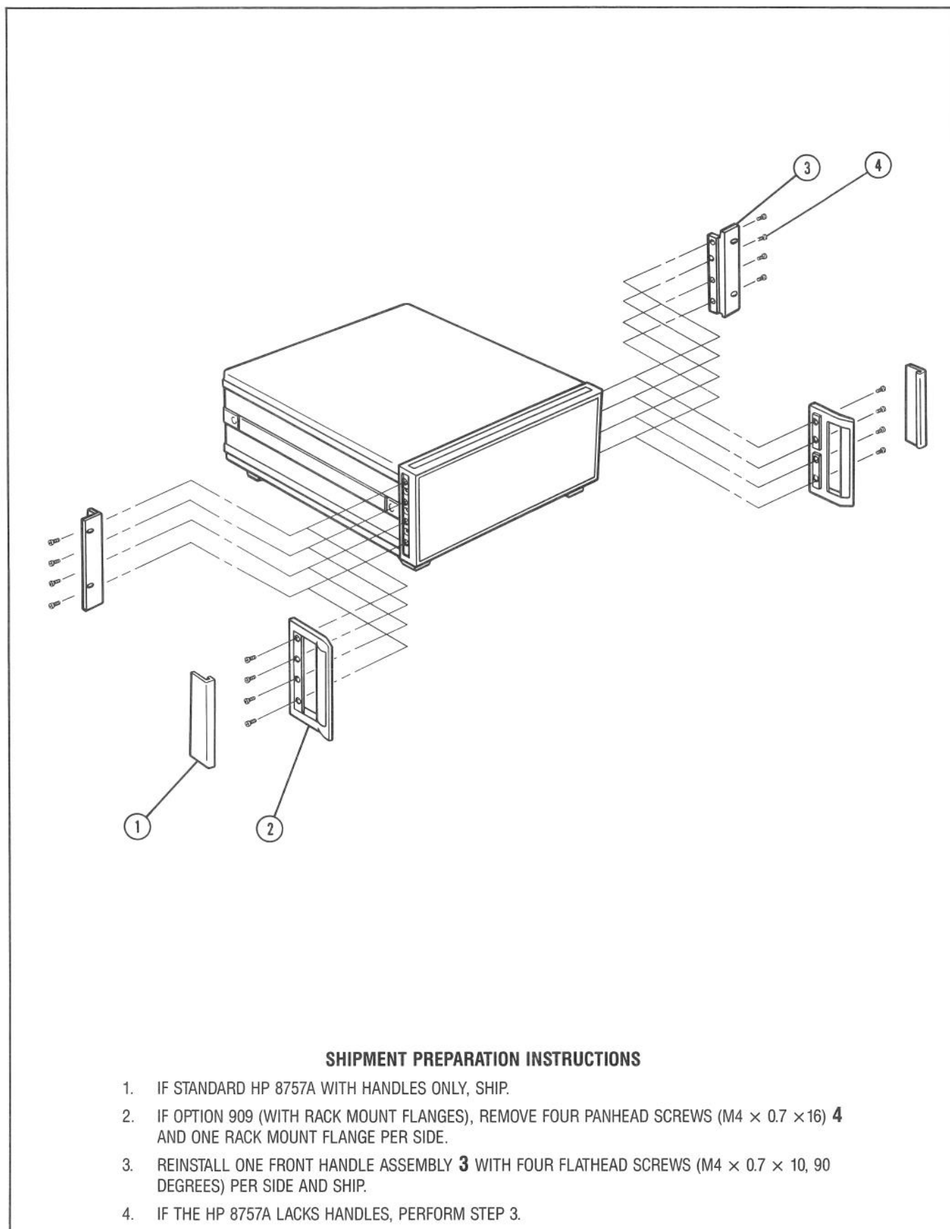
Figure 2-7. Preparation of Instrument for Shipment
