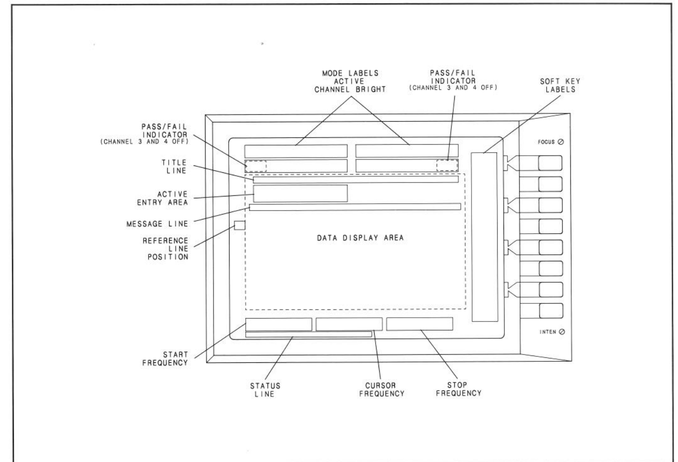
Figure 7. HP 8757A CRT Display
