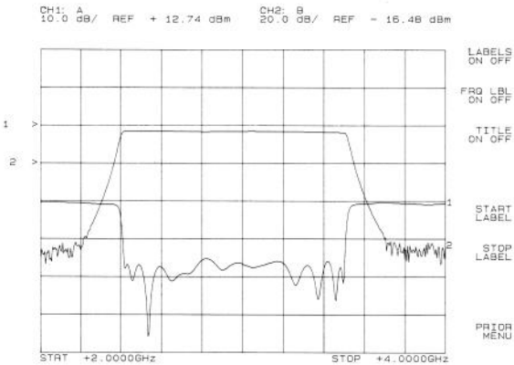
Figure 3-25. The Labels Menu
