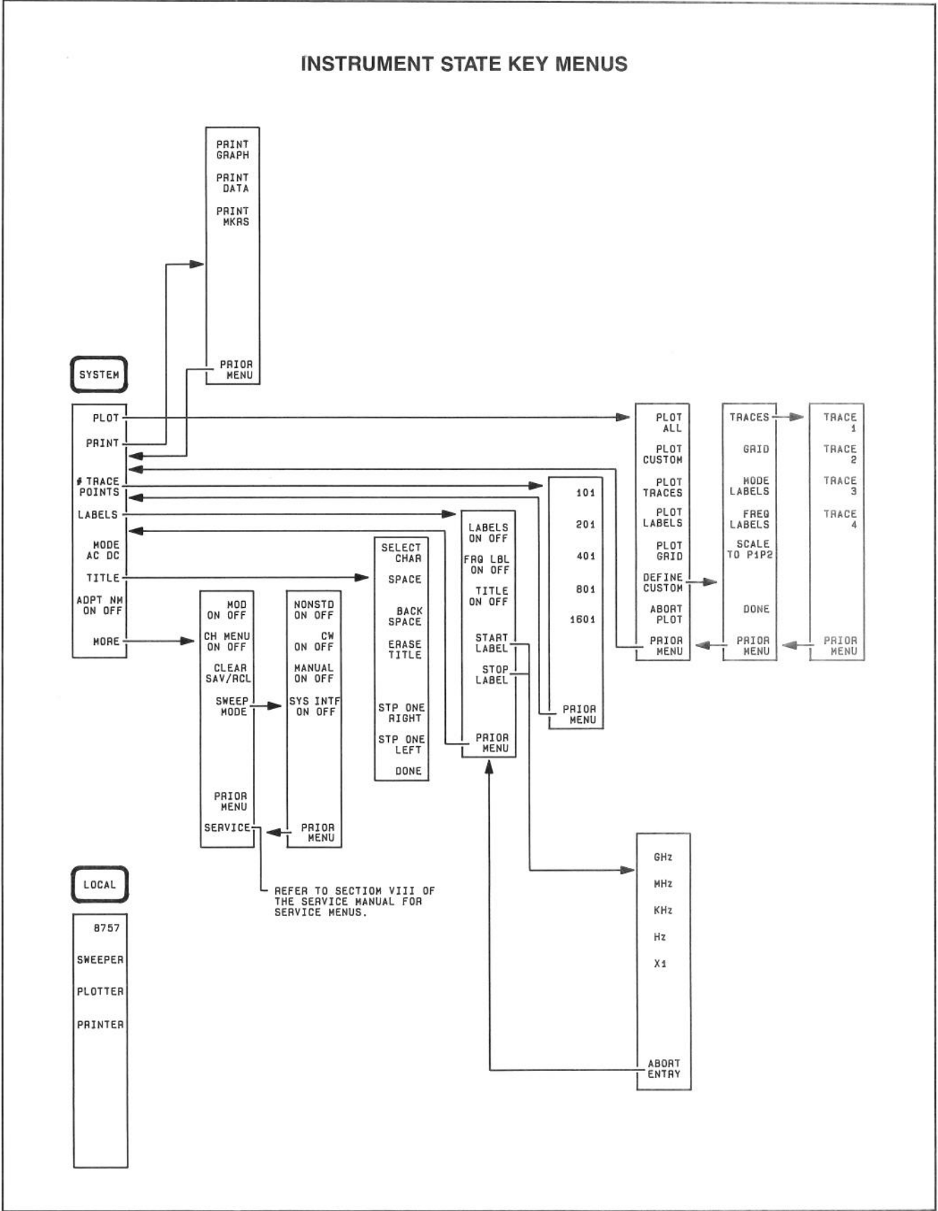
Figure 3-30. HP 8757A Menu Structure (3 of 3)
