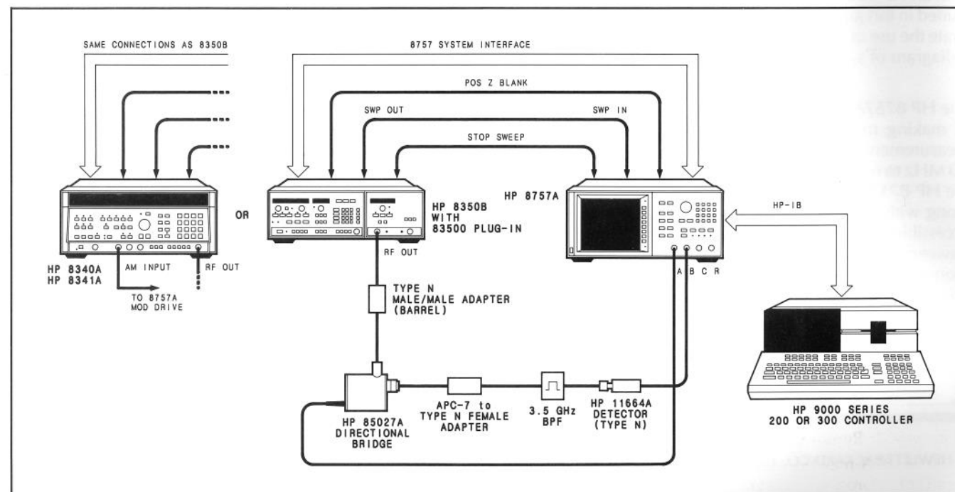
Figure 1. System Connections
