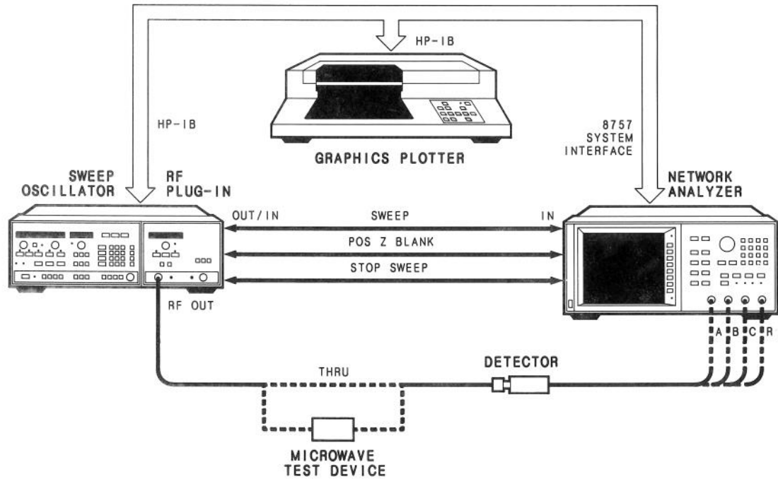
Figure 3-32. Equipment Setup for Operator's Check
