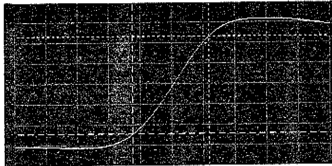
Figure 6-19. Risetime 10-90%
