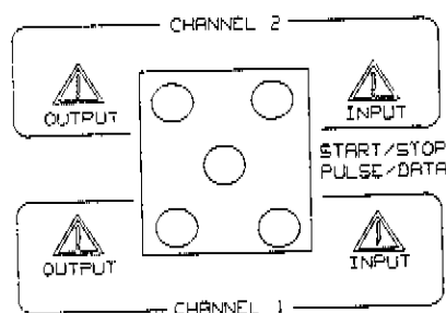
Figure 3-12. Rearpanel signal-connectors
