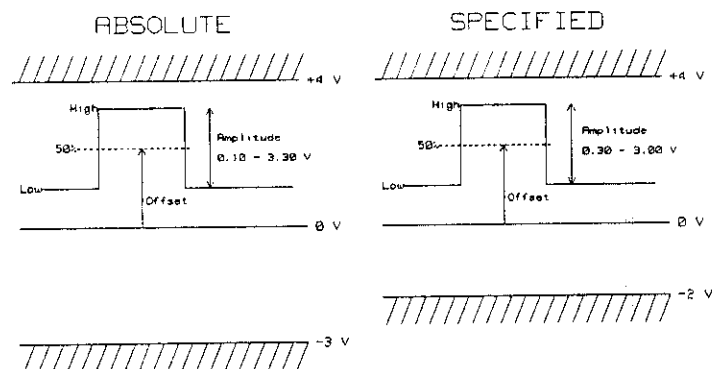
Figure 3-9. PULSE/DATA Output-level limits into 50 \Omega
