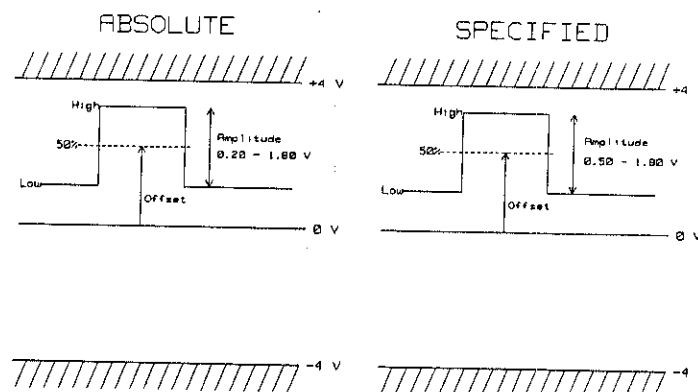
Figure 3-5. TRIGGER Output-level limits into 50Ω
