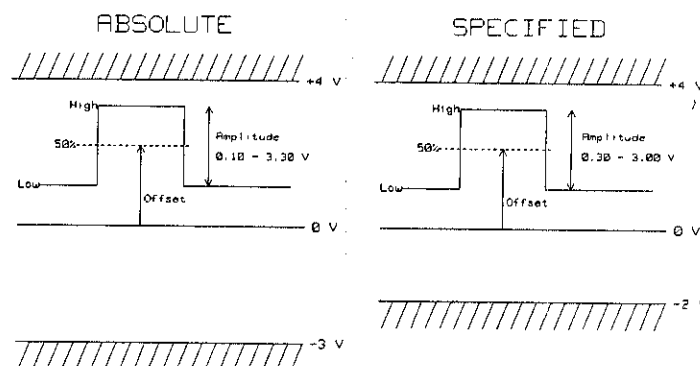
Figure 3-7. PULSE Output-level limits into 50 \Omega
