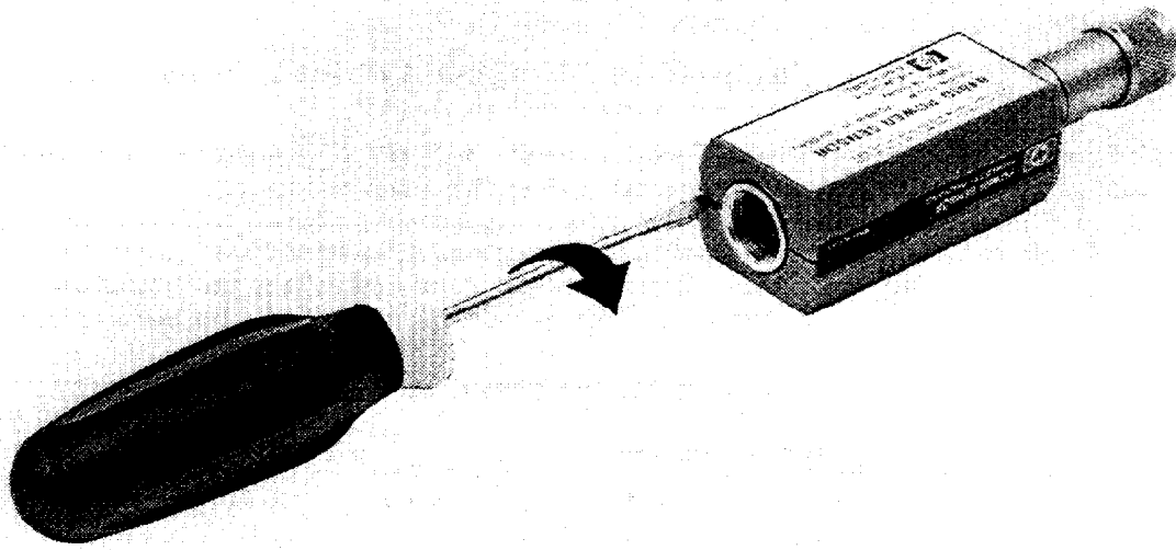
Figure 4 Removing Power Sensor Shell
