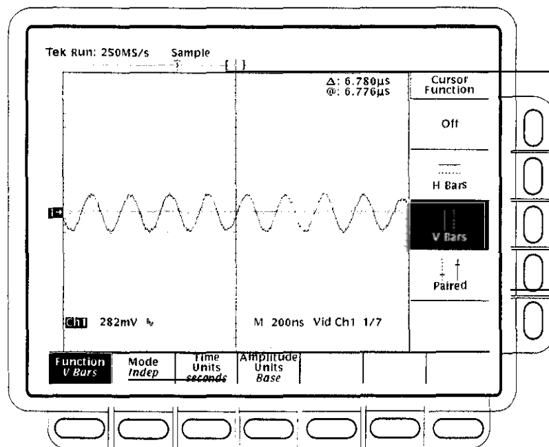
Figure 1-36: Line Count Accuracy Correct Result Waveform
