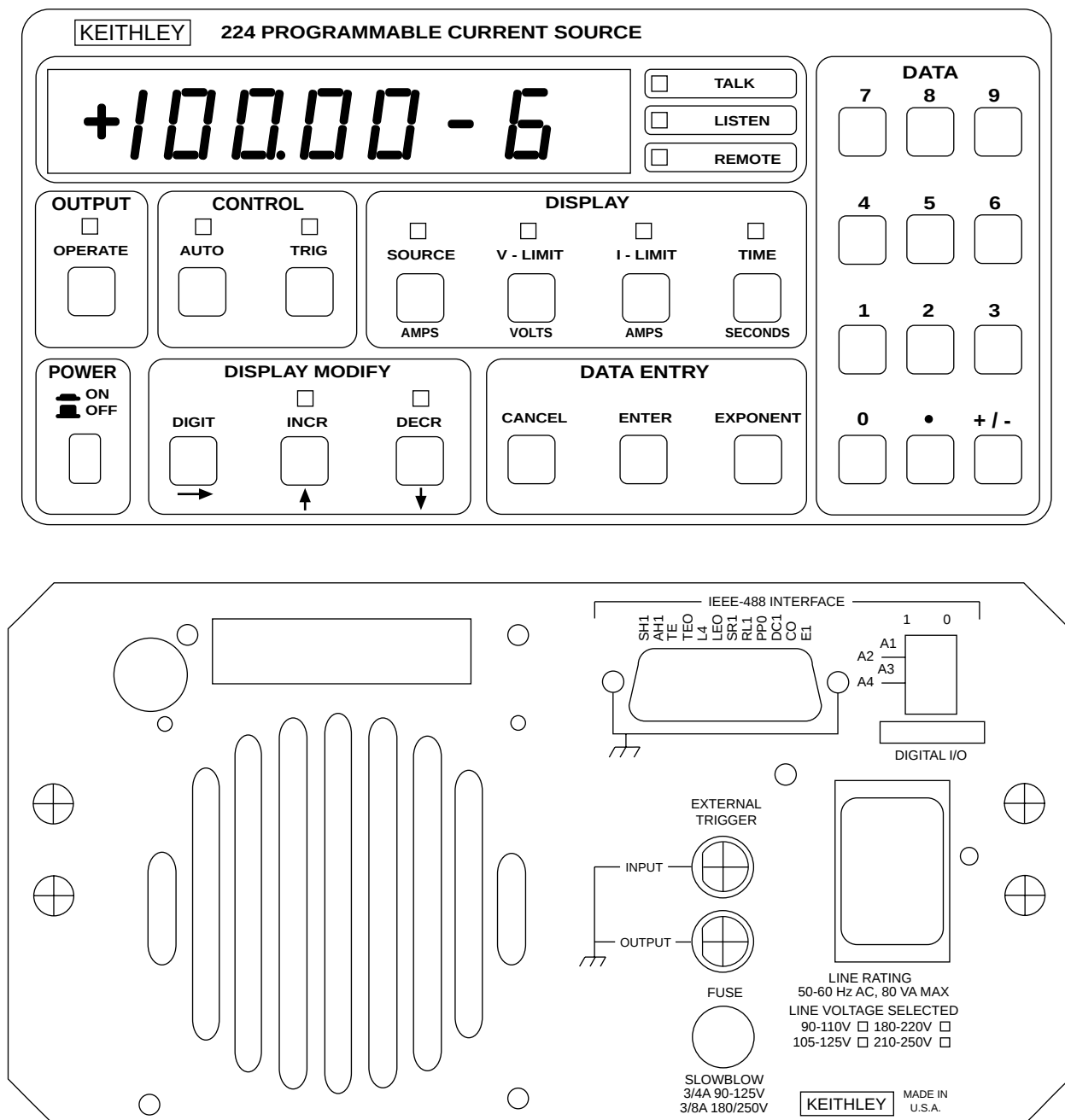
Figure 2-1. Model 224 Front and Rear Panels
