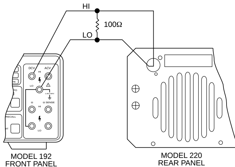
Figure 3-1. 100mA to 1mA Range Verification
