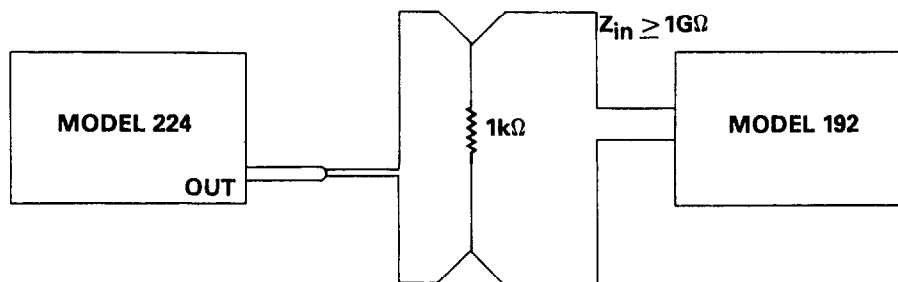
Figure 5-2. Calibration Configuration
