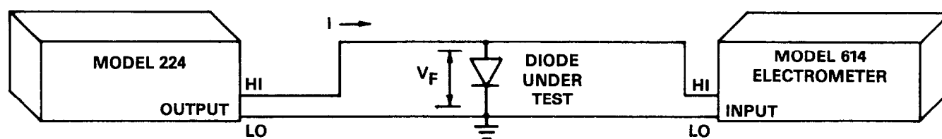
Figure 2-12. Diode Characterization
