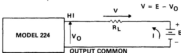
Figure 2-9. Connections as a Current Sink with a Resistive Load
